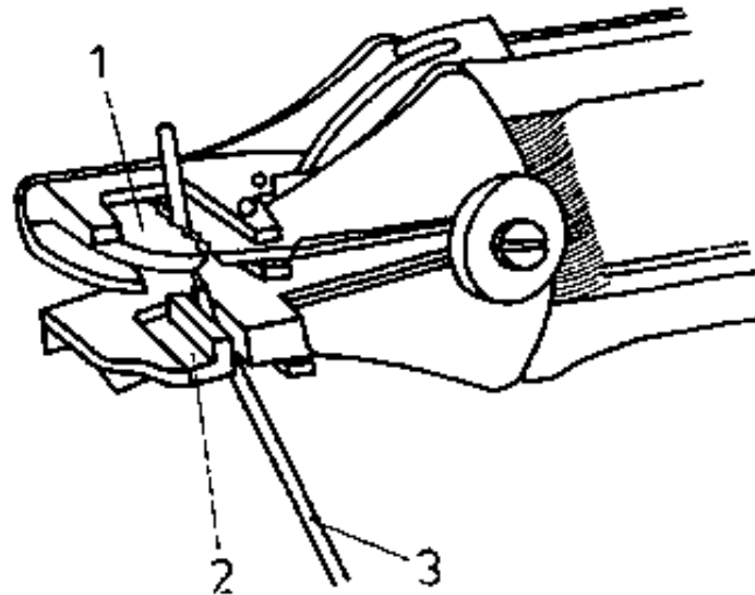
Figure 9 Wire strippers
