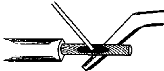
Figure 10 Tinning of a conductor
