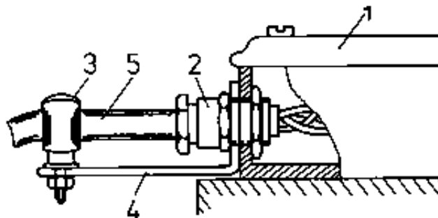
Figure 28 Tension relieving at an engine cable
