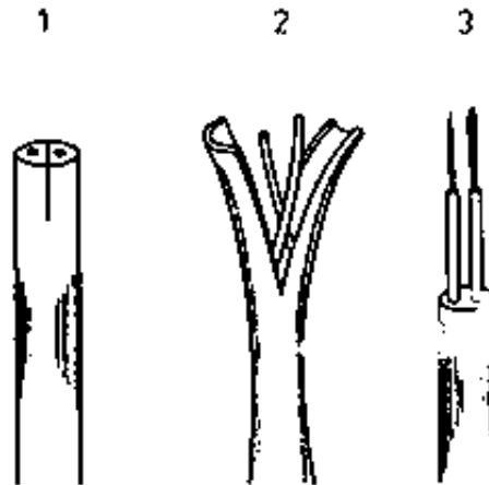
Figure 6 Stripping of a light rubber hose cable
