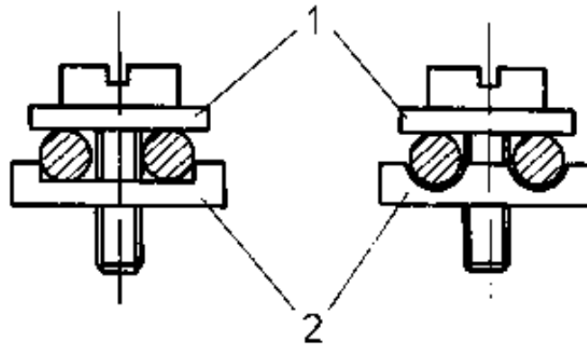
Figure 26 Connection to cap-screw with holding fixture
