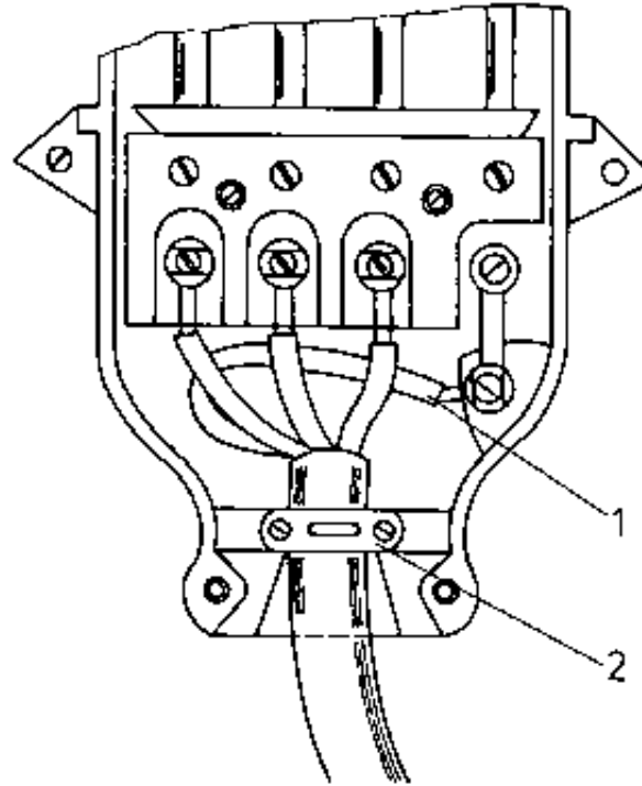
Figure 21 Collar coupler plug
