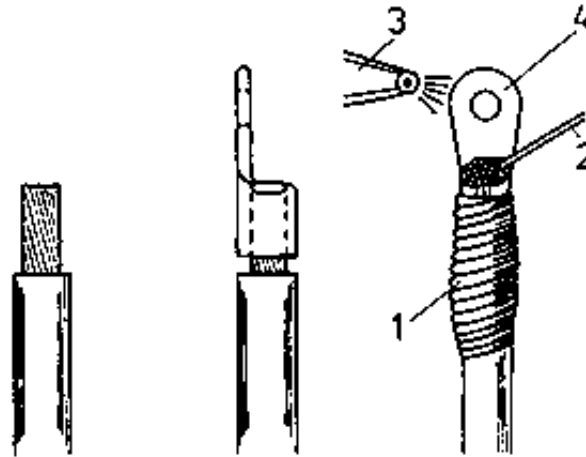
Figure 11 Soldering of a cable eye
