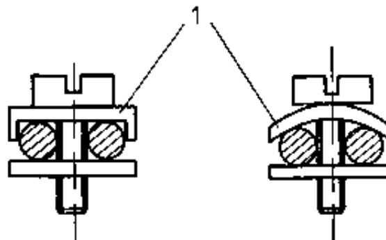
Figure 25 Connection to a cap-screw with clamping bow
