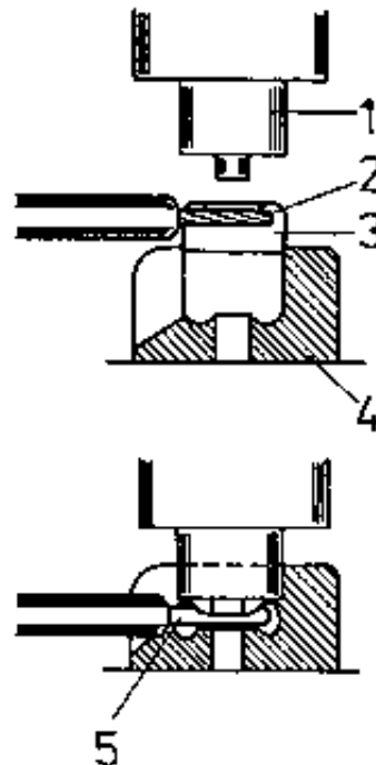
Figure 19 Principle of the pressing-on of contact eyes
