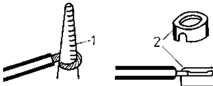
Figure 18 Prebending of the conductor over an arbor
