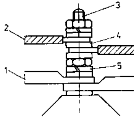
Figure 23 Connection to a connection bolt
