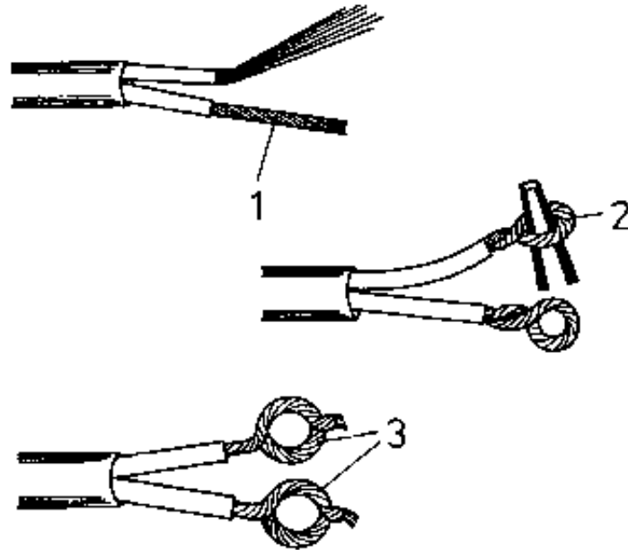
Figure 17 Bending of eyes
