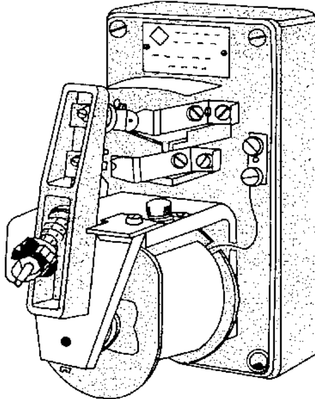
Figure 30 Undervoltage relay
