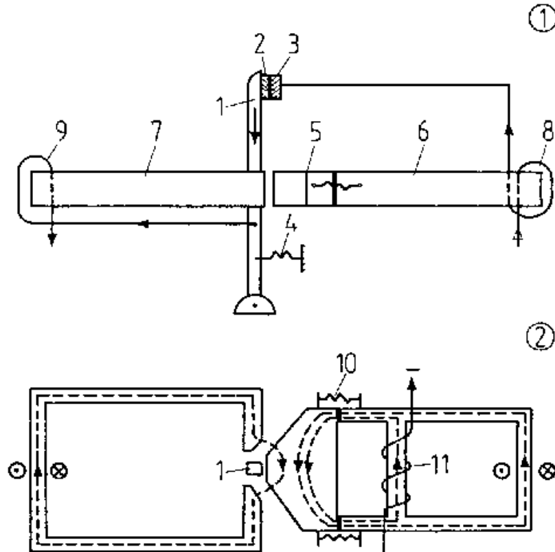
Figure 5. Principle of the highspeed switch with impact armature (1) Side view (2) Top view - 1 switch lever, 2 movable contact, 3 fixed contact, 4 contact pressure spring, 5 impact armature, 6 holding
