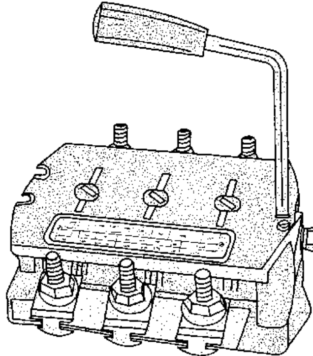
Figure 20. FTLA load-break switch 250 A in open design
