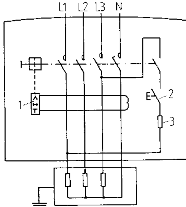
Figure 10. Principle of the fault-current protective switch
