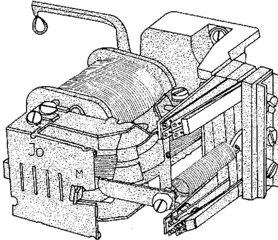
Figure 35 Signal relay RA70
