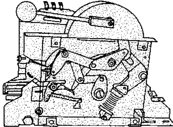
Figure 2. Latching mechanism of the universal circuit breaker of type EL
