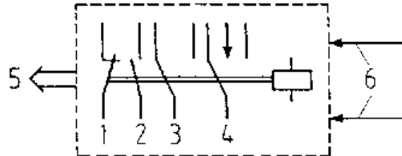
Figure 27. Types of contacts (types of switching elements) on a relay
