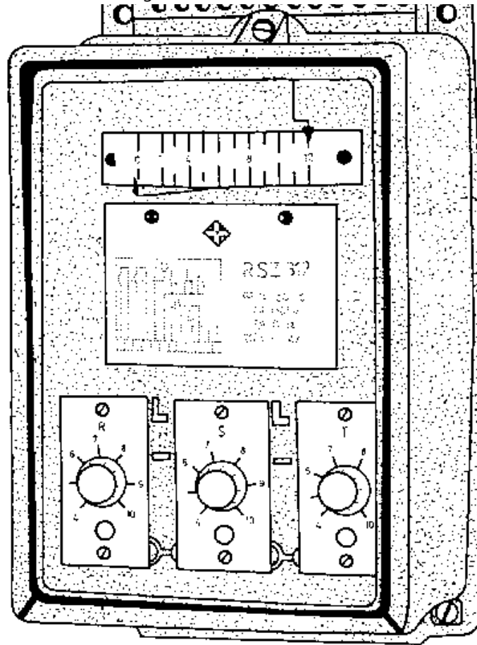
Figure 33. Overcurrent time relay RSZ3f2
