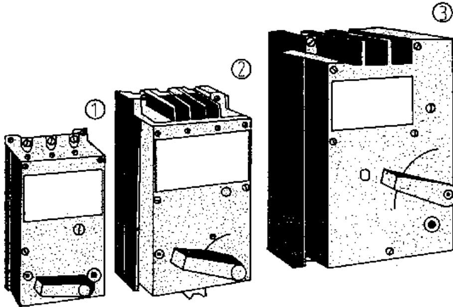
Figure 3. Compact circuit breaker of type EBL (1) 25 A, (2) 63 A, (3) 160 A
