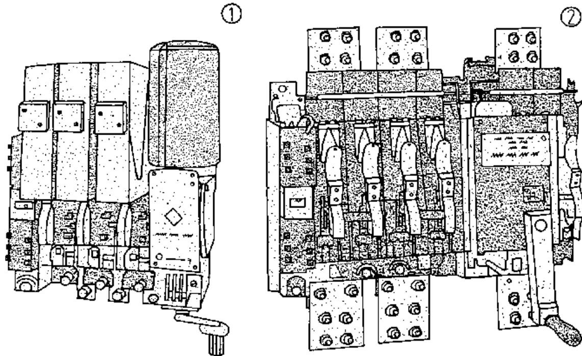
Figure 1. Universal circuit breaker of type EL (1) 630 A,(2) 1000 A with the arc-control chamber removed
