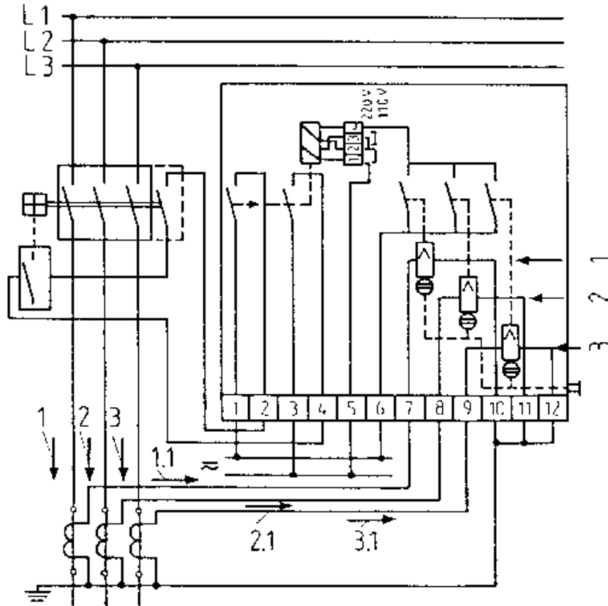
Figure 34 Circuit of the overcurrent time relay RSZ3f2
