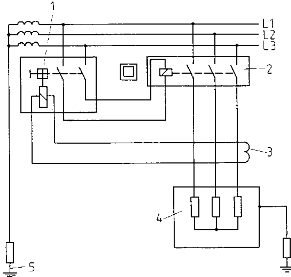
Figure 11 Fault-current control circuit
