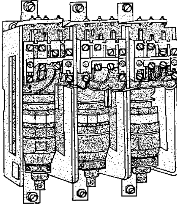
Figure 19. Vacuum contactor with three arc chambers
