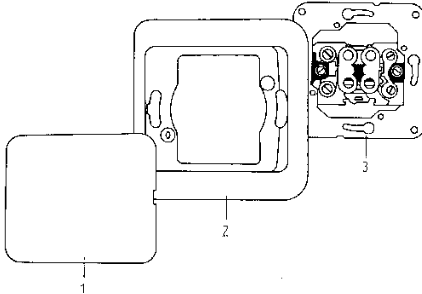
Figure 22. Installation switch, dismantled (flush design) - 1 junction rocker, 2 covering frame, 3 switch 10 A/220 V a.c.
