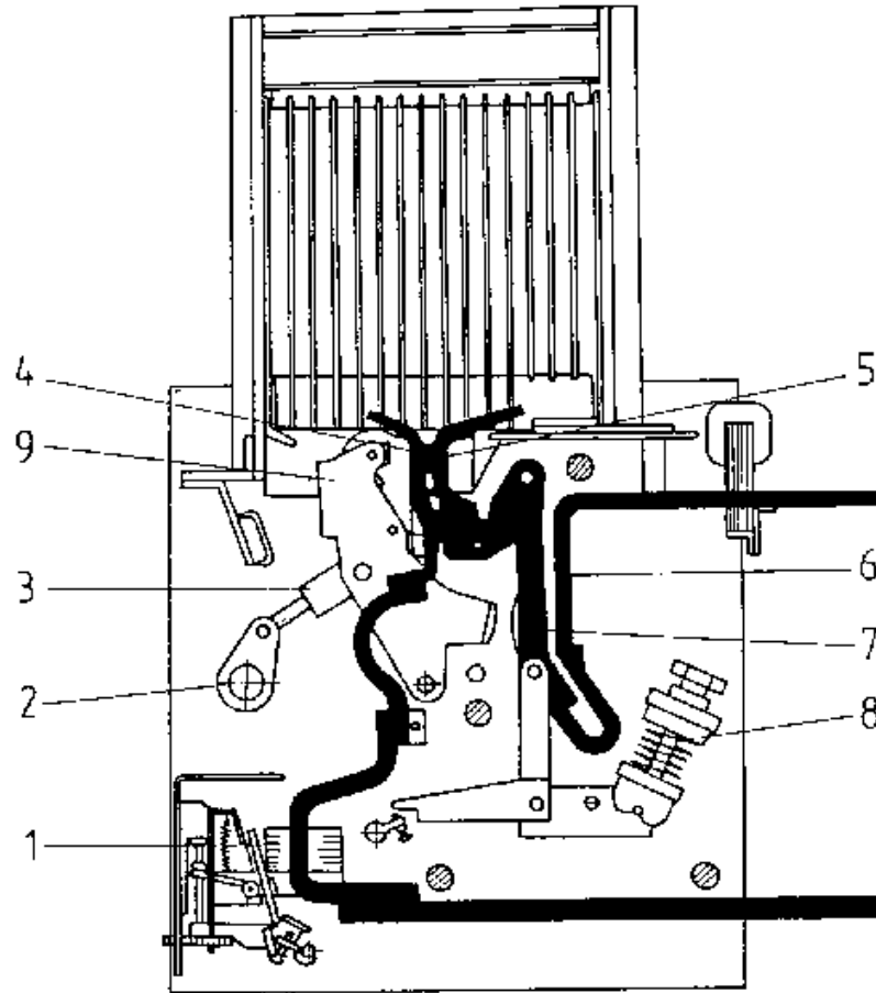
Figure 4. Sectional drawing of the compact circuit breaker of type EBL
