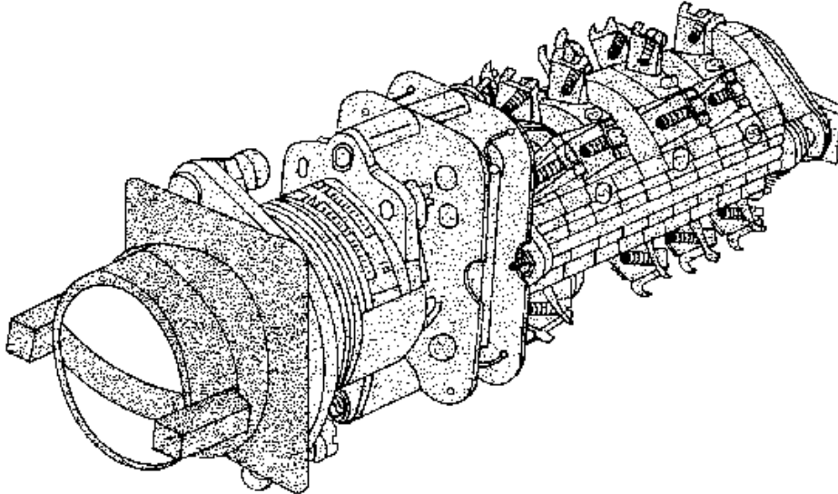
Figure 37 Discrepancy control switch SM2
