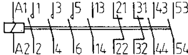
Figure 14. Circuit diagram of an LX1-32 air-break contactor
