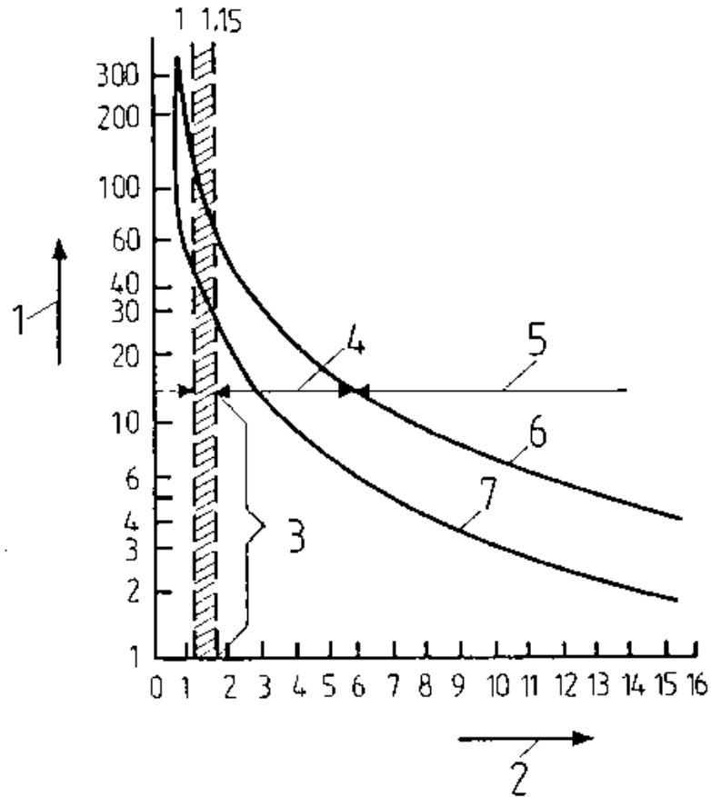
Figure 31. Release characteristic of a thermal overcurrent relay in the
