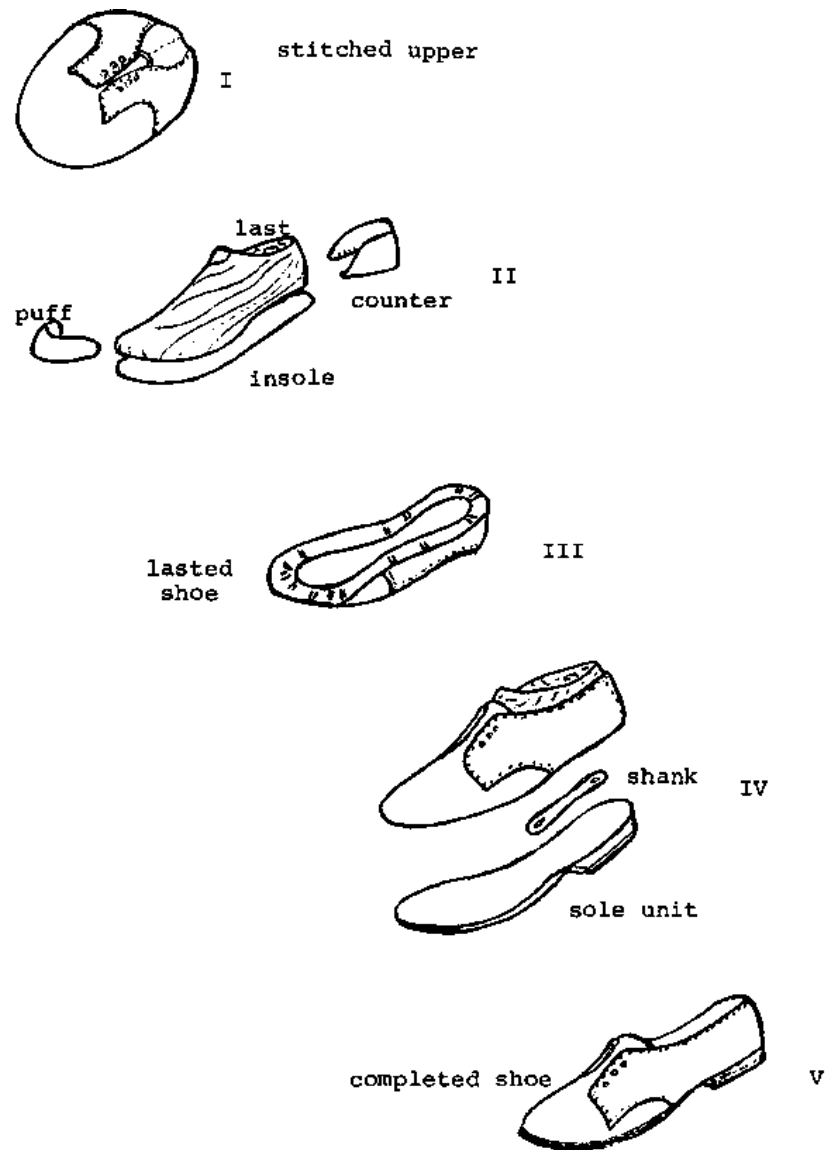
Figure II.1 Stages in the manufacture of Type 1 footwear
