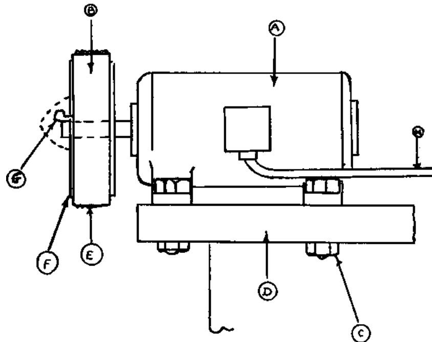
Figure II.11 A simply made scrouer for small volume production.
