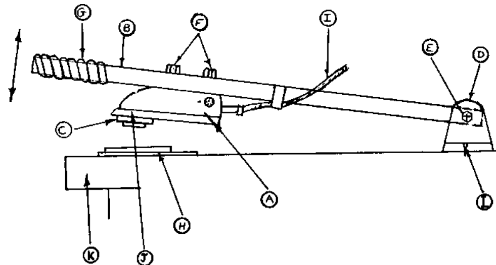
Figure II.4 A simply made insole embosser for small volume production
