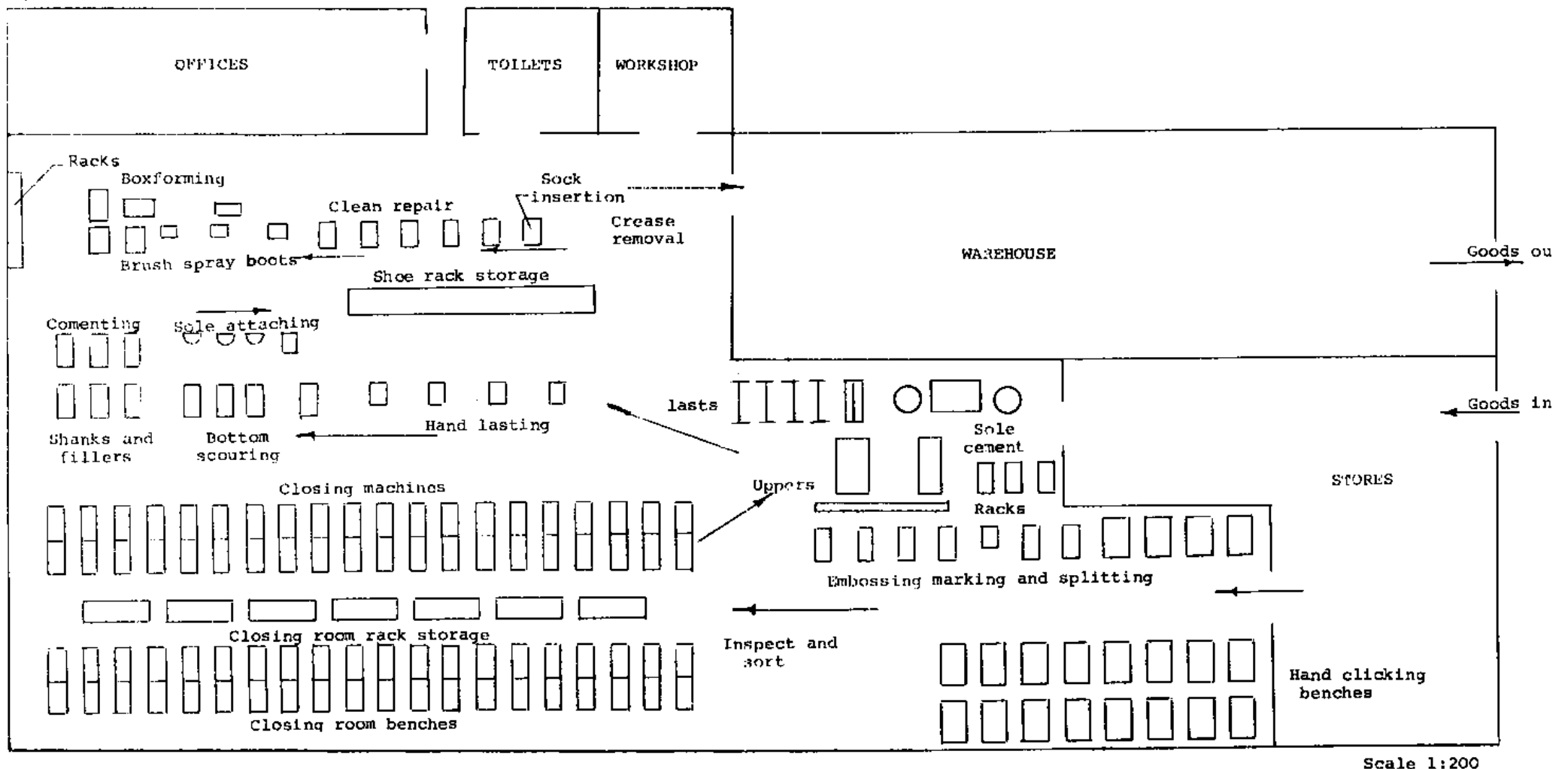
Figure II.15 Plant layout for type 1 foot-year - 1000 pairs per day
