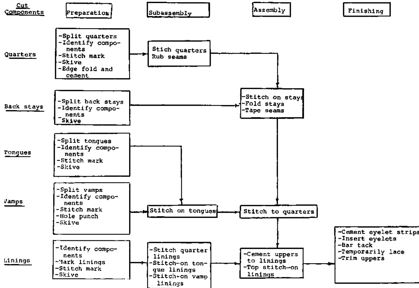
Figure II.3 Typical work flow during preparation and stitching
