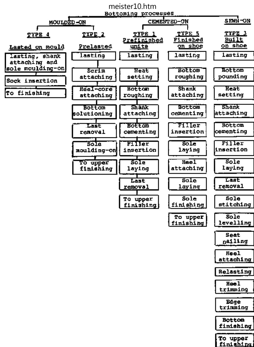
Figure III.1 Comparison of alternative bottoming processes
