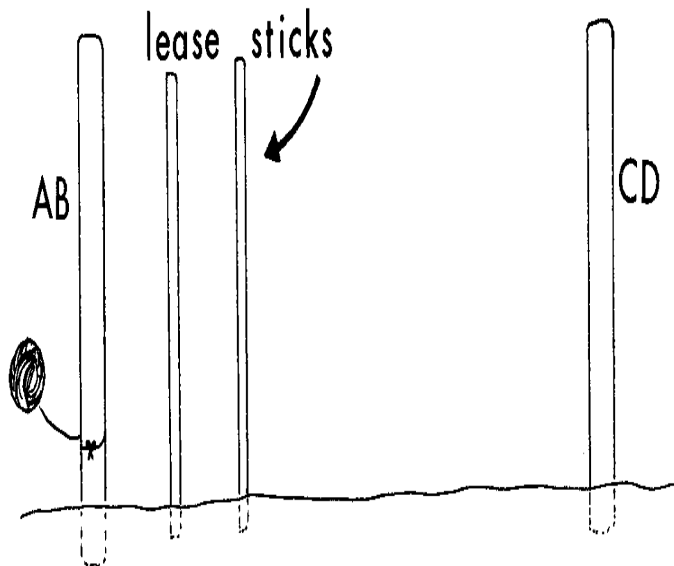
Side View - Warping the Peg Loom
