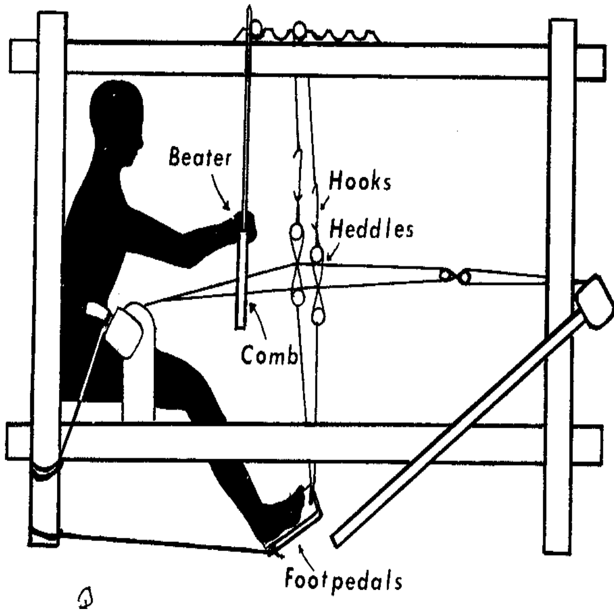
MACHINERY IN PLACE ON CEILING-SUPPORTED LOOM
