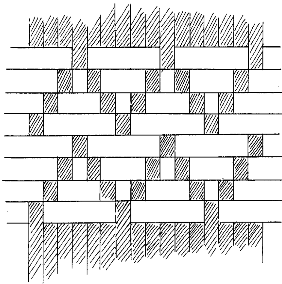
HERRINGBONE TWILL
