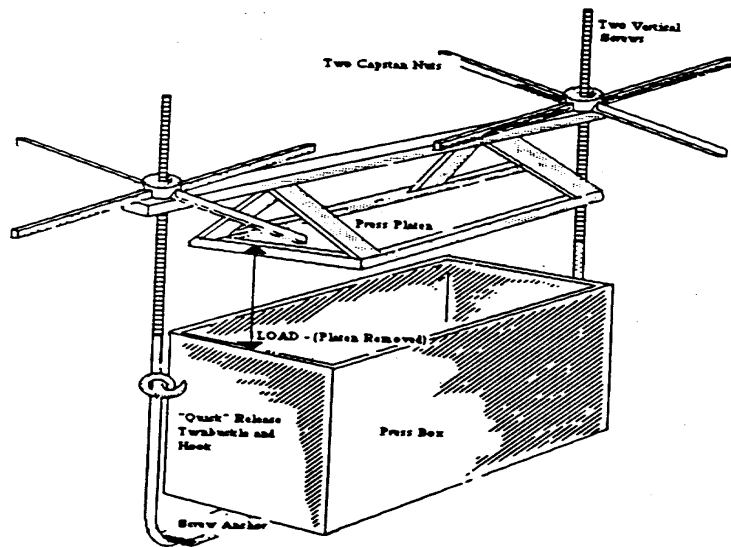
Figure 1. HAND-POWERED MECHANICAL PRESSES
