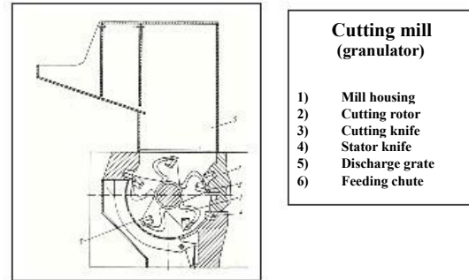
Fig. 2: Grinder/granulator for hard plastic
