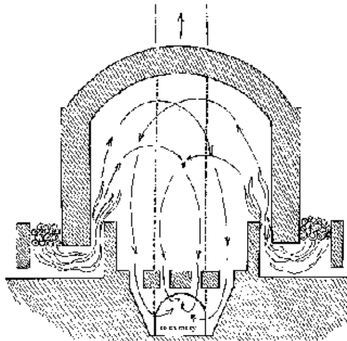
Fig.2-16: Down-draught kiln with flue channels under the floor
