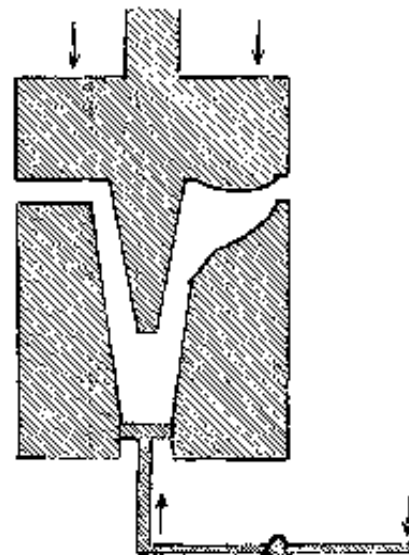
Fig. 1-29: Thimble press mould with ejector
