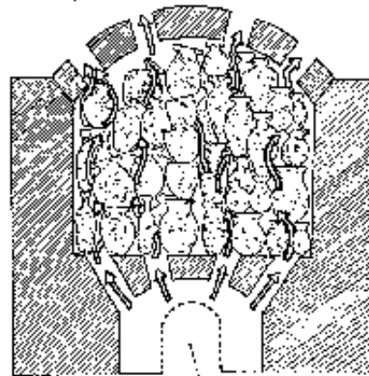
Fig.2-11: Setting of pots in an up-draught kiln has to be done so that the hot gases rise evenly through the pots.
