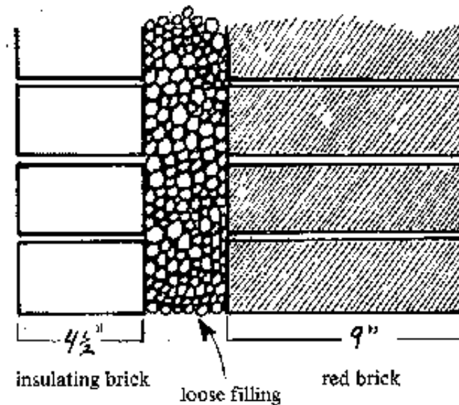
Fig.2-87: Cross-cut of a circular kiln wall.
