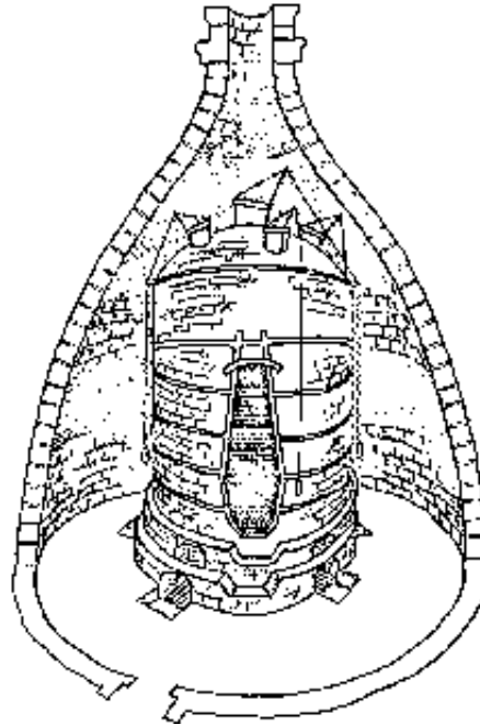
Fig.2-13: Cross-section of a hovel kiln
