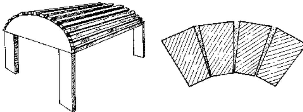
Fig.2-93: Arch support frame Fig.2-94: Bottom of the joints should be as thin as possible.
