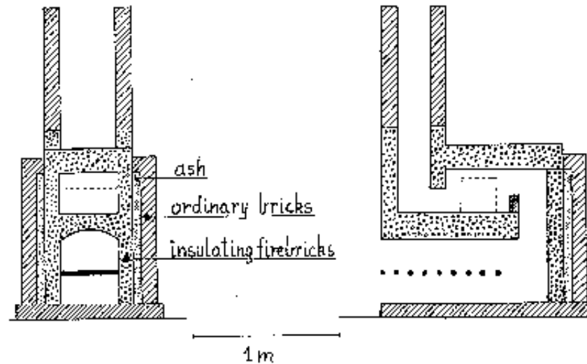
Fig. 1-48: Test kiln
