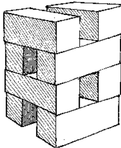
Fig. 1-37: Open stacking of firebricks for even drying
