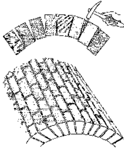
Fig.2-96: Square brick arch. Fig.2-97: Bonded arch
