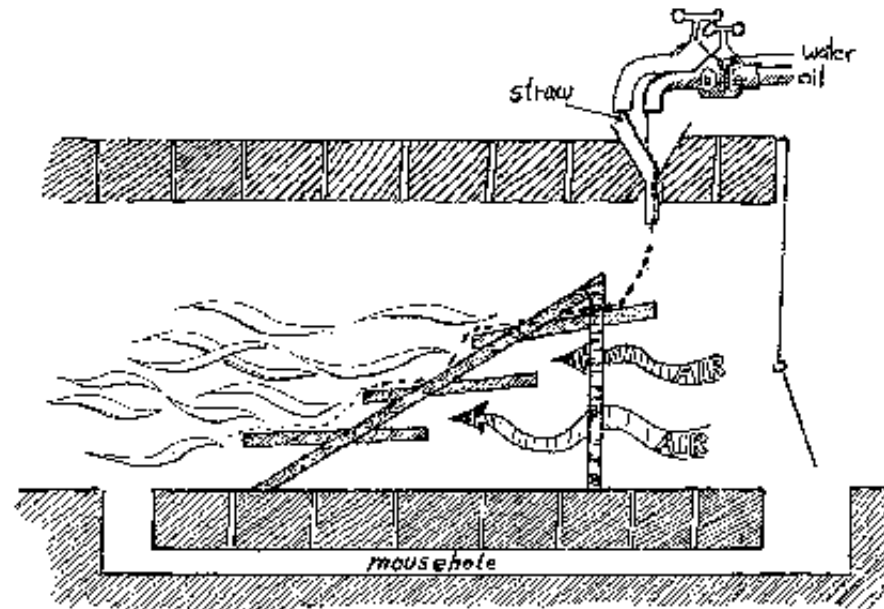
Fig.2-66: Drip-plate burner.
