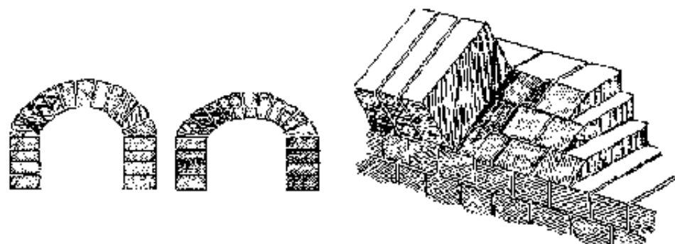
Fig.2-90: Firebox arch after construction, and later after firing shrinkage of the firebricks has taken place. The initial high rise saved the firebox arch from collapsing due to firing shrinkage; Fig.2-91: Skewbacks cut from square bricks
