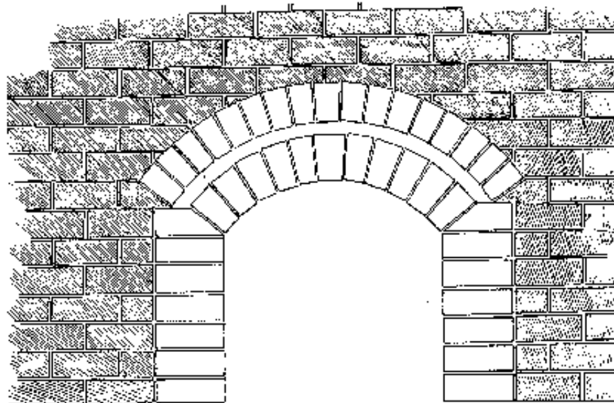
Fig.2-92: Relieving arch.
