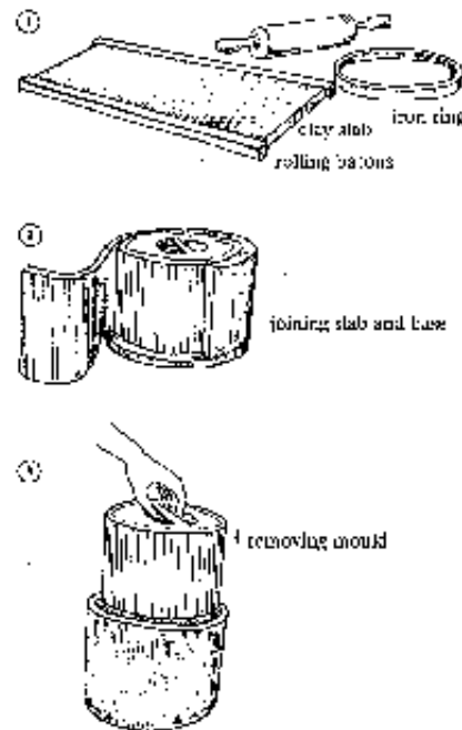
Fig.1-20 Hand- moulding of a saggar
