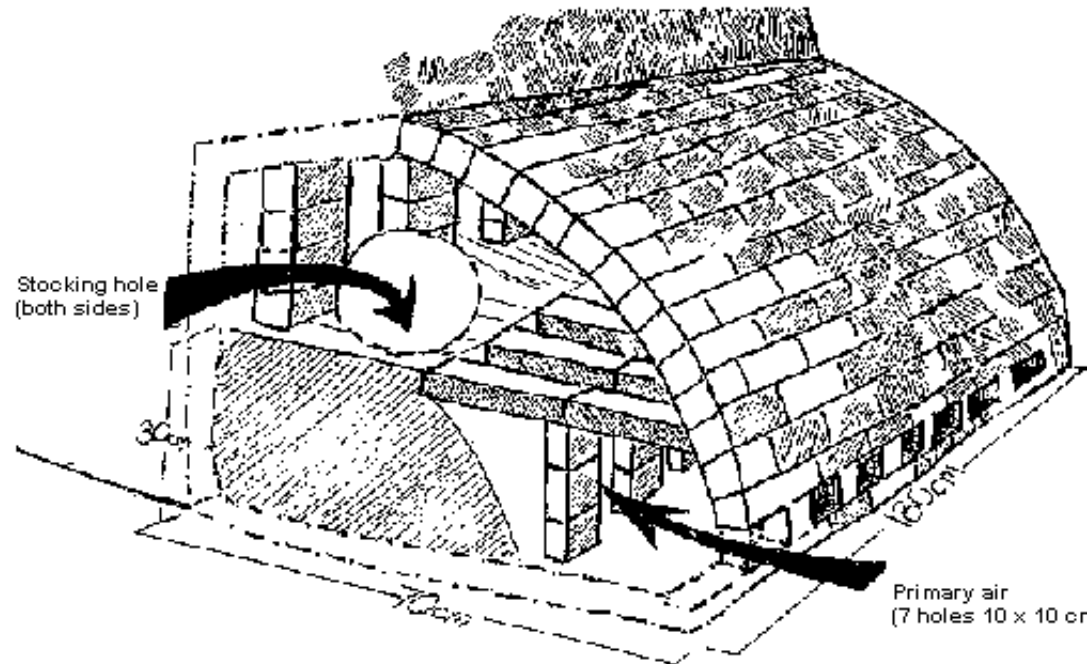
Fig.2-34: Champaknagar firebox.
