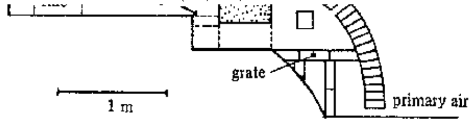
Fig.2-33: Two-chambered wood-fired kiln. Champaknagar, Banladesh.
