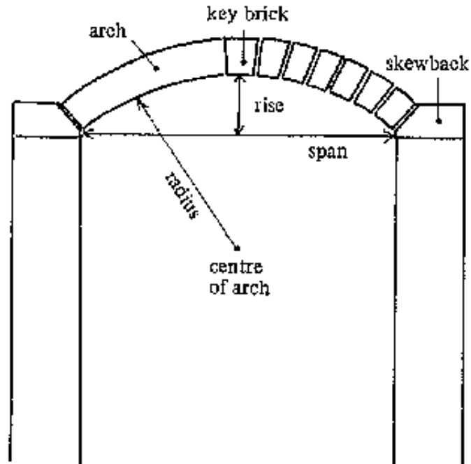
Fig.2-89: Arch.
