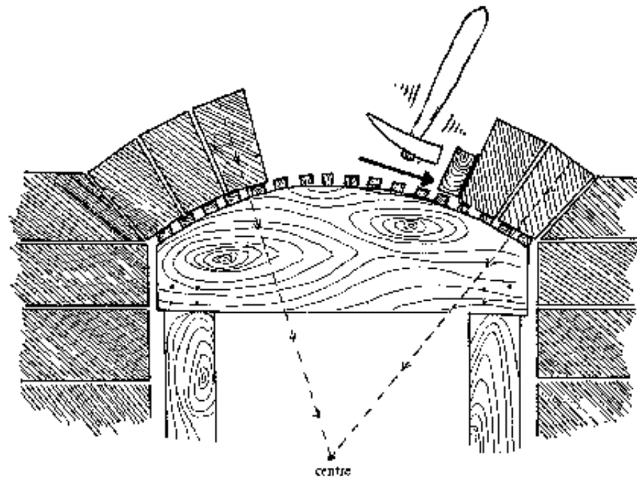
Fig.2-95: Laying the arch
