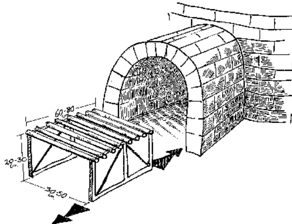
Fig.2-51: Iron grates will last longer if they can be removed after firing has been finished (F.Olsen "The Kiln Book" fastfire wood kiln).
