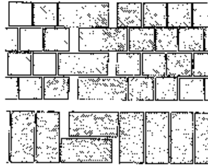
Fig.2-108: Expansion joints in a kiln wall. Side elevation. Fig.2-109: The same expansion joints as in fig. 2-108 seen from the top of the wall.
