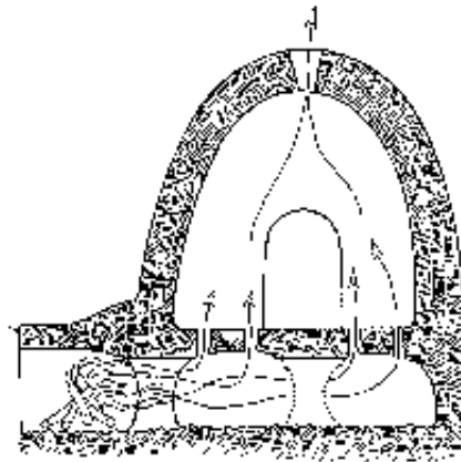
Fig.2-9: Ancient up-draught kiln from Greece
