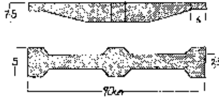
Fig.2-60: Typical grate bars for coal. The thickened parts adjust the open space between the bars.
