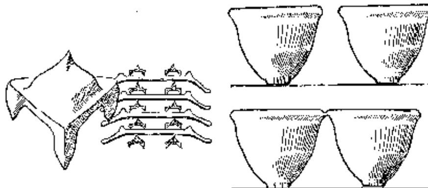
Fig.2-121: Spurs resting on the unglazed bottom of the plates. Fig.2-124: Glazed pots should be placed 3-5 mm apart to prevent them from "kissing".
