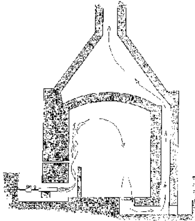
Fig.2-23: The Mayangone kiln is made with flue channels in the walls.
