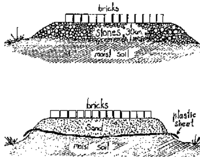
Fig.2-78: A layer of stone pebbles seals off the moisture - Fig.2-79: Plastic sheets with a protective layer of sand work as a moisture seal.
