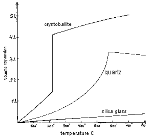
Fig1-3: Three forms of silica with different rates of expansion. The cristoballite expand suddenly at 220 C and quartz expand suddenly at 573 C. When silica has no crystal form as in silica glass or ash it expands evenly.
