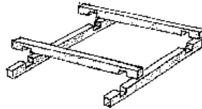
Fig. 1-26: Separable wooden frame for slab-making. The sticks have thickness of the slab
