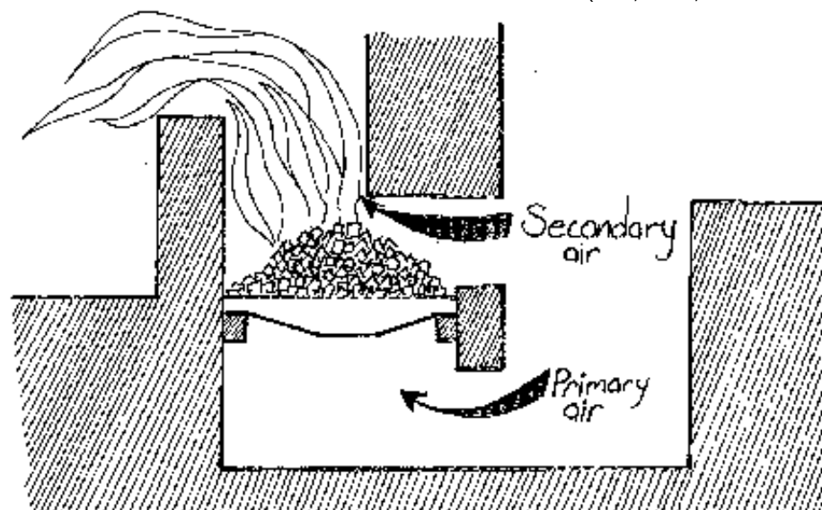
Fig.2-61: Coal firebox with flat grates.
