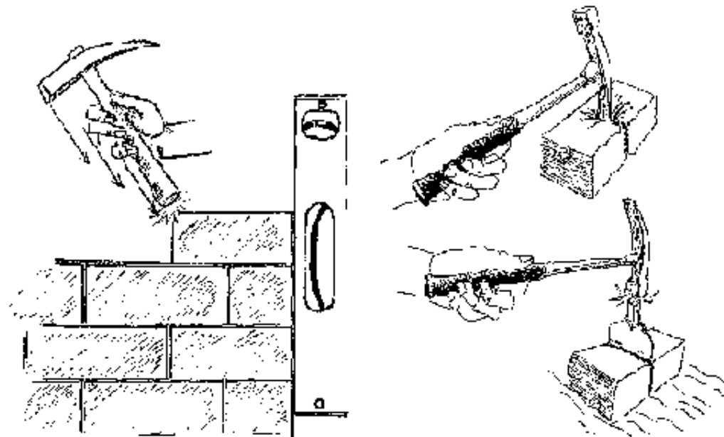
Fig.2-81: Each brick should level vertically with the wall. Fig.2-82: Cutting of firebricks
