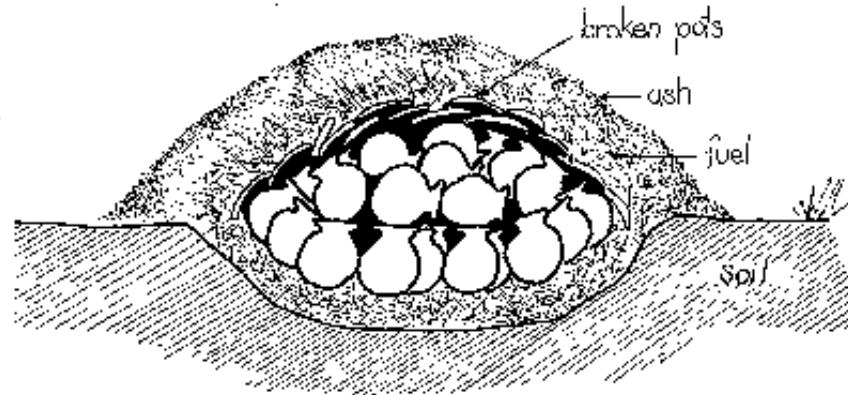
Fig.2-1: Bonfire kiln
