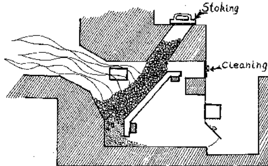
Fig.2-63: Stoking of a semi-gas producer.
