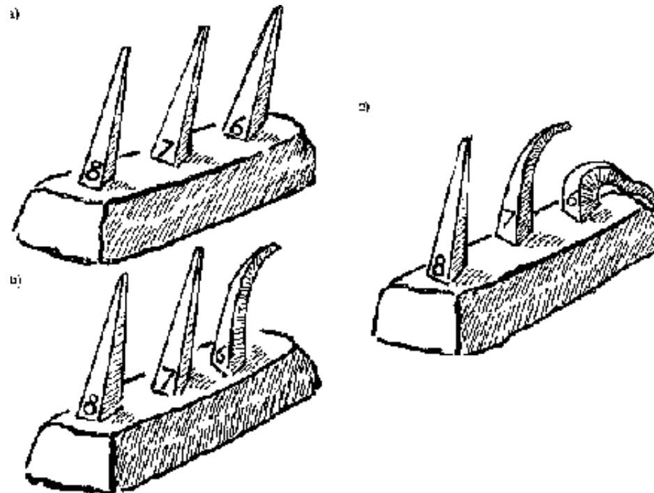
Fig.2-139: Setting of cones: a) Cones should be set similarly at each firing; b) Cone 6 has started to bend, warning the fire-master that the firing is soon to finish; c) Cone 7 is on its way down. When the tip of the cone touches the base the maturing temperature has been reached.
