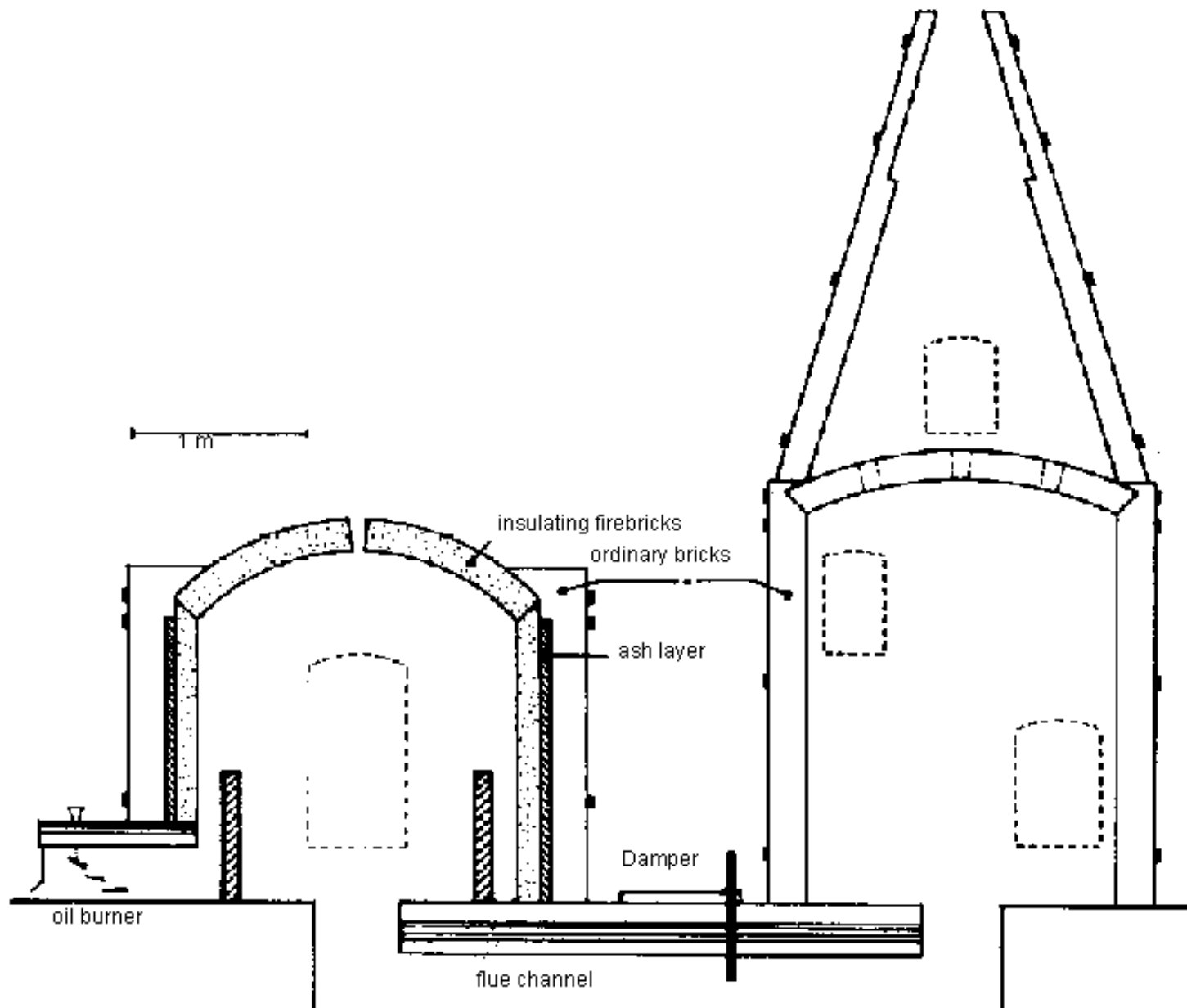
Fig.2-24: Two-chamber Bujora kiln, cross-section. The first chamber is provided with three fireboxes for oil firing but fireboxes for firewood or coal could be used as well.
