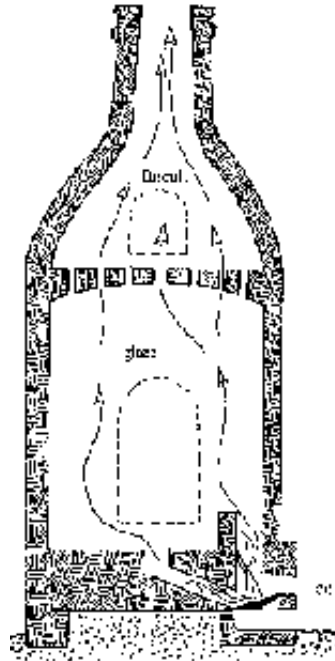
Fig.2-12: Bottle kiln with its innovations: chimney, firebricks and iron grates for burning coal.
