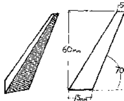
Fig.2-141: Shape and dimension of cones.
