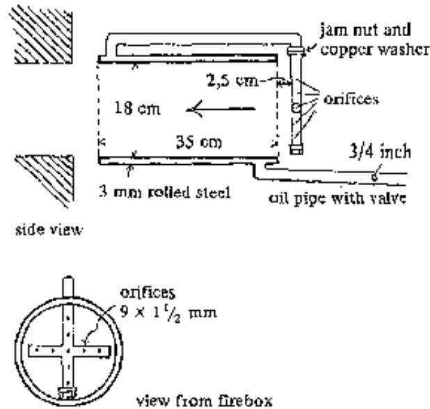
Fig.2-70: Large pressure burner.
