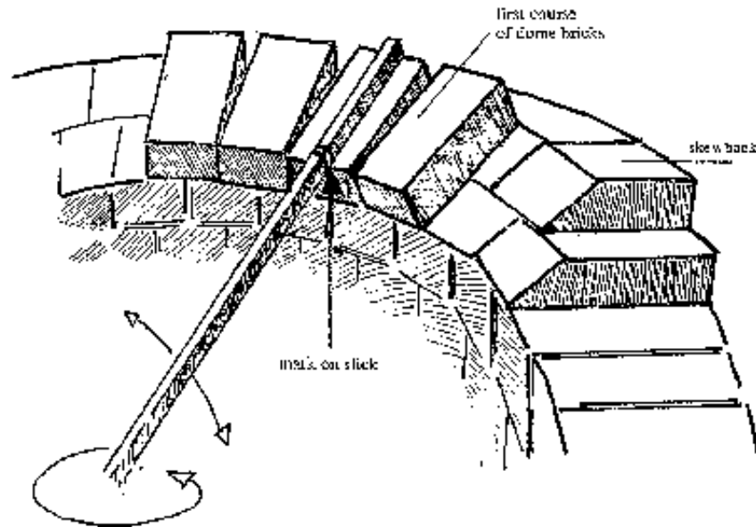
Fig.2-100: Skewbacks are laid as headers.
