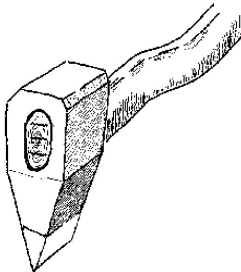
Fig.2-38: Special axe for splitting firewood. The axe does not cut the wood but splits it by impact. It is not suitable for splitting wood with long fibres.
