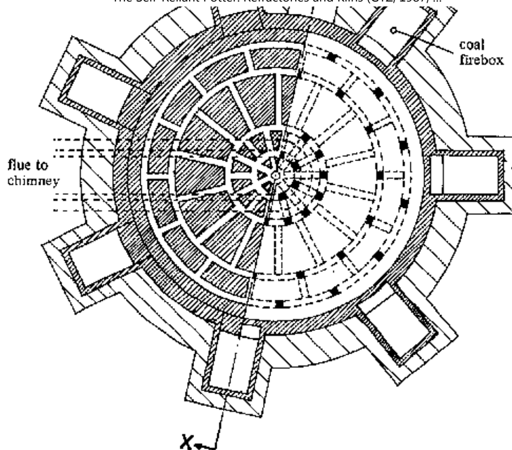
Fig.2-19: Khurja down-draught kiln a) side elevation, b) ground elevation showing flue holes and chanel. The details for this kiln have been obtained from "Status Report on Ceramic Industry at Khurja", published by Central Glass and Ceramic Research Institute, Calcutta, India.
