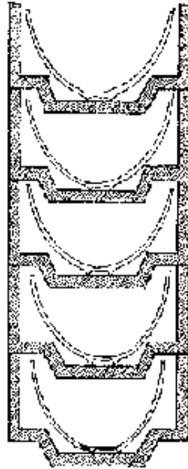
Fig. 1-16: Saggars shaped for dense setting of blows
