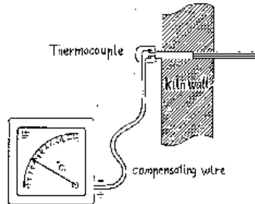
Fig.2-140: Pyrometer
