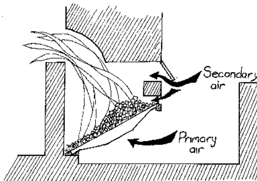
Fig.2-62: Coal firebox similar to the ones seen in fig.2-59. The firebox is within the outer wall of the kiln. Secondary air is regulated by opening of the stoking shutter
