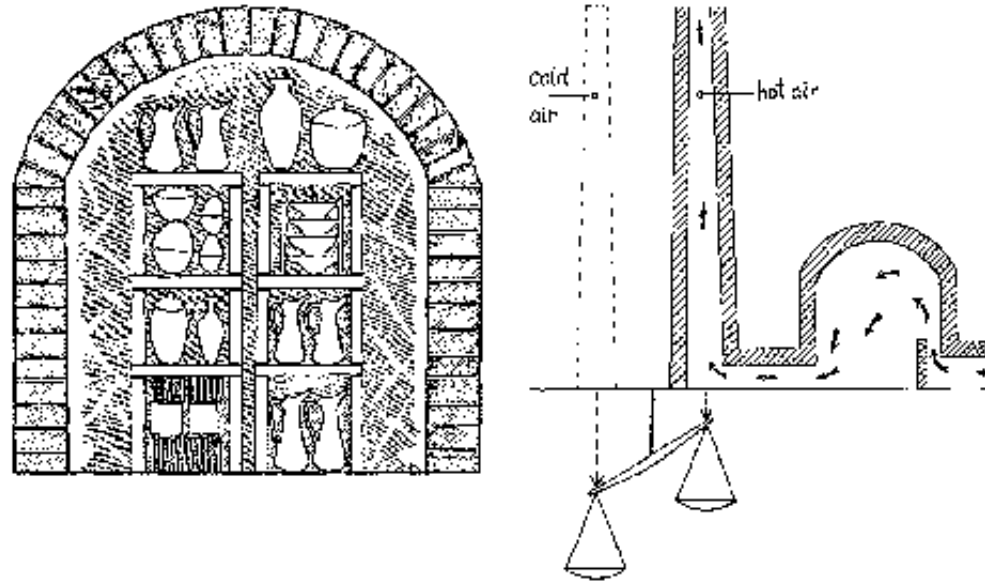
Fig.2-72: At red heat the kiln walls will radiate heat back to the kiln setting. Fig.2-73: The hot air the chimney weighs much less than cold air of the same volume. The balance illustrates this weight difference.
