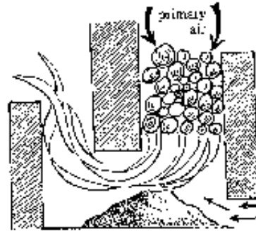
Fig.2-52: Hob firebox.
