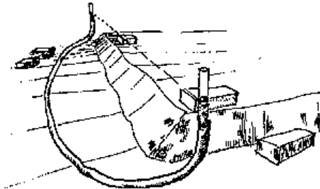
Fig.2-77: Levelling of the foundation by the help of a hose
