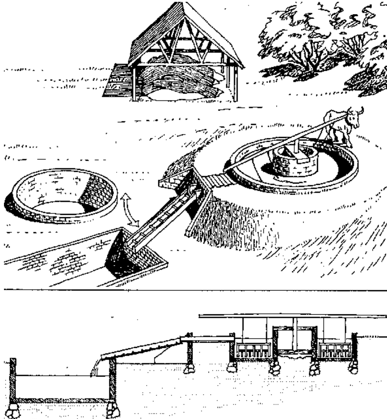
Figure 1-7 Animal powered washmill for clay cleaning. A grooved tray leads to the
