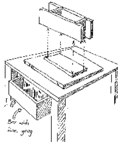
Fig. 1-38: Stock mould fixed to a solid table
