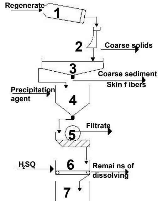
1: Tanning mixer, 2: Bow Sieve, 3: Holding and primary settling tank, 4: Precipitation and settling tank, 5: Filter plant (drum filter), 6: Treatment tank, 7: Storage tank
