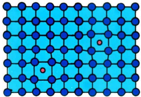
Interstitial atoms
