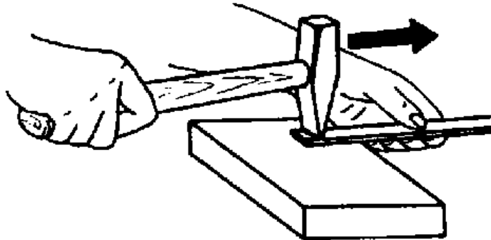
Figure 15 Lengthening with hammer pane
