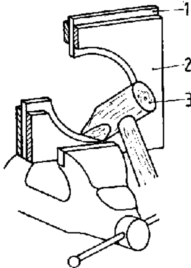
Figure 22 Rough-flanging: bending down of the inside border
