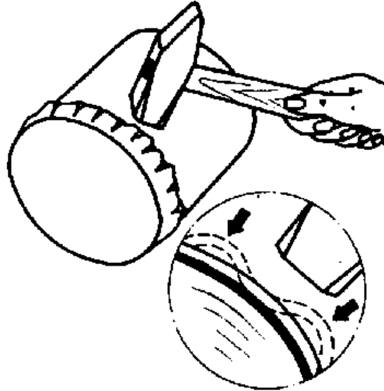
Figure 21 Finish-flanging: bulging in and smoothing of puckers
