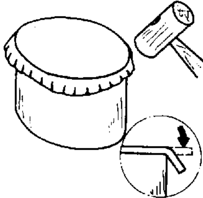
Figure 20 Rough-flanging: bending down of the outside border
