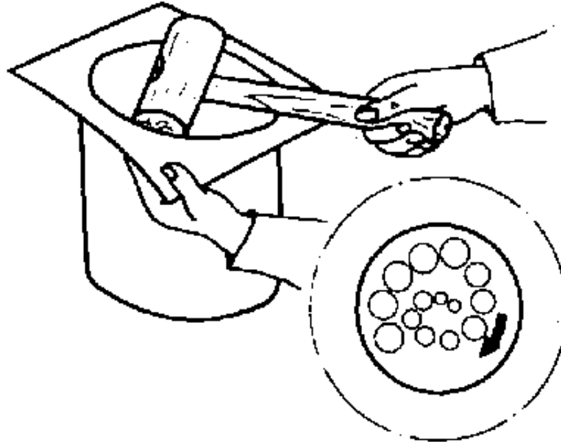
Figure 19 Chasing on hollow hammering support
