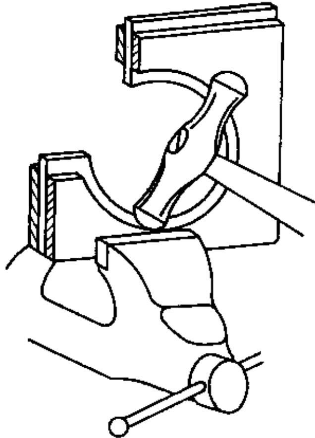
Figure 23 Finish-flanging: bulging in and smoothing of puckers
