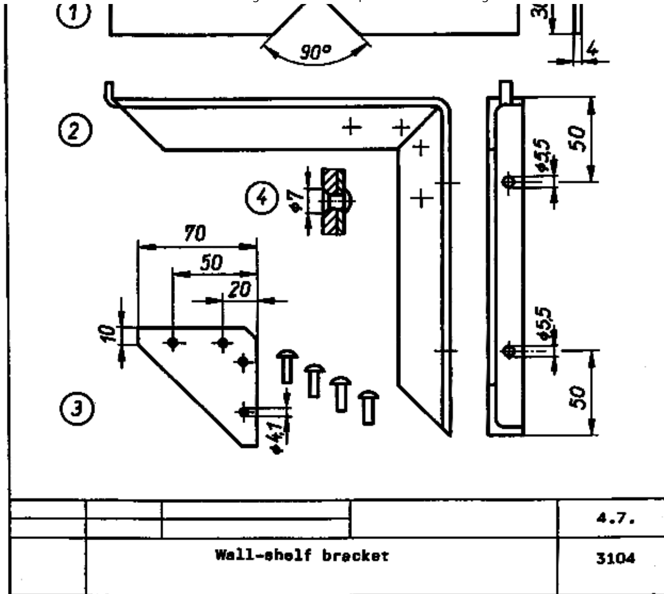
Wall-shelf bracket
