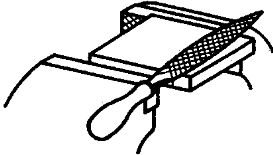
Figure 14 Filing of the guiding groove
