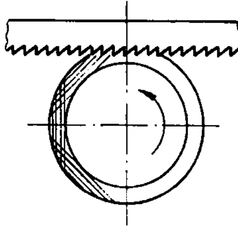
Figure 17 Sawing of tubes with multiple re-clamping
