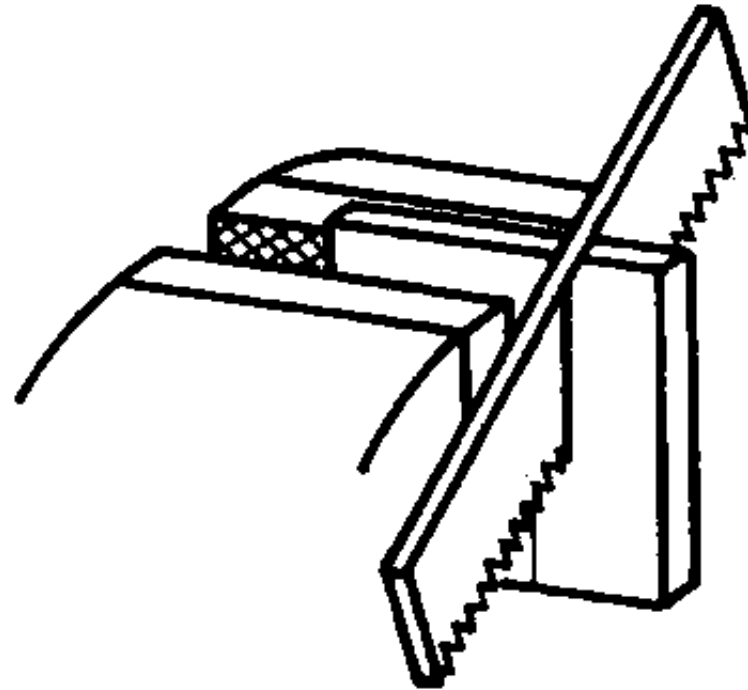
Figure 16 Sawing of sheets in upward pushing direction
