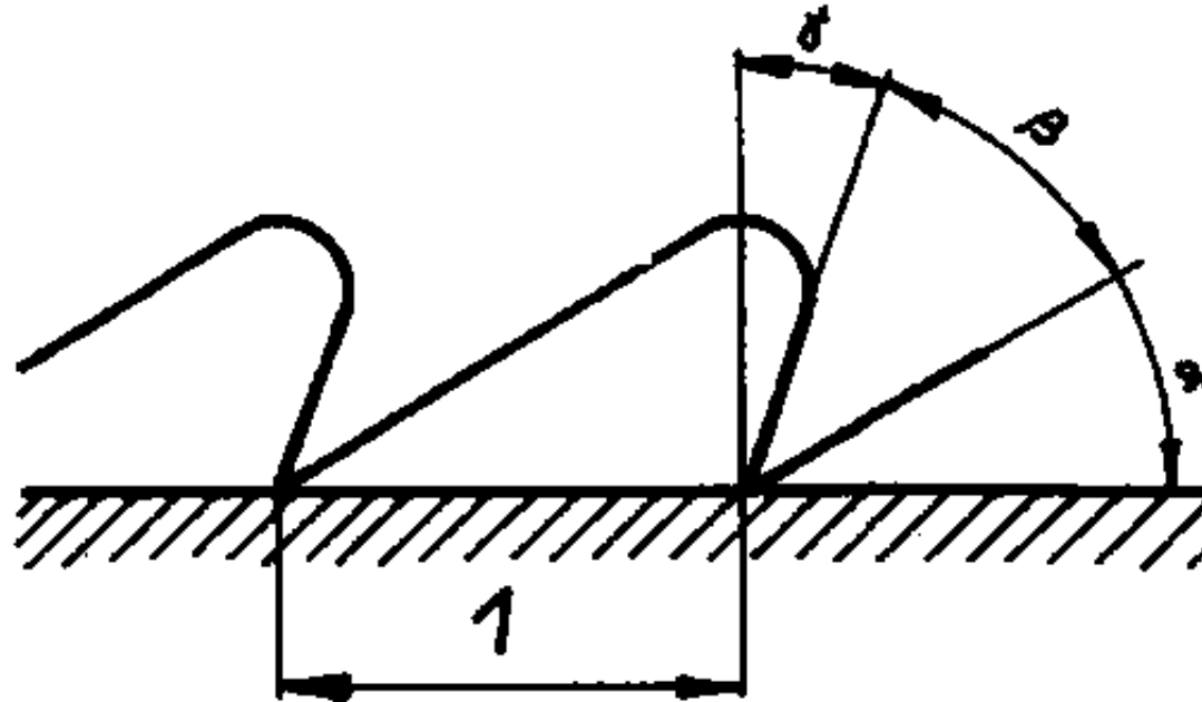
Figure 4 Angles at the saw tooth
