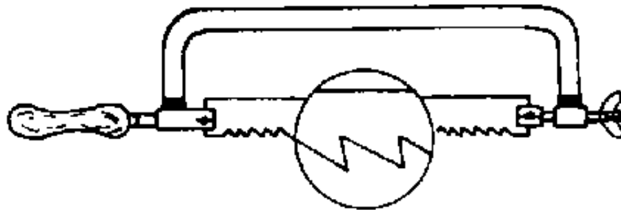
Figure 13 Correctly clamped saw blade
