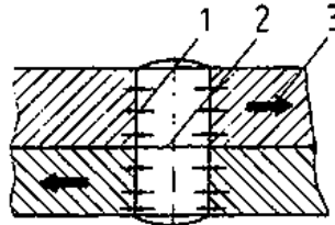
Figure 14 Stresses in Pinned Joints
