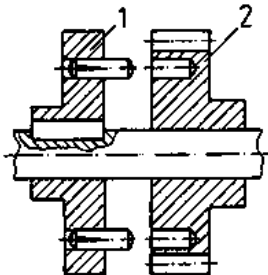
Figure 8 Pinned joint for driving
