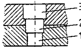
Figure 22 Drilling steps (1-2-3)
