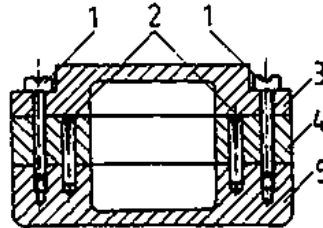
Figure 11 Pinned joint for fitting
