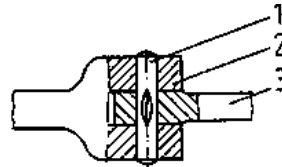
Figure 10 Pinned joint for hinging
