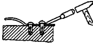
Figure 26 Undoing a grooved drive stud joint
