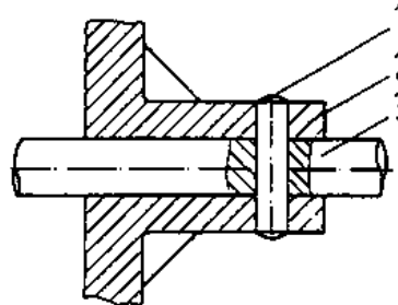
Figure 1 Pinned joint
