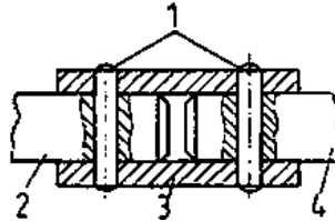
Figure 13 Pinned joint for shearing
