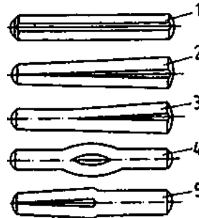
Figure 4 Grooved pins
