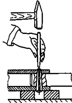
Figure 24 Undoing a pinned joint with a drift
