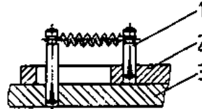
Figure 9 Pinned joint for holding
