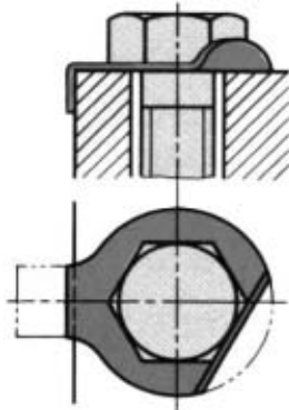
Locking Plate tongued outside
