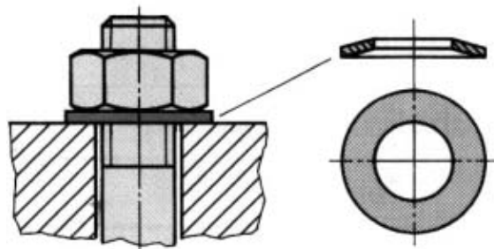
Conical Spring Washer
