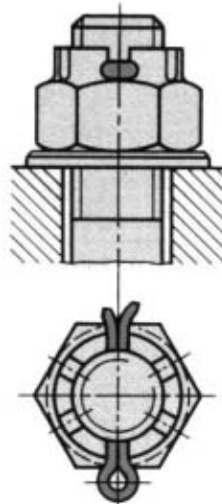
Castel Nut with split-pin
