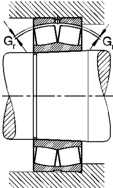
Radial clearance reduction in spherical roller taper 1:30
