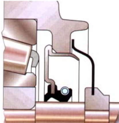
Restricted Space
