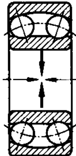
Self-Aligning Ball Bearing
