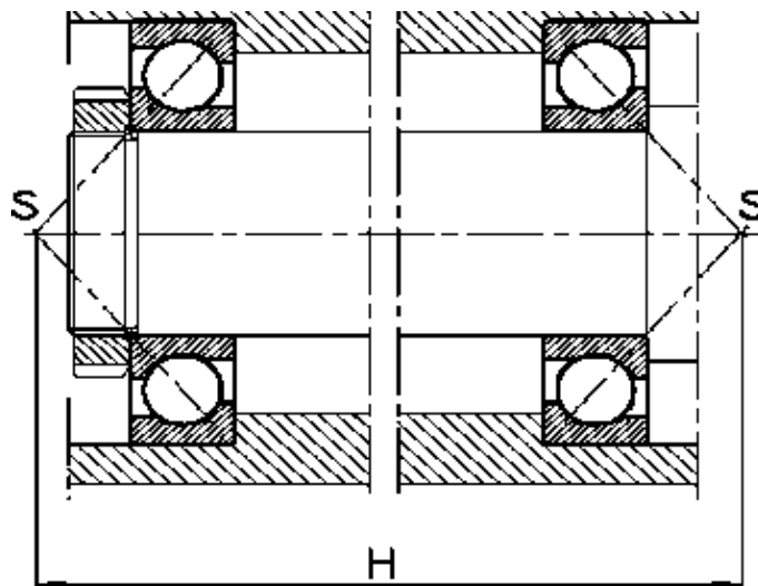
Adjusted Angular Ball Bearings in "O" Arrangement
