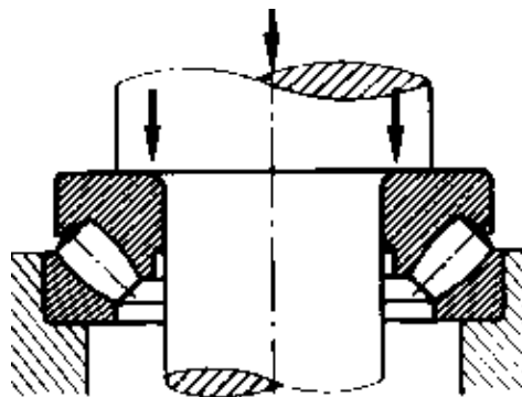
Spherical Roller Thrust Bearing
