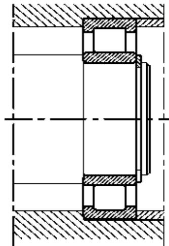
Floating Bearing Cylindrical Roller Bearing NU
