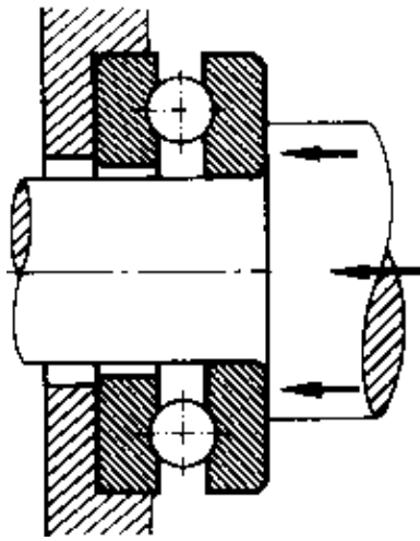
Thrust Ball Bearing
