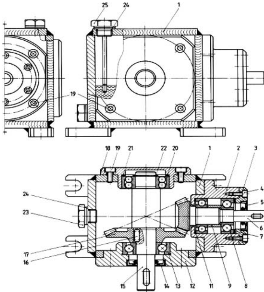
List of parts: Bevel Gear Drive
