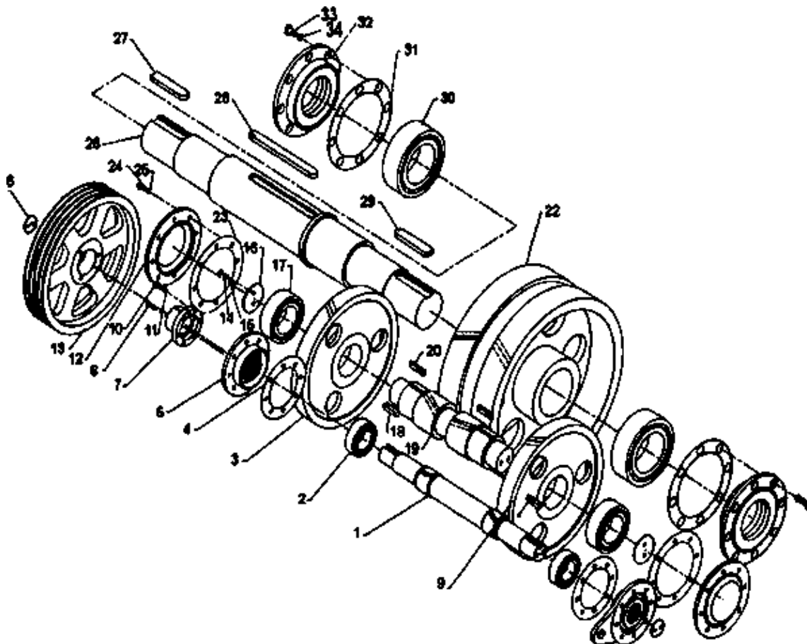
International Gear Reducer Assembly
