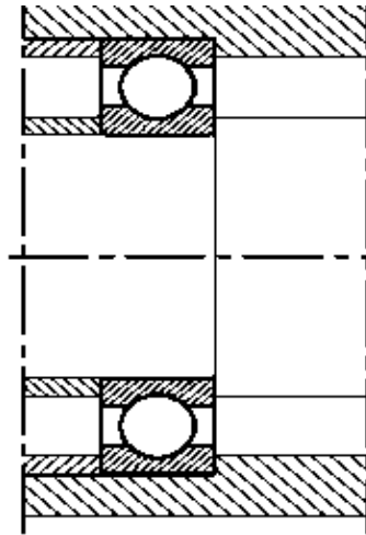
Locating Bearing Deep Groove Ball Bearing
