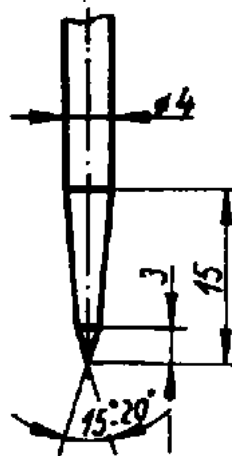
Figure 11 - Dimensions of the scriber
