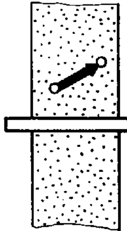
Figure 16 - Upward movement of the drill
