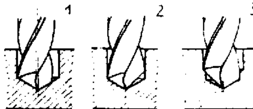
Figure 18 - Consequences of grinding faults (explanations 1,2,3 in the text)
