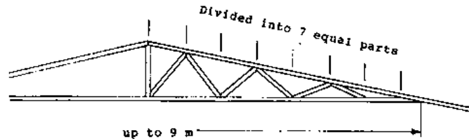
Span up to 9 m.
