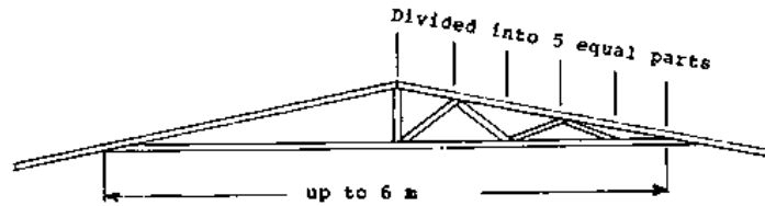
Span up to 6 m.
