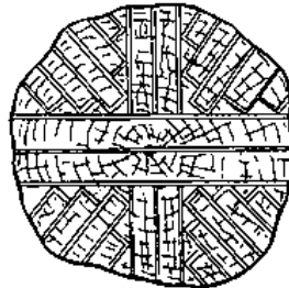
Quarter sawing (Radial cut)
