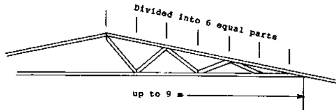
Span up to 9 m.
