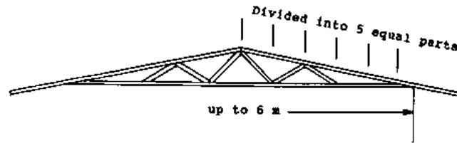
Span up to 6 m.
