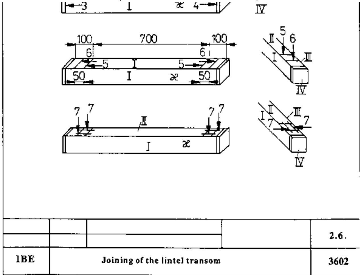
Joining of the lintel transom
