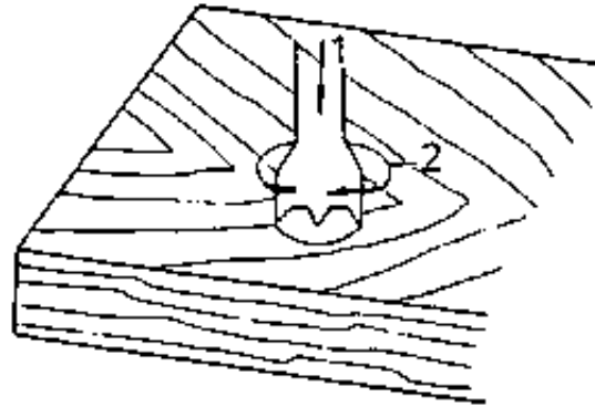
Figure 9 Boring forces
