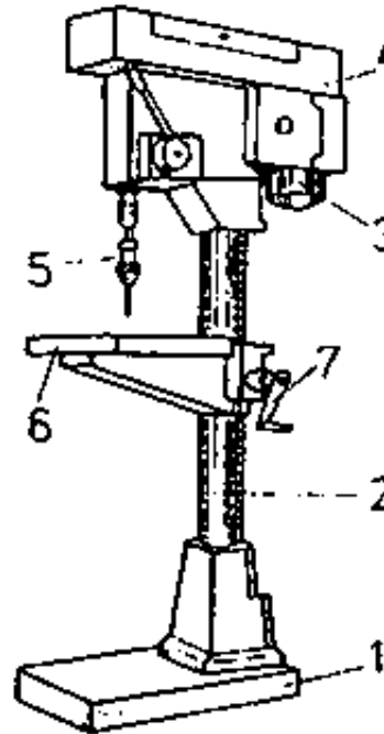
1 base plate, 2 column, 3 driving motor, 4 spindle drive, 5 drilling spindle with drill, 6 work supporting table, 7 hand crank for table height adjustment
