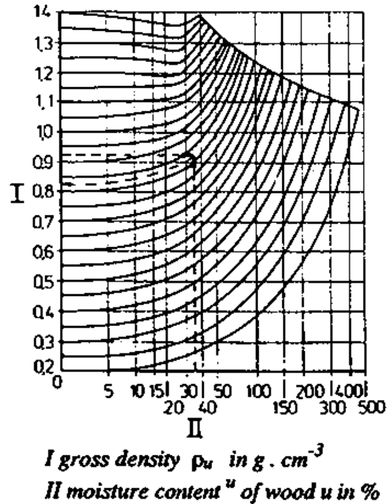
Figure 2 Plot of gross density and moisture content
