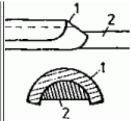
1 turning tool, 2 Setting-up of the plane shaped stone iron flap
