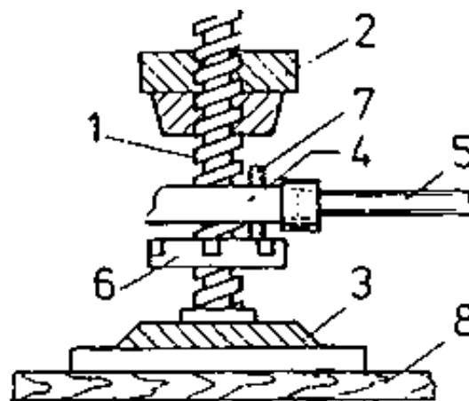
Figure 26 Hand screw press
