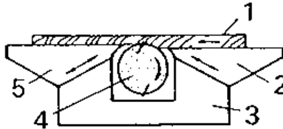
1 stop rail, 2 adjustable feed table, 3 machine frame, 4 blade shaft, 5 adjustable unloading table
