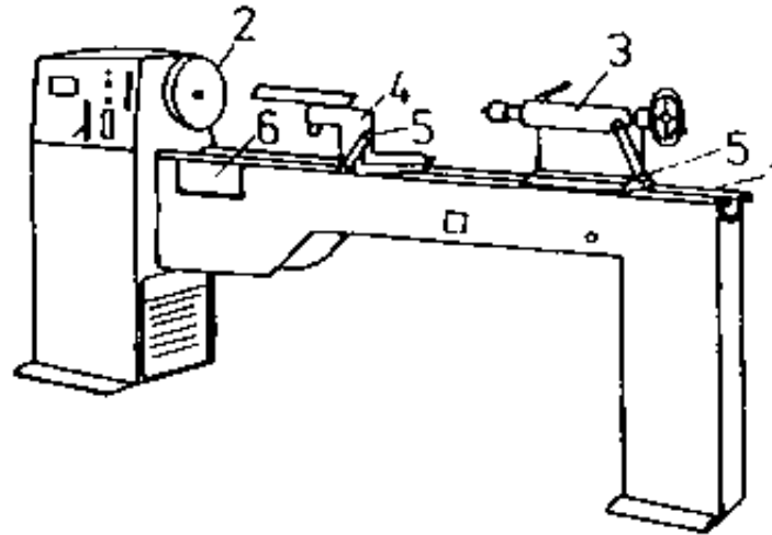
1 machine bed, 2 spindle, 3 tailstock, 4 rest, 5 eccentric, 6 gap
