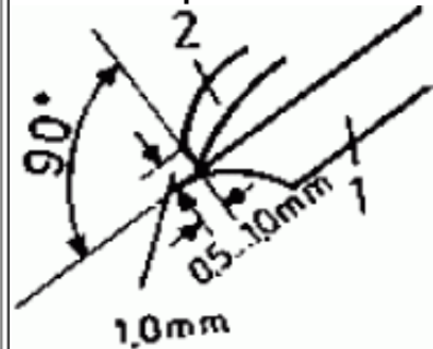
1 plane iron, 2 flap
