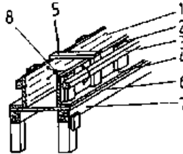
Figure 11 Beam formwork
