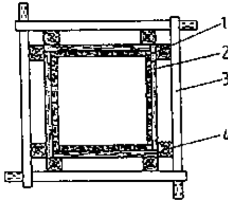
Figure 12 Column formwork (horizontal section)
