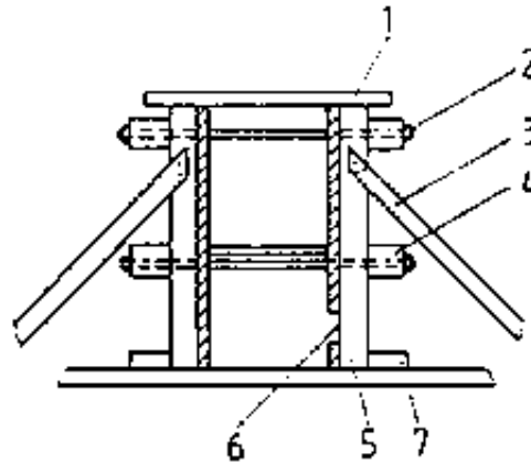
Figure 8 Wall formwork (vertical section)
