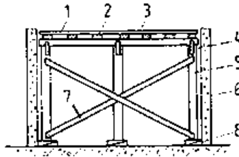
Figure 9 Ceiling formwork (vertical section)
