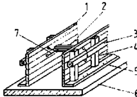
Figure 7 Foundation formwork
