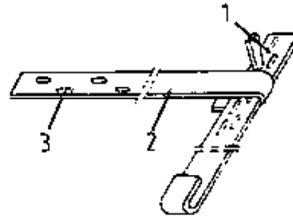
Figure 5 Steel clamp corner point for column formwork
