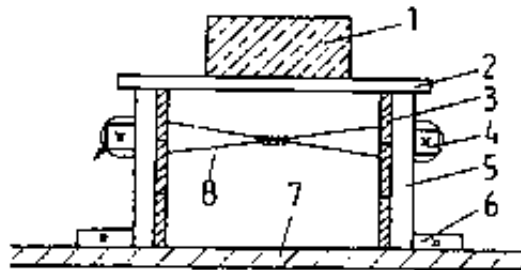
Figure 2 Formwork tying by loads on the formwork
