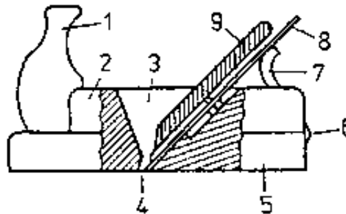
Figure 1 Parts of the plane
