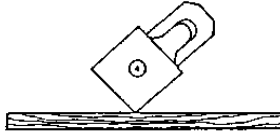
Figure 21 Returning the plane
