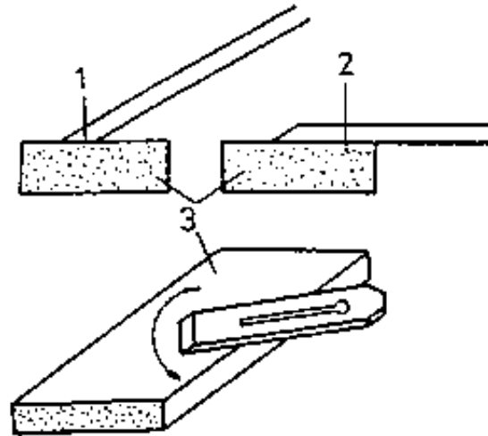
Figure 10 Stoning of the plane iron
