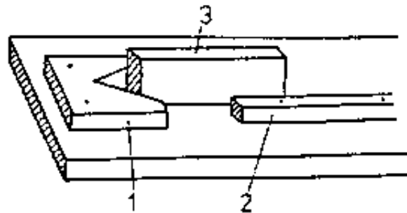
Figure 15 Clamping board to plane on sites
