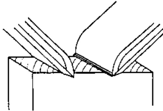
Figure 28 Working directions for planing of narrow faces of end-grained wood
