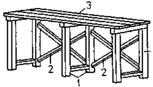
Figure 14 Site workbench
