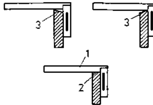
Figure 27 Checking of squareness of the wide face to the narrow face
