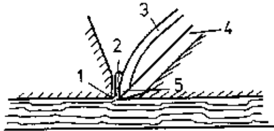
Figure 4 Breaking of the wood shaving
