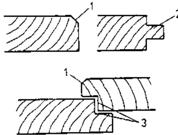
Figure 31 Profiles at narrow faces and edges
