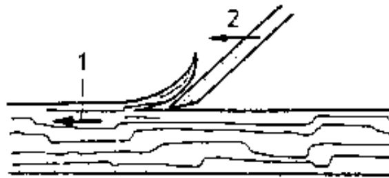
Figure 17 Correct working direction for planing
