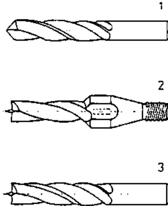
Figure 4 - Twist drill
