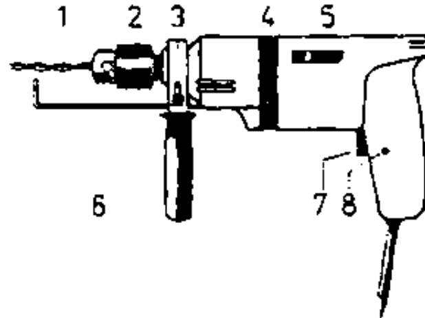
Figure 2 - Electrical hand drilling machine
