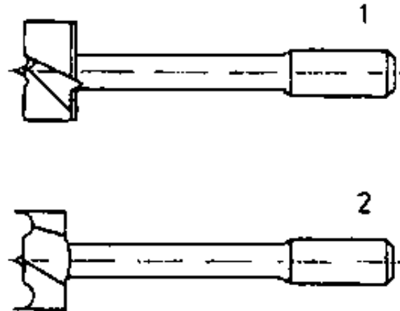
Figure 6 - Cylinder drill
