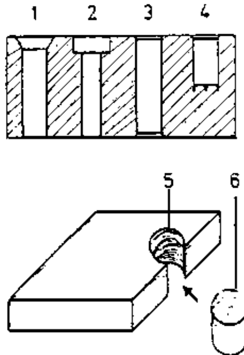
Figure 1 - Bore types
