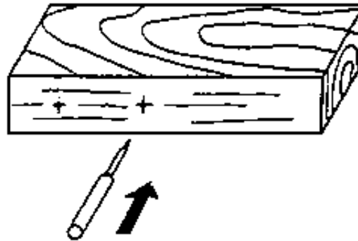
Figure 7 - Marking and punching of the bore centres
