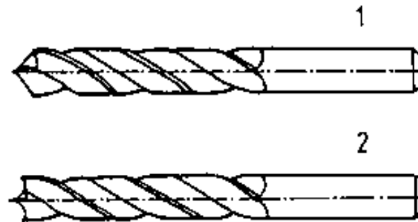
Figure 4 - Twist driller
