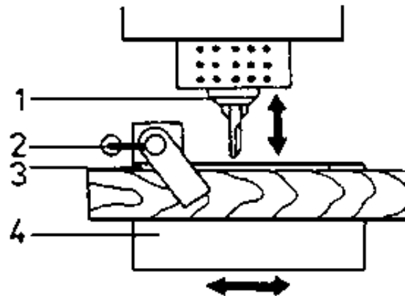
Figure 3 - Fastened wooden boards
