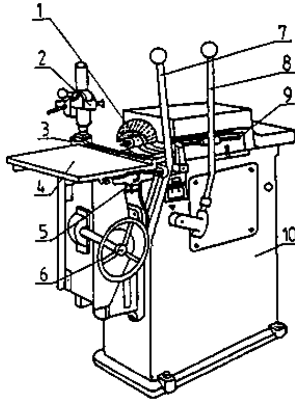
Figure 2 - Construction of a long-hole cutting machine
