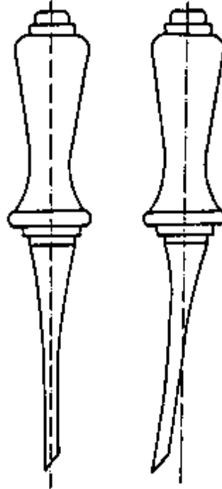
Figure 3 Requirements on mortising tools
