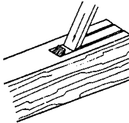
Figure 21 Splitting off the wood chips
