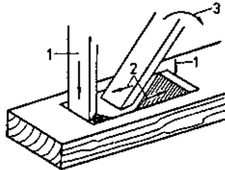
Figure 26 Alternately chiselling out the opening
