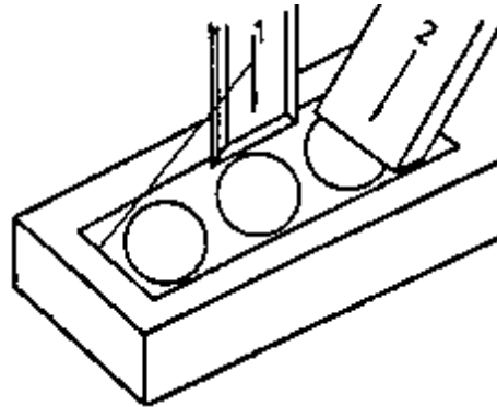
Figure 27 Chiselling out predrilled holes
