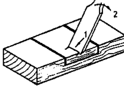
Figure 16 Driving in and bending the firmer chisel
