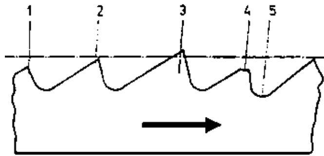
Figure 21 Badly filed saw teeth
