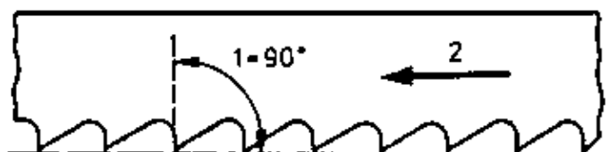
Figure 4 Push-type cutting teeth
