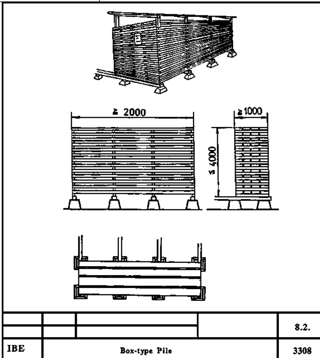
Box-Type Pile
