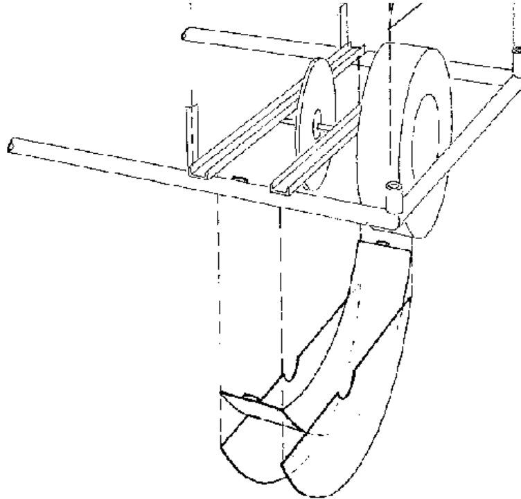
Fig 38: Arrangement of the protective coverings on the frame
