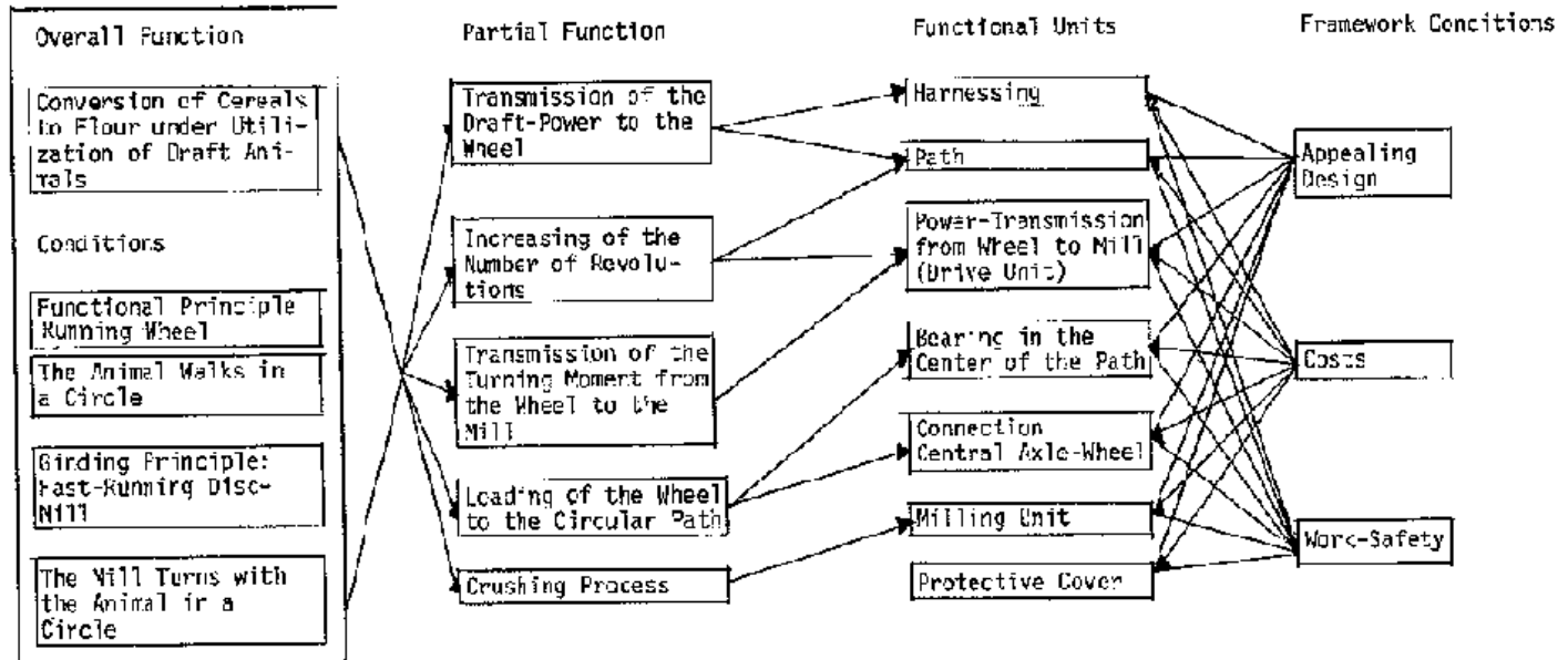
FIGURE 12: Functional diagram of the animal powered mill.
