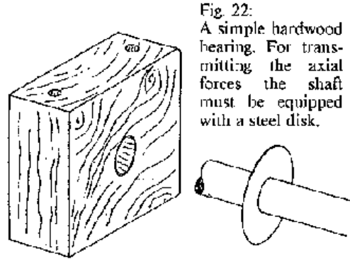
Fig. 22:A simple hardwood bearing. For transmitting the axial forces the shaft must be equipped with a steel disk.
