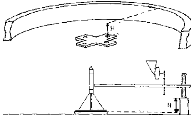
Fig. 31: Determination of the foundation height
