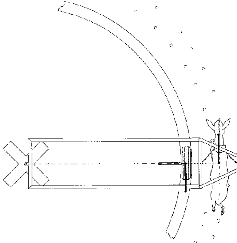
Fig. 15: Power losses are avoided by harnessing the draft animal to a semi-circular harness]
