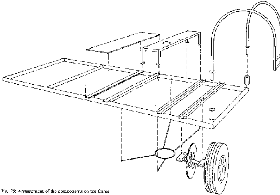
Fig. 28: Arrangement of the components on the frame
