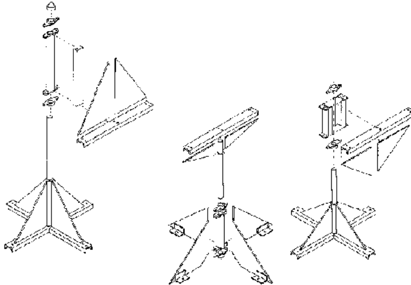
Fig. 32: Different constructions of the central axle
