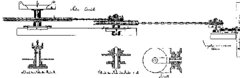
Fig. 3: A "chain power gear" patented in the German Reich in 1879
