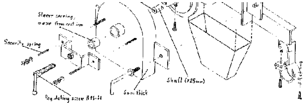
Fig. 36: Components of the locally constructible grinding unit
