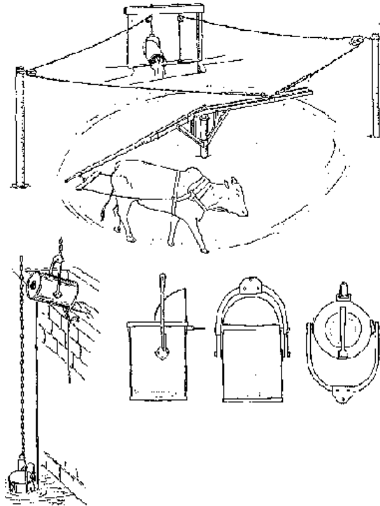
Fig. 32: Stoney's Mote, basic concept
