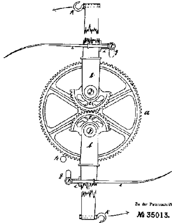
Fig.: "Power gear with self-acting device for the equalization of tractive forces and
