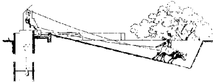
Fig.: Delou with an automatic emptying arrangement
