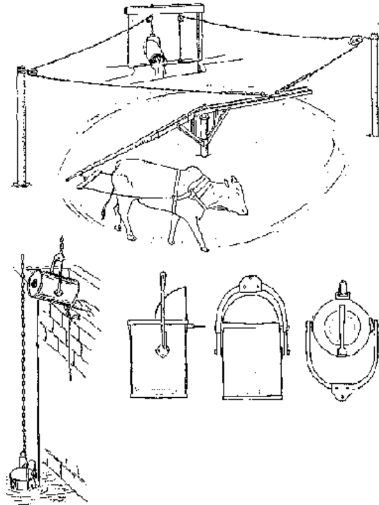
Fig.: Manège du Jardinier - once used for well building
