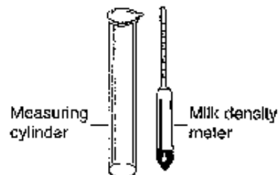
Figure 9. Measuring the density of milk
