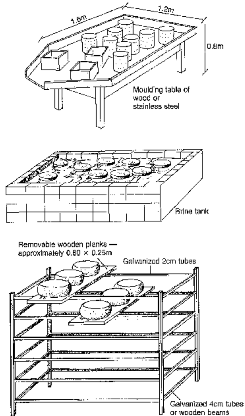
Figure 21. Basic equipment for the cheese factory
