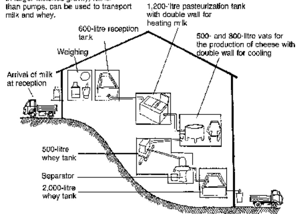
Figure 19. Gravity circuit of a 2,000-litre cheese factory
