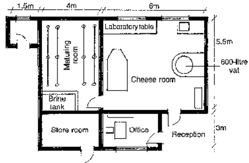
Figure 20. Plan of a 600-litre-capacity cheese factory (1:75 scale)
