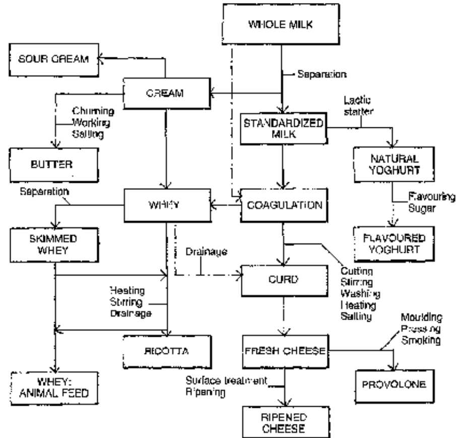
Figure 2. Flow chart of the transformation of milk into cheese and its by-products Traditionally salt was used in cheesemaking in order to preserve the product for a longer period. However, today conservation can be achieved by the use of lactic cultures, so that over-salting is no longer necessary.
