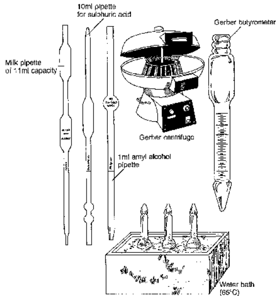
Figure 8. Equipment for testing fat content
