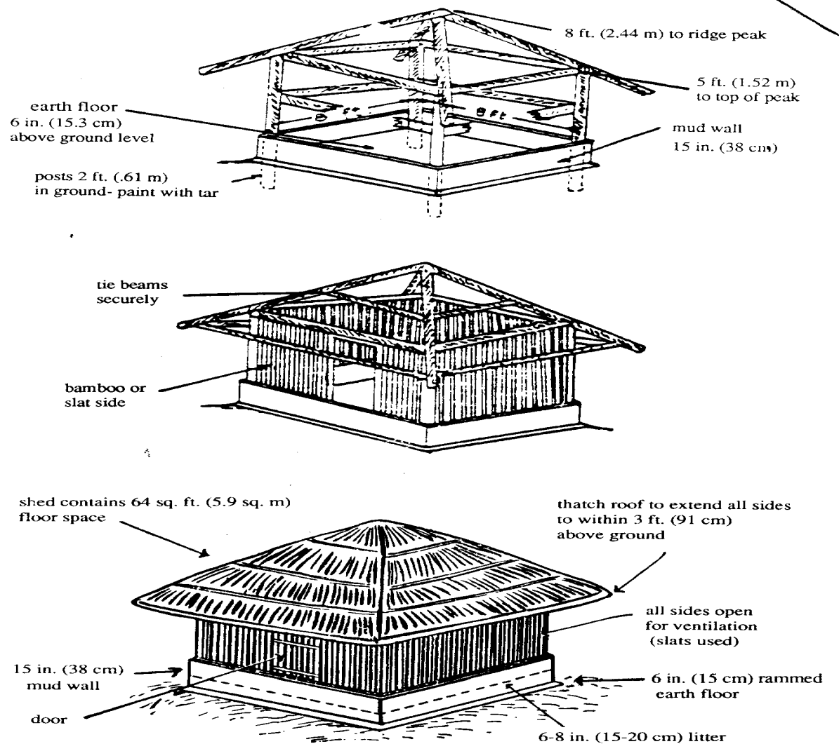
Figures 7 Building a deep-litter shed
