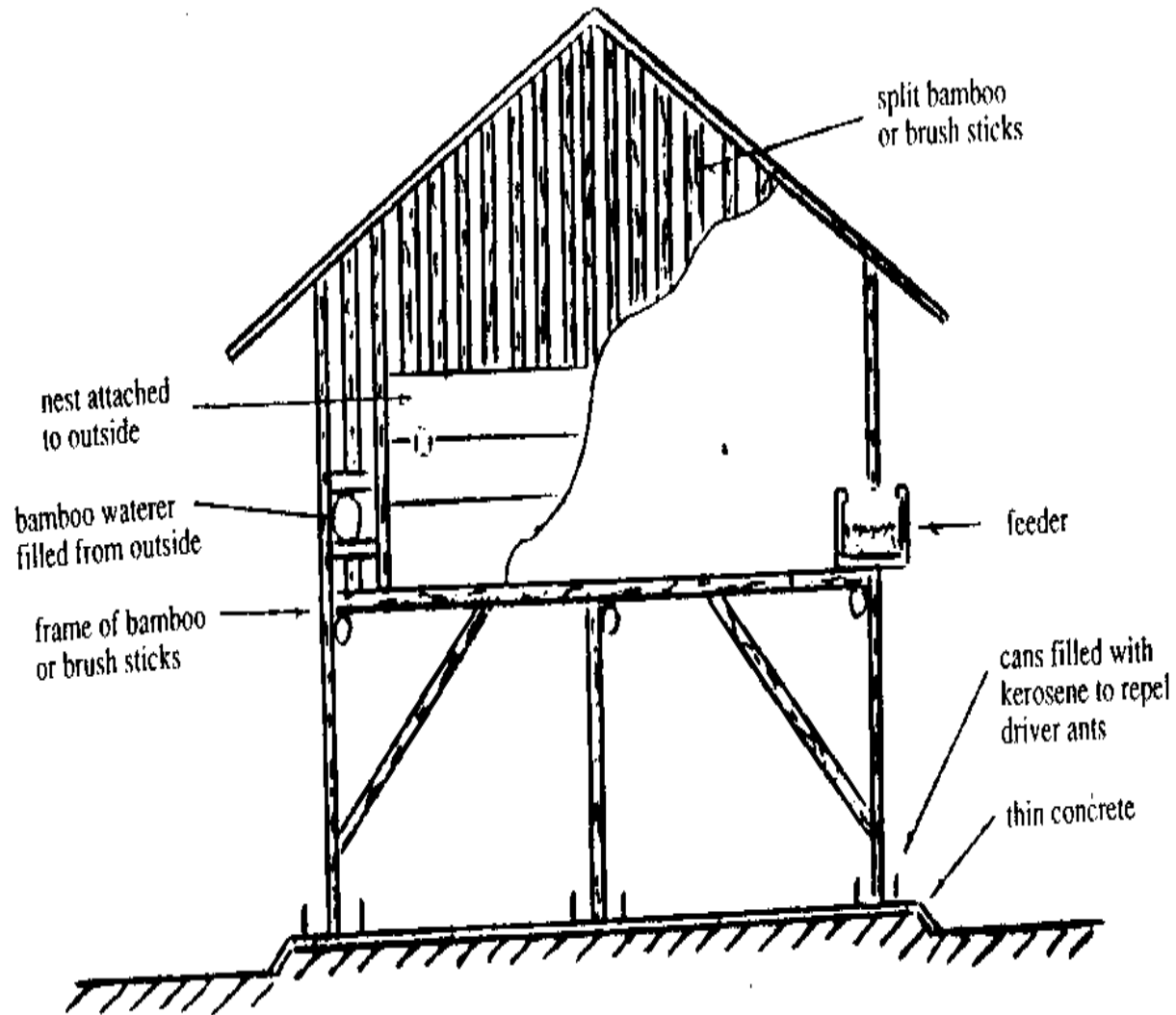
Figure 3 Slatted-Floor Poultry House
