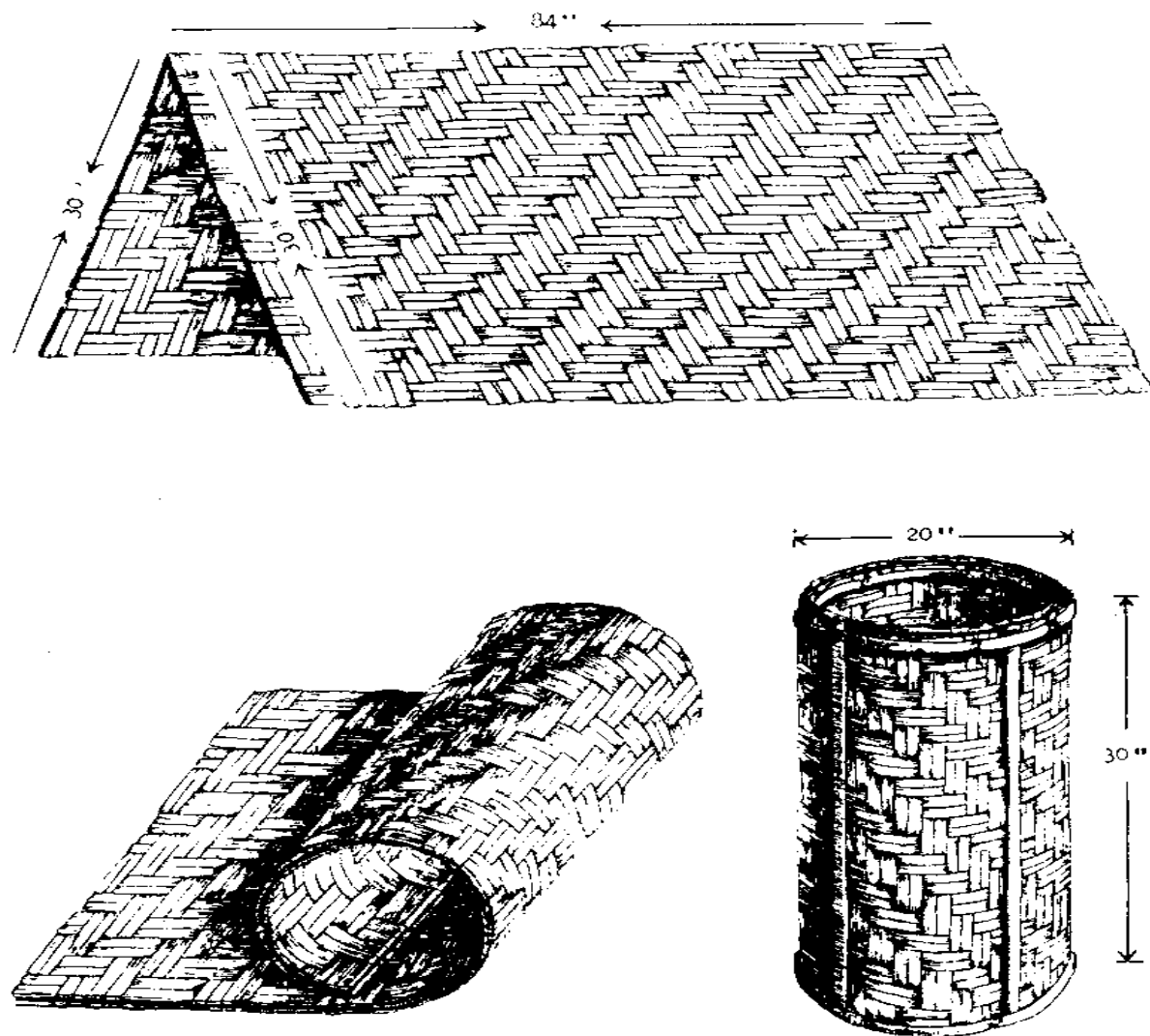
Figure 8 Making a cylinder for 900 eggs.
