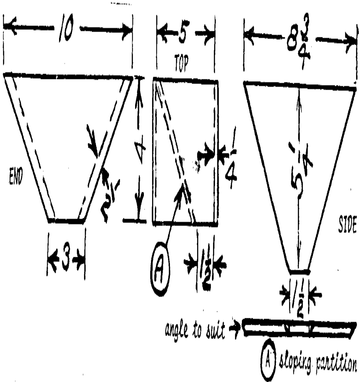
(7) Dribbler Trough Height Adjustment Bar. Use 3/4" thickness pine.
