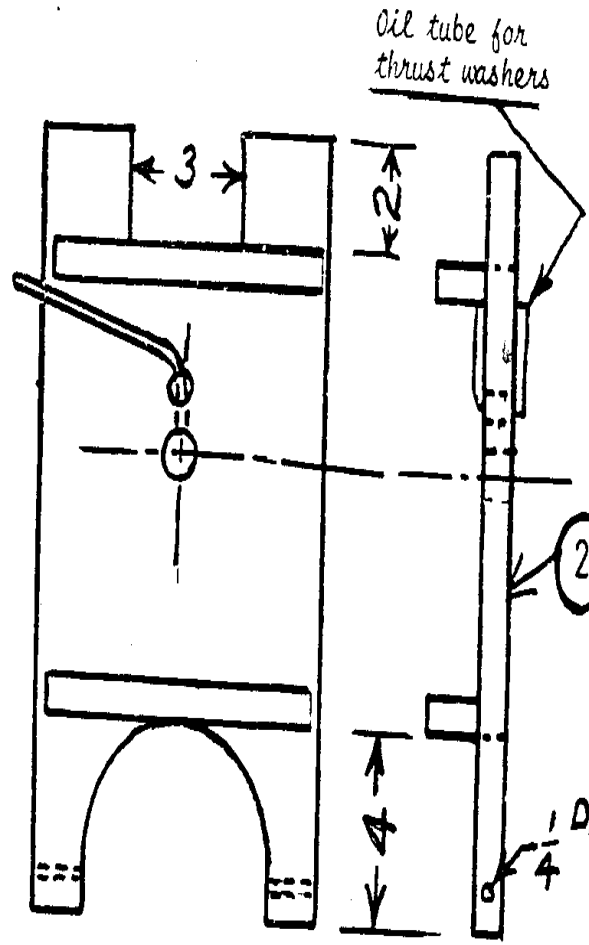
④ Center Bulkhead. Overall dimensions same as detail ③, note other variations.
