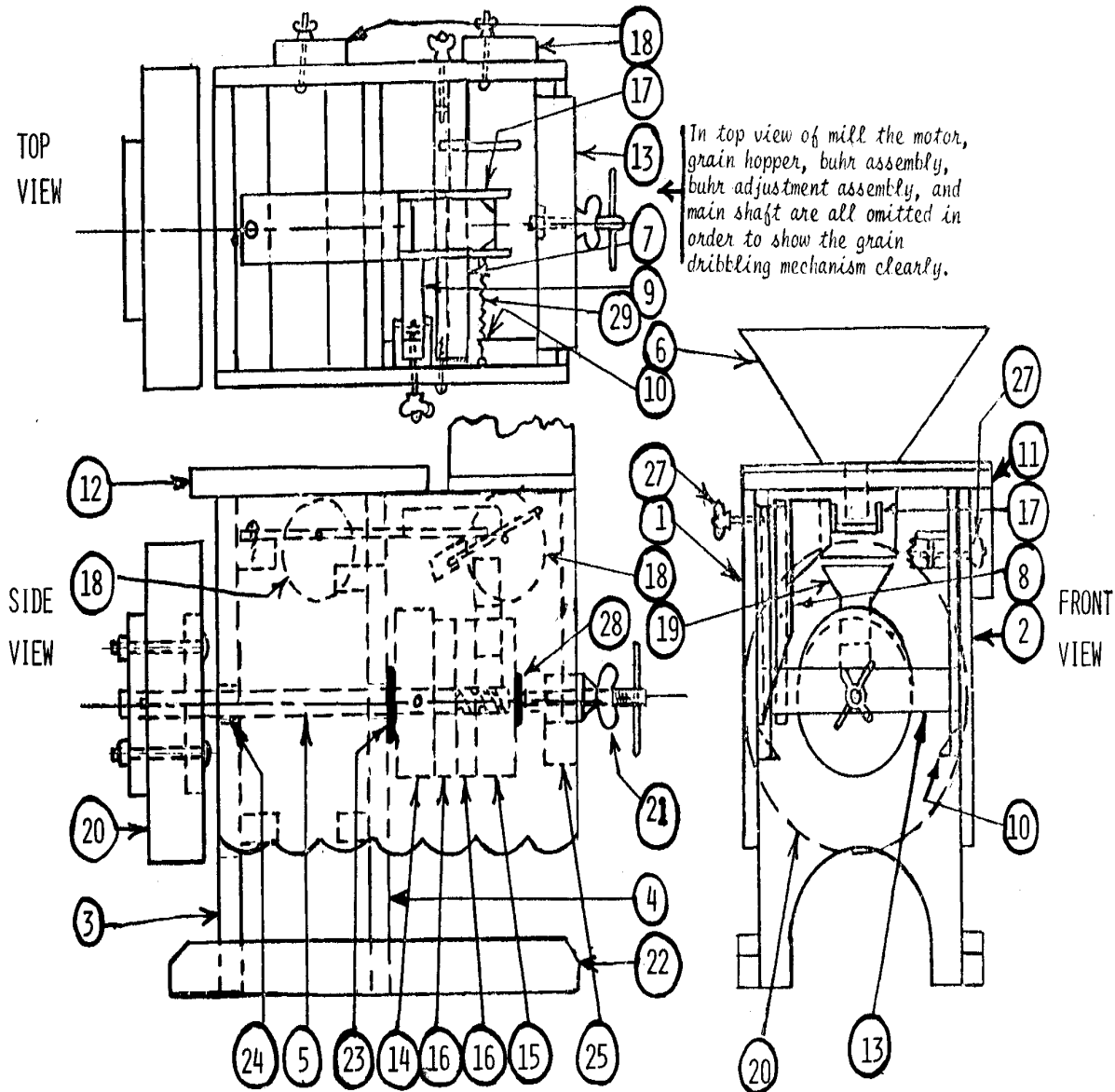
ASSEMBLY DRAWING OF MILL
