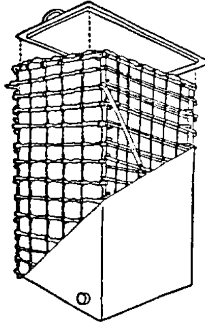
Fig. 54 Air-tight wattle and daub grain store, Sierra Leone
