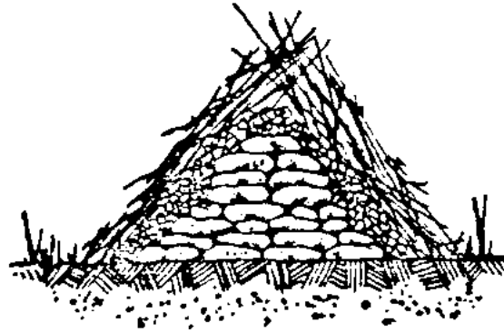
Fig. 37 In the field potato clamp
