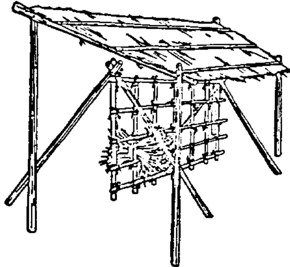
Fig. 8 Improved post-harvest air-dryer for rice, Sierra Leone
