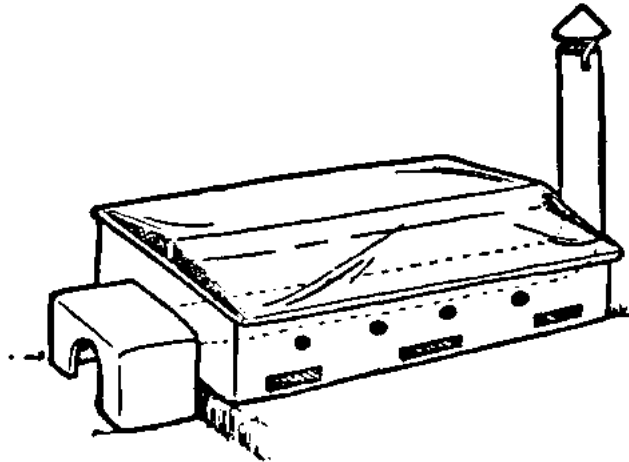
Fig. 15 VITA solar dryer with fuel-fired rainy season dryer attached
