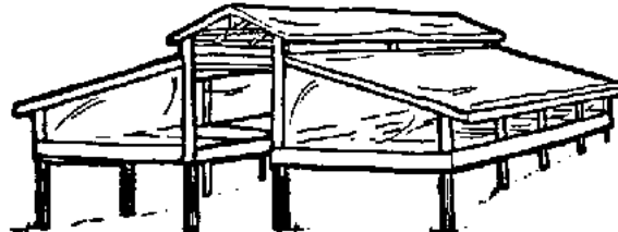
Fig. 19 Walk-through, plastic-covered, solar coffee dryer, Columbia
