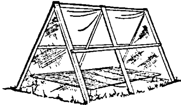
Fig. 12 Solar tent dryer, Philippines
