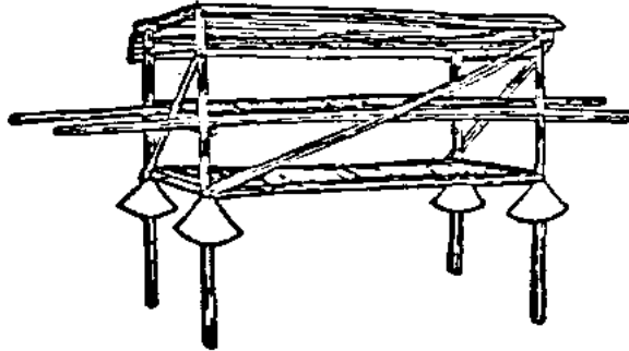
Fig. 16 Improved air dryer/store, Sierra Leone
