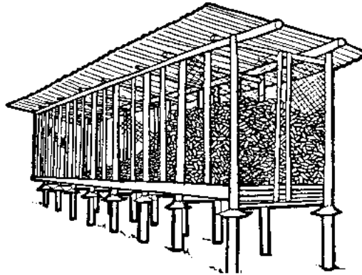
Fig. 59 Improved maize crib,
