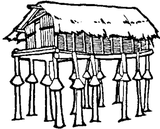
Fig. 42 Dungu, improved with rat guards, Tanzania
