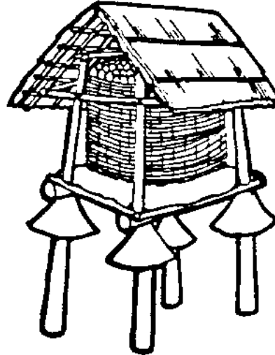
Fig. 48 Traditional store improved with rat guards
