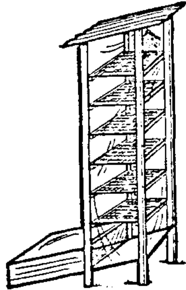
Fig. 17 Solar "chimney" dryer with pre-heater
