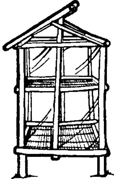
Fig. 24 Solar cabinet dryer, Indonesia
