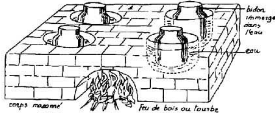
Figure 7 - Chaudière bain-marie
