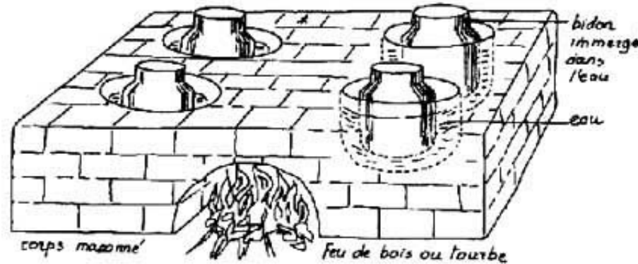
Figure 7 - Chaudière bain-marie
