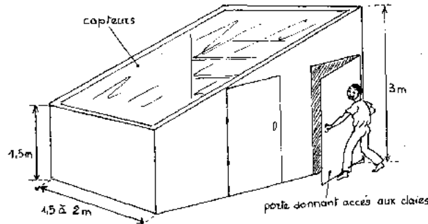
Figure 61: Séchoir case à convection forcée
