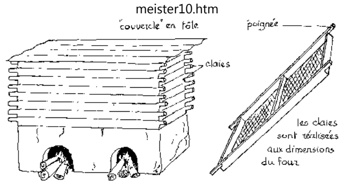
Figure 77: Four Chorkor chargé de claires
