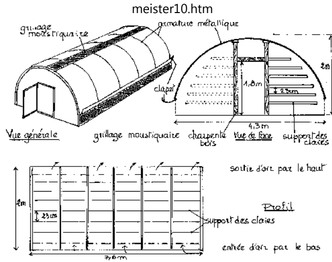
Figure 55: Tente cylindrique ♦ Aden
