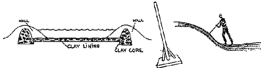
Figure 3.12 Lining and Compaction of Irrigation Pond (Ref. 7)
