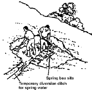
Figure 3.6 Excavating Spring Site (Ref. 39)
