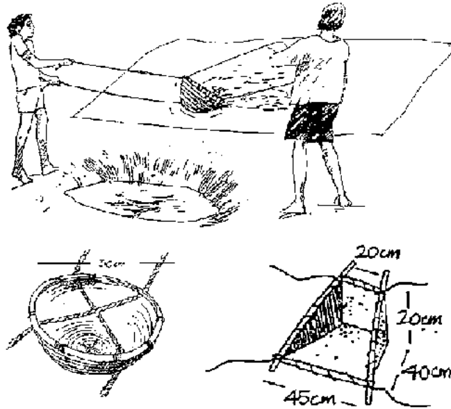
Figure 3.15 Swing Baskets (Ref. 28)
