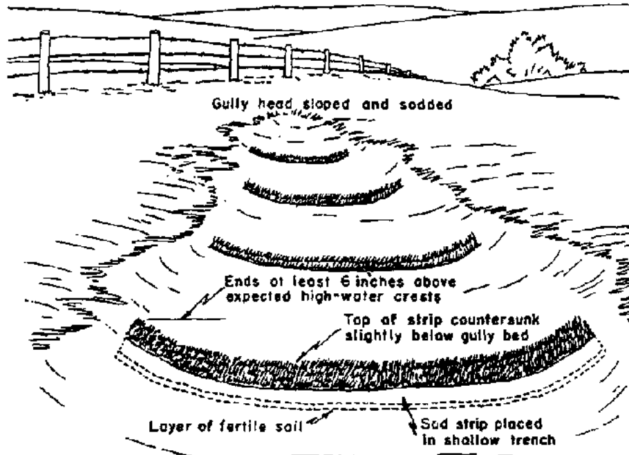
Figure 2.9 Sod Strip Checks on a Small Gully
