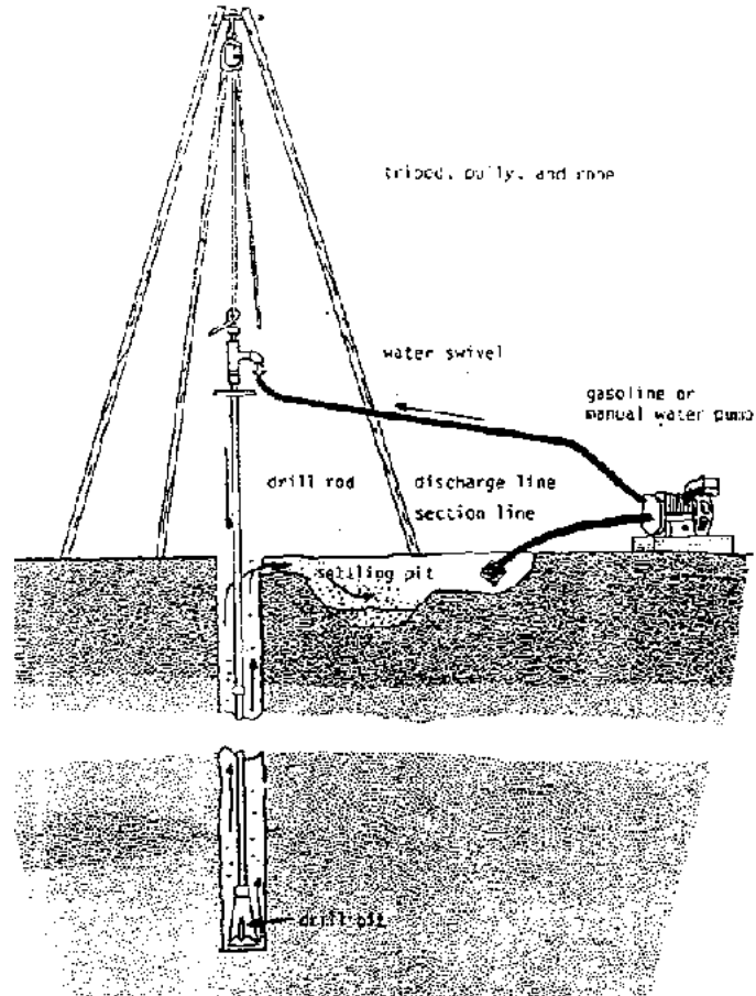
Figure 3.43 Manual Jetting Equipment (Ref. 15)
