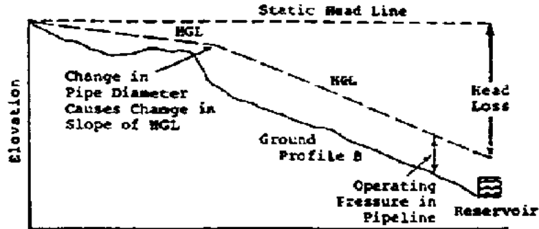
Figure 5.17 Hydraulic Gradient Line with Change in Pipe Diameter (Ref. 21)
