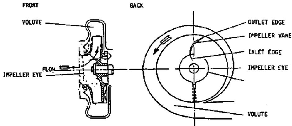
Figure 3.26 Components of a Centrifugal Pump (Ref. 20)
