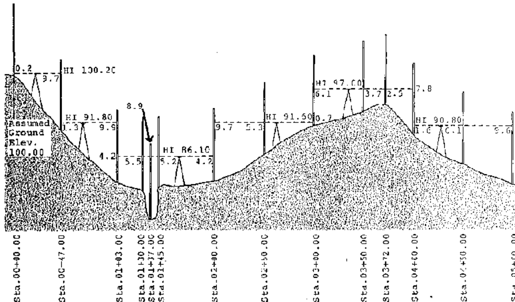
Figure 2.26 Typical Profile (Ref. 21)
