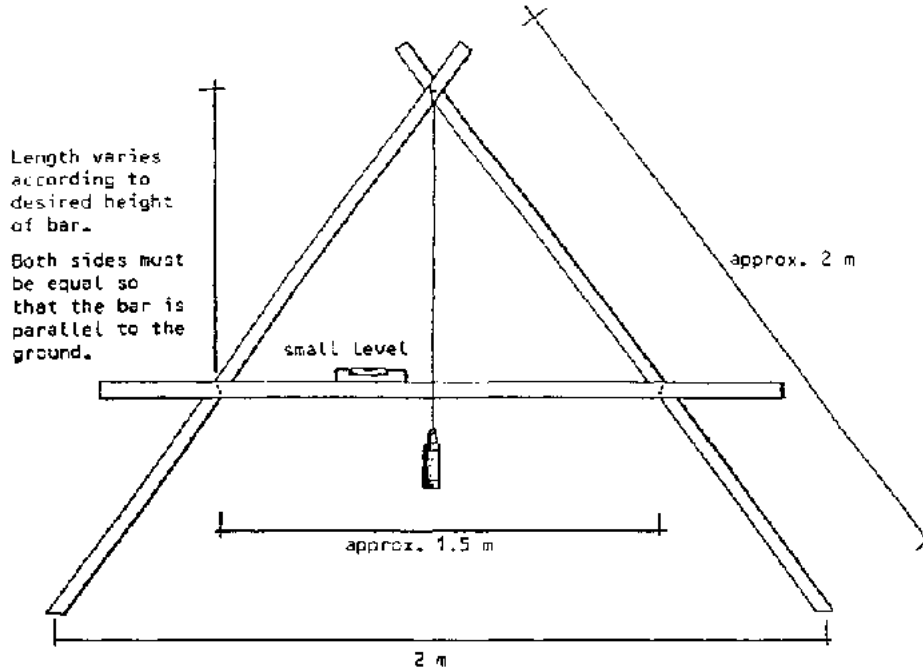
Figure 2.30 A-Frame Level for surveying Contour Lines (Ref. 9)
