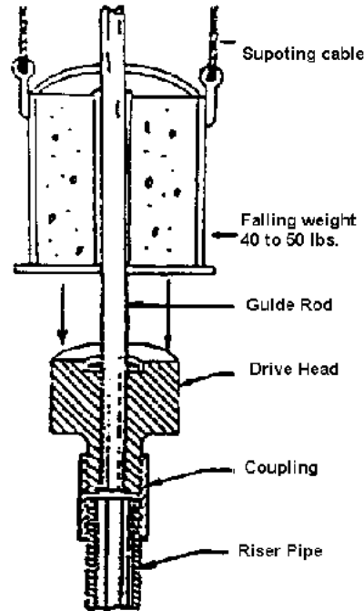
cross-section of sliding hammer and drive stem
