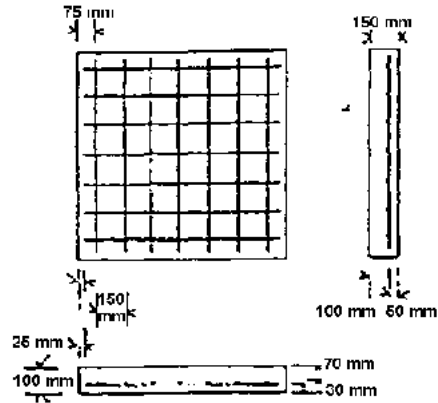
Figure 3.7 Placement of Rebar in Concrete Slab (Ref. 39)
