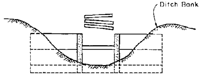
(a) Top-opening Gate with Removable Section Cover
