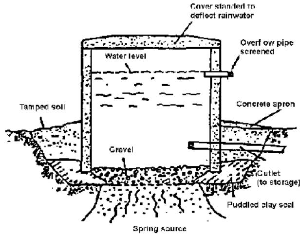
Figure 3.3 Spring Box with Open Bottom (Ref. 39)
