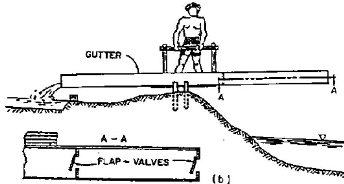
Figure 3.22 Gutters: (Ref. 58) (b) "See-Saw"
