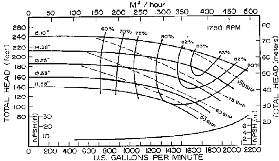
Figure 3.29 Pump Curve
