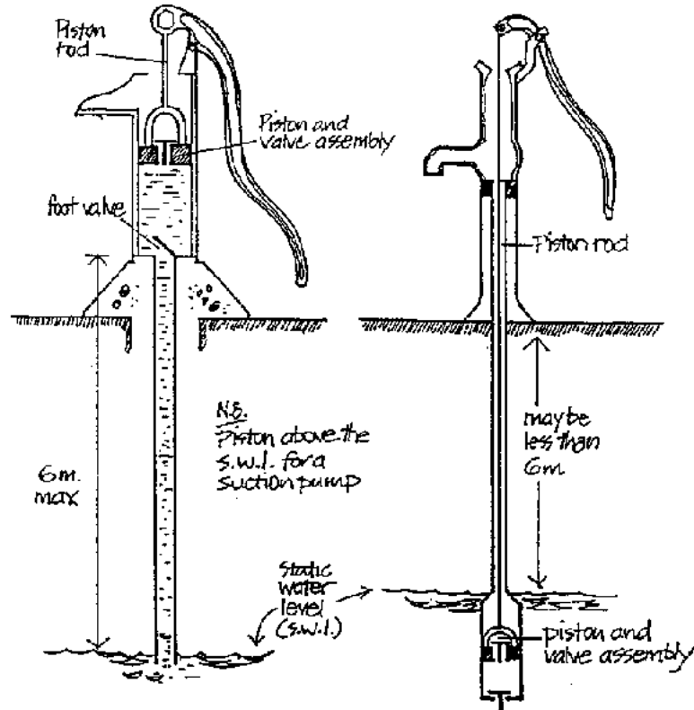
Figure 3.14 Hand (Piston) Pumps (Ref. 28)
