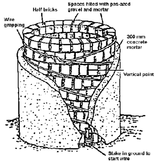
Figure 3.9 Brick Spring Box (Ref. 39)
