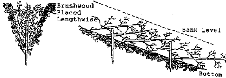
Figure 2.4 Plugging of Smaller Gullies (Ref. 56)
