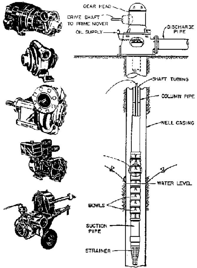
vertically-mounted, "turbine" pump.
