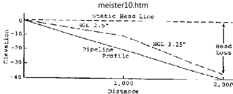
Figure 5.19 Example: Sketch for Pipeline 2 (Ref. 21)
