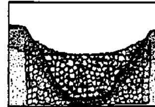
Figure 2.5 Construction of a Rock Check Dam
