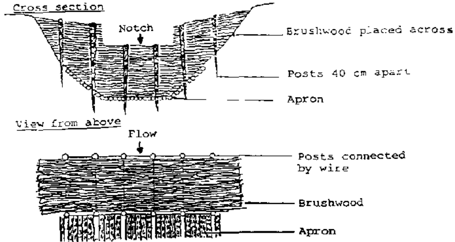
Figure 2.6 Brushwood Check Dam (Ref. 56)
