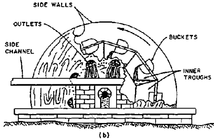
Figure 3.19 Modified Persian Wheel or Zawafa (Ref. 58) (b)
