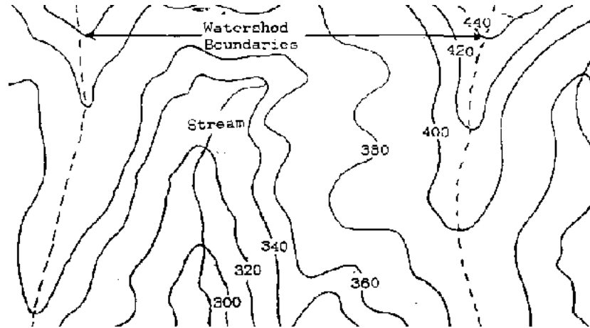
Figure 2.1 Watershed Boundaries on Contour Map
