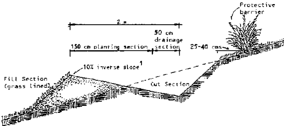
Figure 2.13 Discontinuous Narrow Terrace (cross section) (Ref. 9)
