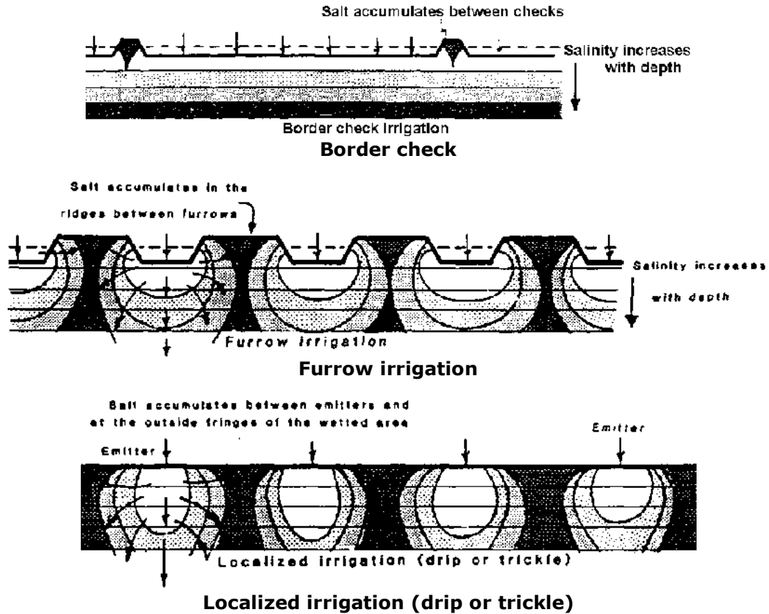
Figure 7.3 Bed Shapes and Salinity Effects (Ref. 1)
