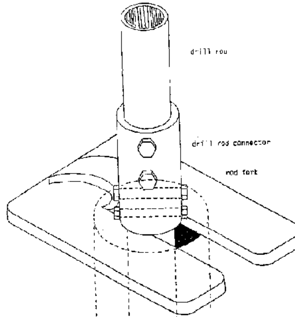
Figure 3.42 Rod or auger Fork Locally Fabricated From 1/4" (6 mm) Steel Plato (Ret. 15)
