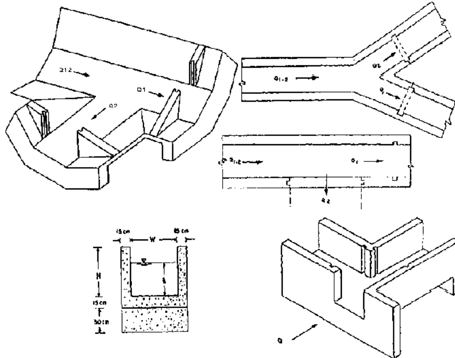
Figure 5.12 Flow Dividers
