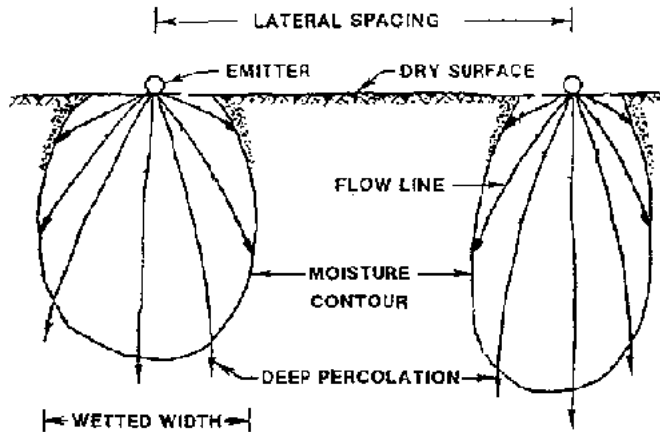
Figure 5.28 Typical Pattern of soil Wetting Under Trickle
