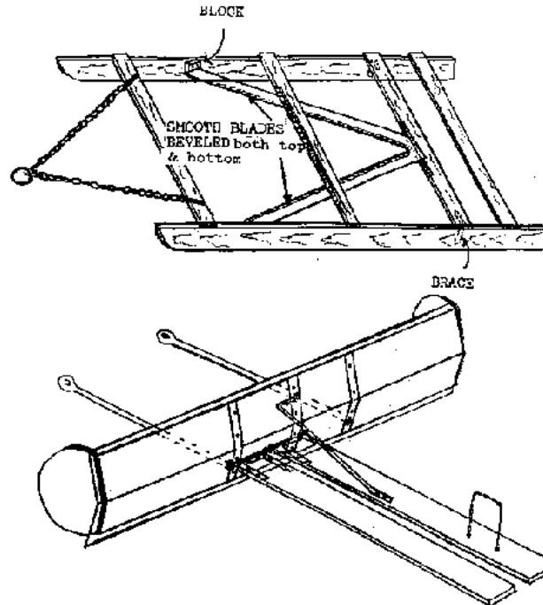
Figure 5.21 Land Smoother and Buckscraper
