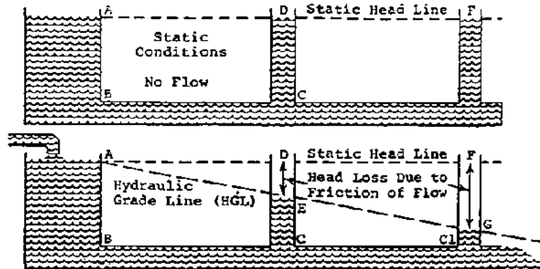
Figure 5.15 Hydraulic Gradient Line With and Without Flow (Ref. 21)
