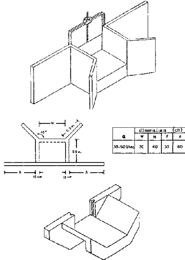
Figure 5.10 Wood, Single Well Check with Turnout (Ref. 41)
