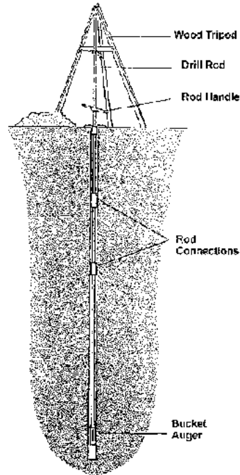
Figure 3.40 Hand Auger Drilling (Ref. 15)
