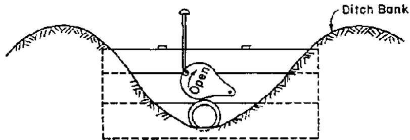
(c) Bottom-opening Gate with Swinging Cover
