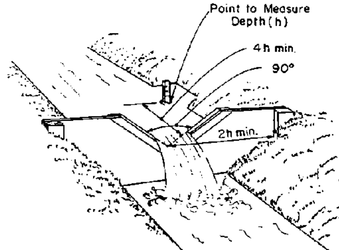
Figure 2.21 Ninety Degree V-Notch Weir (Ref. 41)
