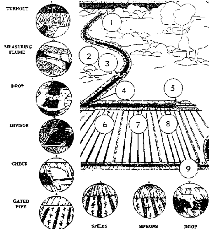
Figure 5.1 A Farm Irrigation System (Ref. 41)
