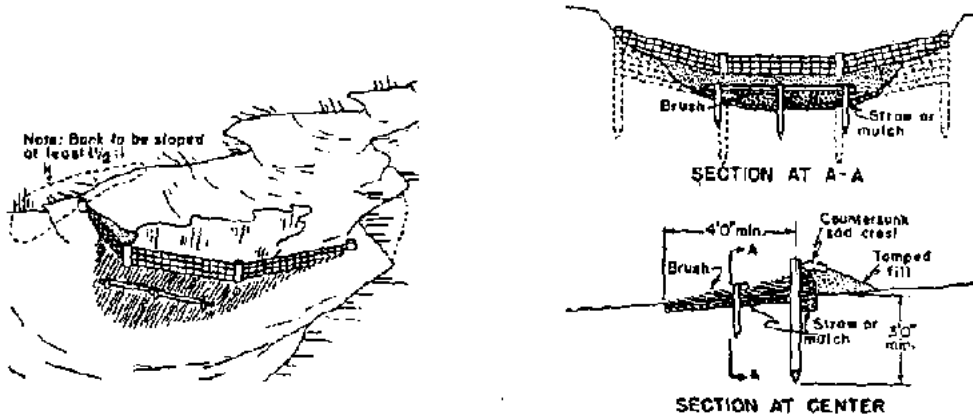
Figure 2.8 A Woven Wire Check Dam
