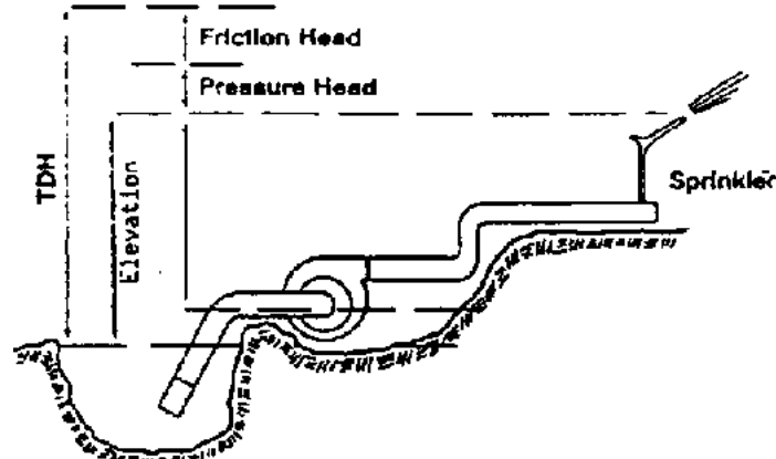
Figure 3.28 Diagram of a Centrifugal Pump Installation Showing Head and Lift Concepts
