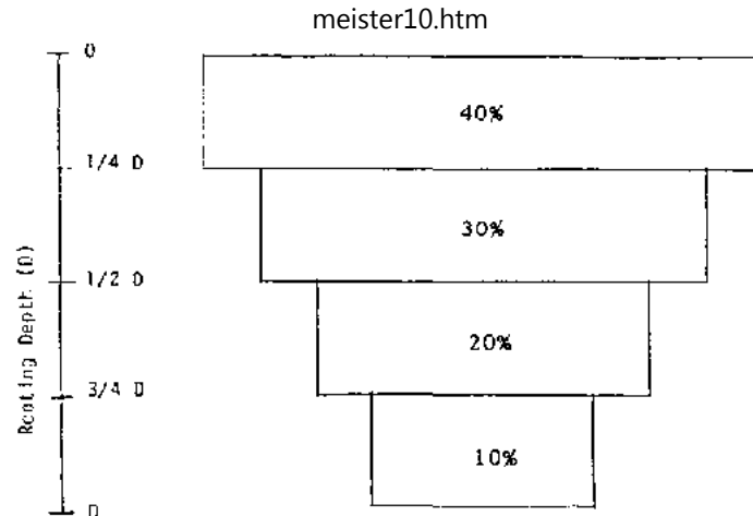
Figure 2.36 Typical Crop Water Extraction Patterns
