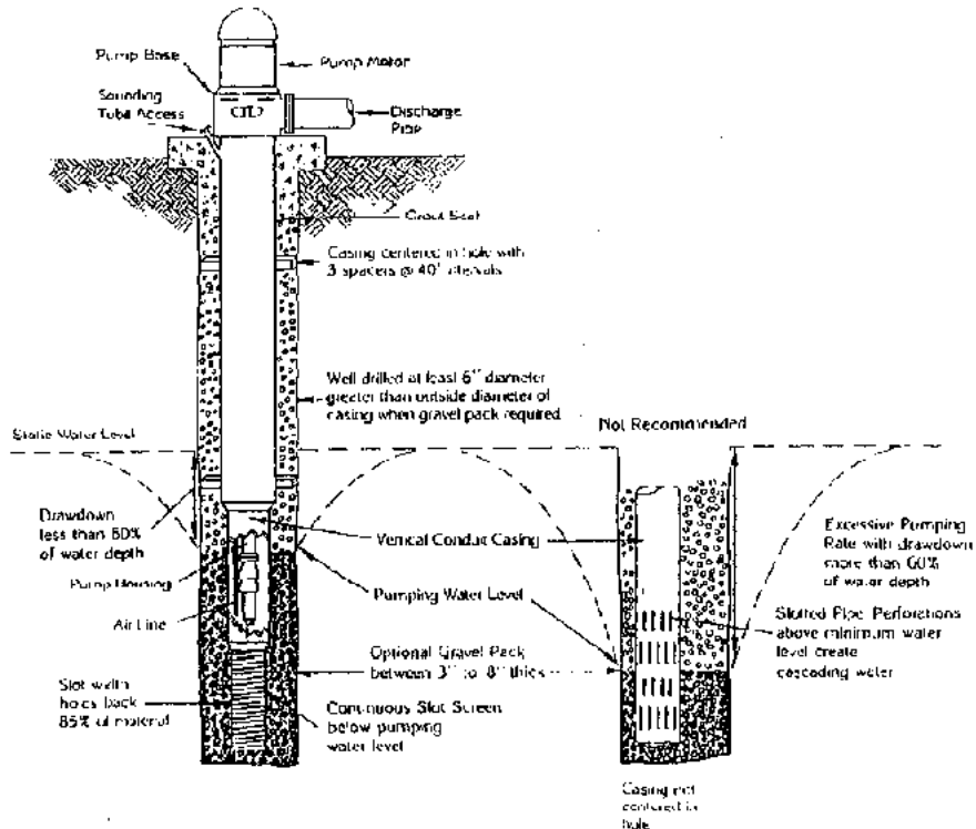
Figure 3.33 Recommended Pump Installation (Turbine) (Ref. 54)
