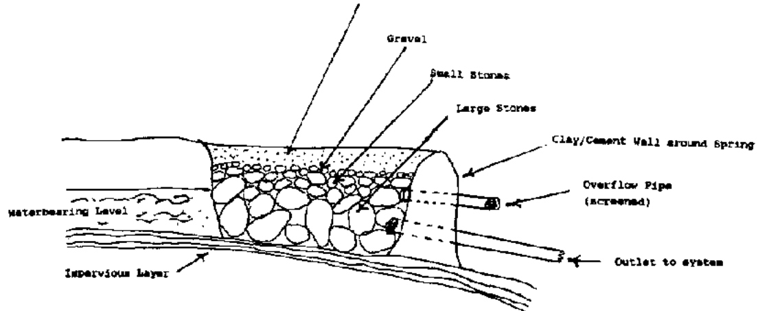
Figure 3.1 Spring Box Design
