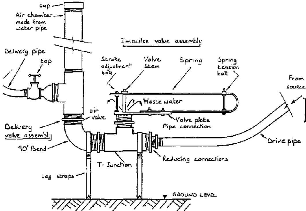
Figure 3. 37 Hydraulic Ram (Ref. 55)
