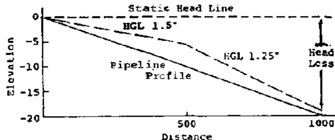
Figure 5.18 Example: Sketch for Pipeline 1 (Ref. 21)
