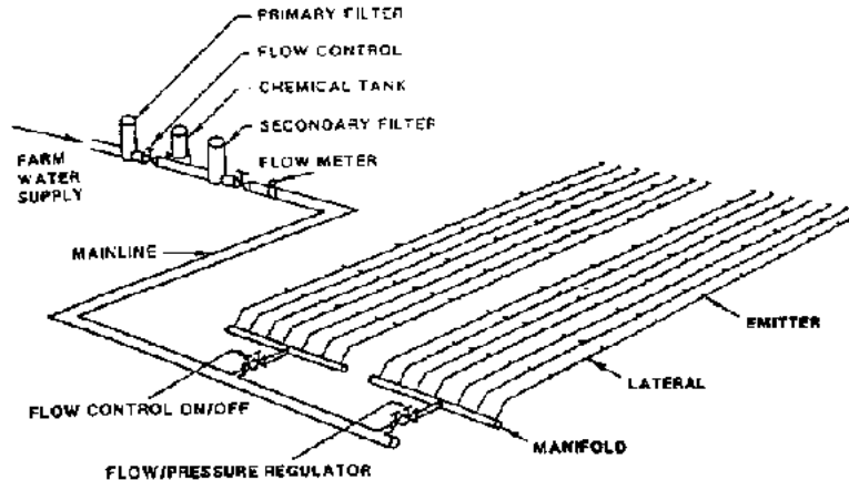
Figure 5.27 Basic Components of a Localized Irrigation System
