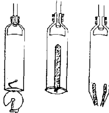
Figure 3.41 Typical Hand Augers and Equipment (Ref. 15) (a) Sand Augers for Non-Cohesive Soils
