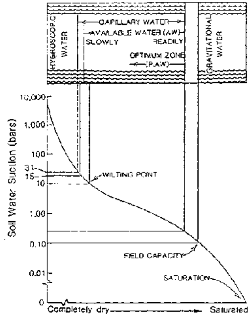
Figure 2.33 Soil Water and its Availability
