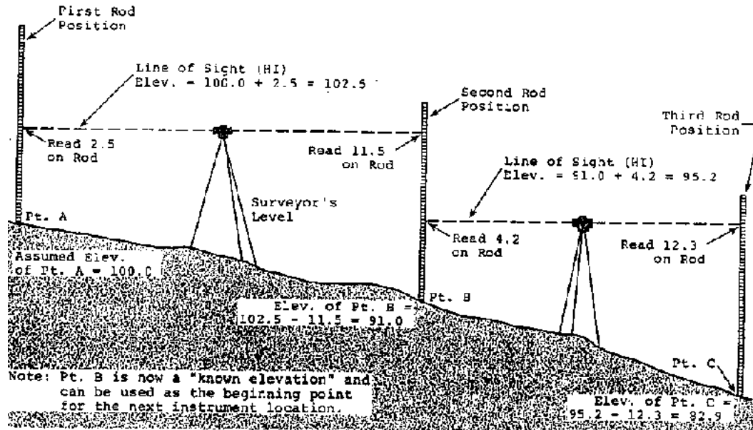
Figure 2.25 Profiling: Example (Ref. 21)
