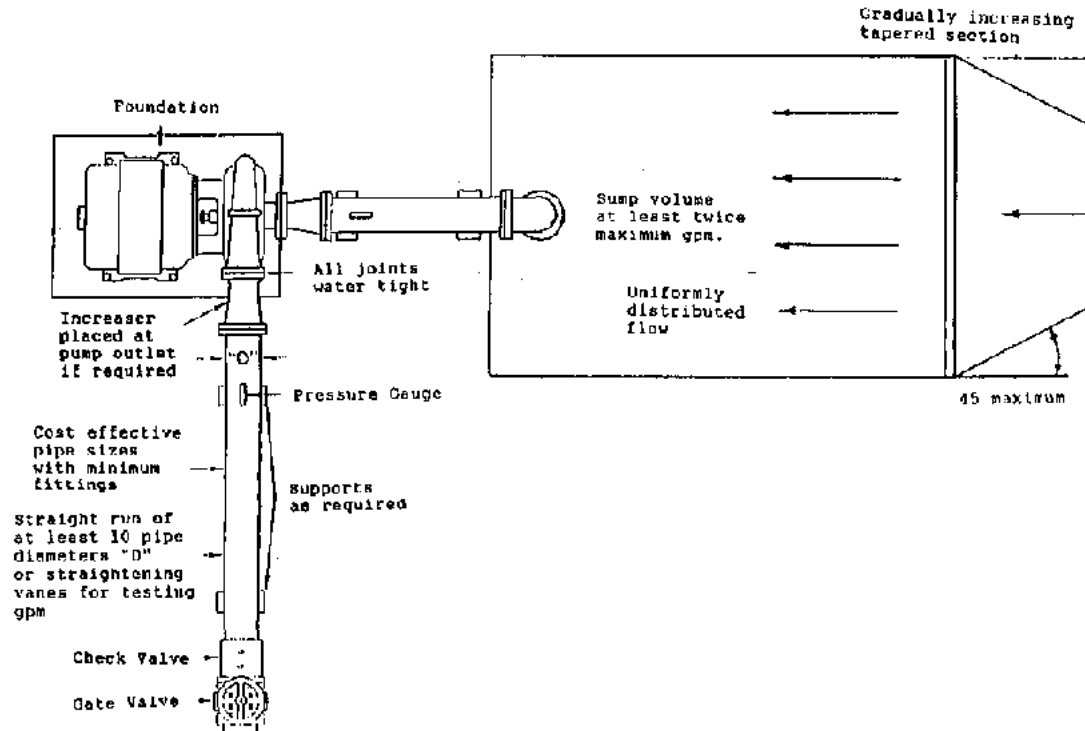
Figure 3.32 Recommended Pump Installation - Top View (Ref. 54)
