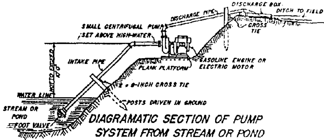
DIAGRAMMATIC SECTION OF PUMP SYSTEM FROM STREAM OR POND
