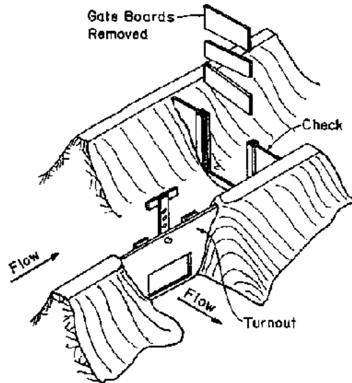
Figure 5.9 Small Concrete Ditch Check (Ref. 41)
