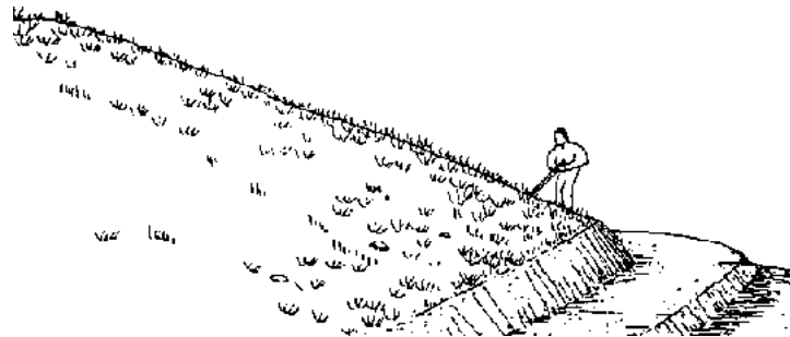
Figure 2.16 Bench Terrace Construction Sequence "A" (Ref. 9)
