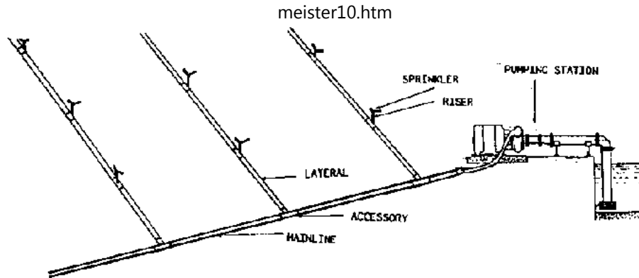
Figure 5.24 Typical Sprinkler Irrigation System Components
