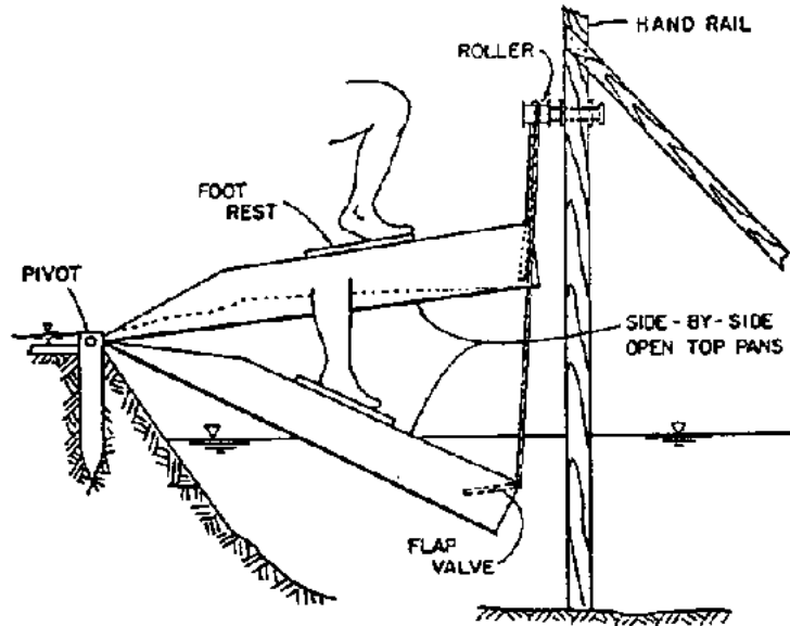
Figure 3.23 Modifications of the Doon (Ref. 58) (b)
