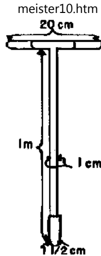
An auger-type soil sampler
