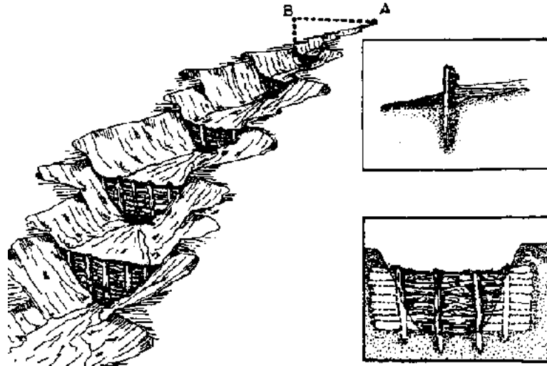
Figure 2.7 Pole or Log Check Dam
