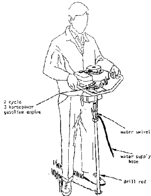
Figure 3.44 Hydra-Drill (Ref. 15)
