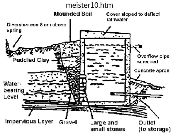
Figure 3.2 Spring Box with Open Sides (Ref. 39)
