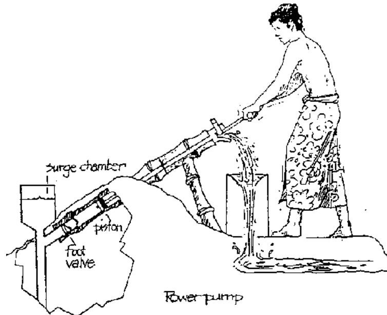
Figure 3.25 Rower Pump (Ref. 28)
