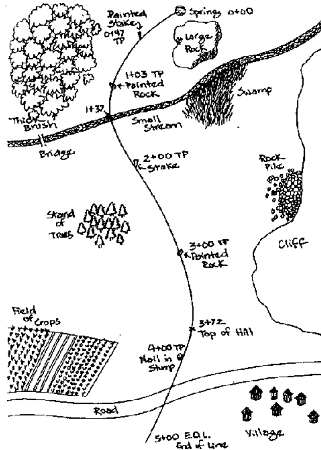
Figure 2.27 Survey Sketch and Notations (Ref. 21)
