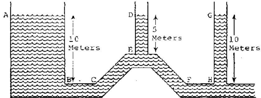
Figure 5.14 Head on System with No Flow (Ref. 21)
