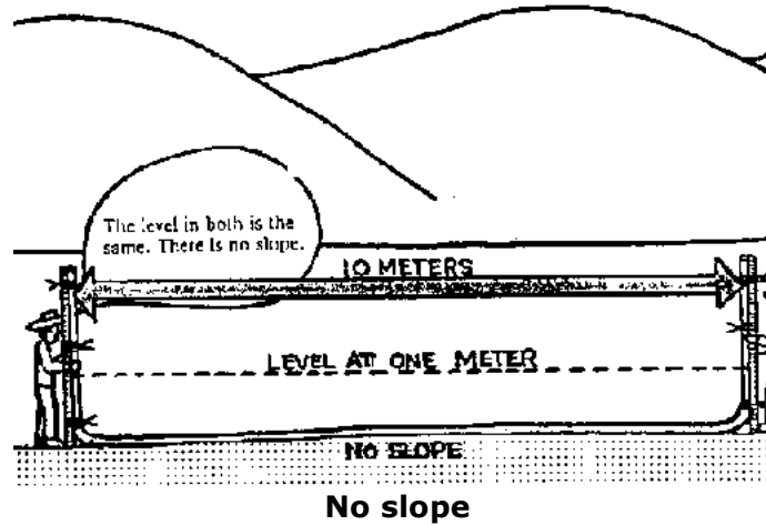
Figure 2.32 Use of a Hose Level (Ref. 42)
