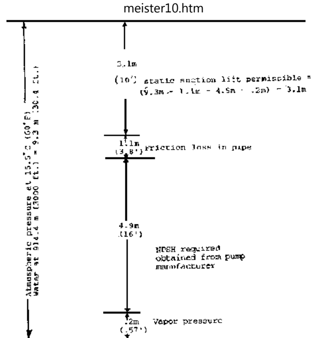
Figure 3.30 Graphical Solution of NPSH (Ref. 20)
