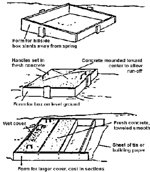
Figure 3.8 Forms for spring Box Cover (Ref. 39)
