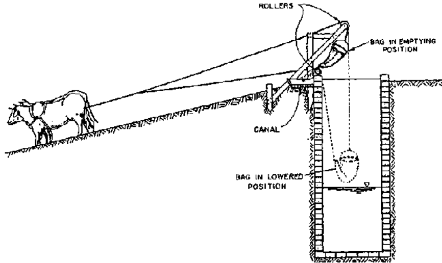
Figure 3.24 Self- Emptying Not with Inclined Tow Path (Ref. 58)
