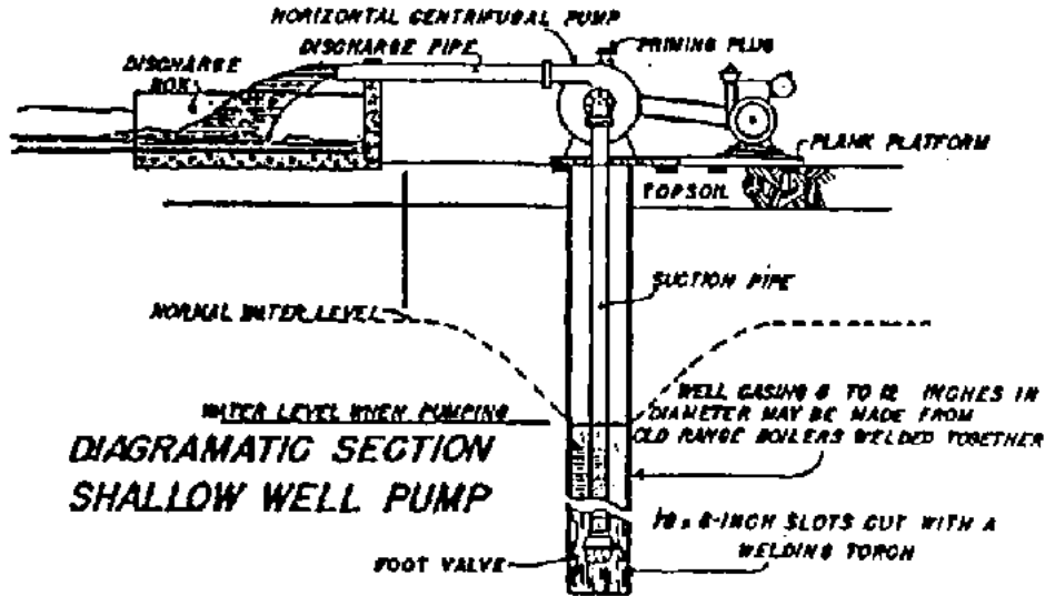
DIAGRAMMATIC SECTION SHALLOW WELL PUMP
