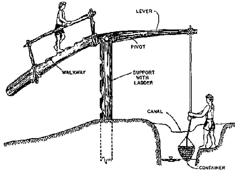
Figure 3.20 Picottah, Using Man as Moveable Counterweight
