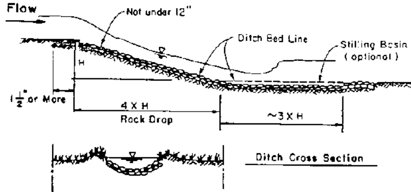
Figure 5.6 Sloping Rock Drop Structure (Ref. 41)
