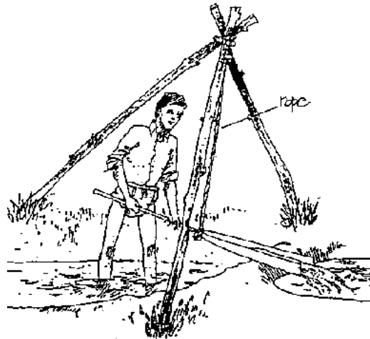
Figure 3.17 Suspended Scoops (Ref. 28)
