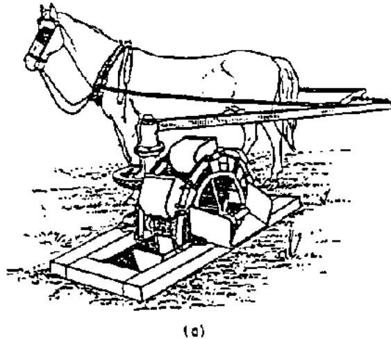
Figure 3.19 Modified Persian Wheel or Zawafa (Ref. 58) (a)
