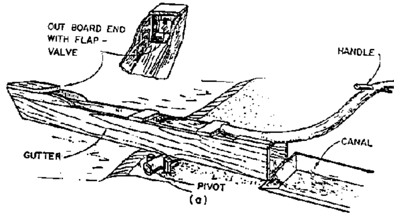
Figure 3.22 Gutters: (Ref. 58) (a) Single with Handle
