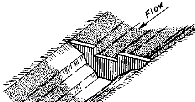
Figure 5.9 Small Concrete Ditch Check (Ref. 41)
