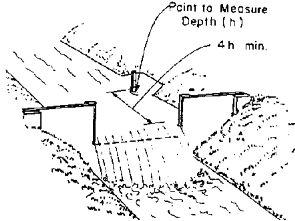
Figure 2.20 Rectangular Weir Used as Measuring Device and Drop
