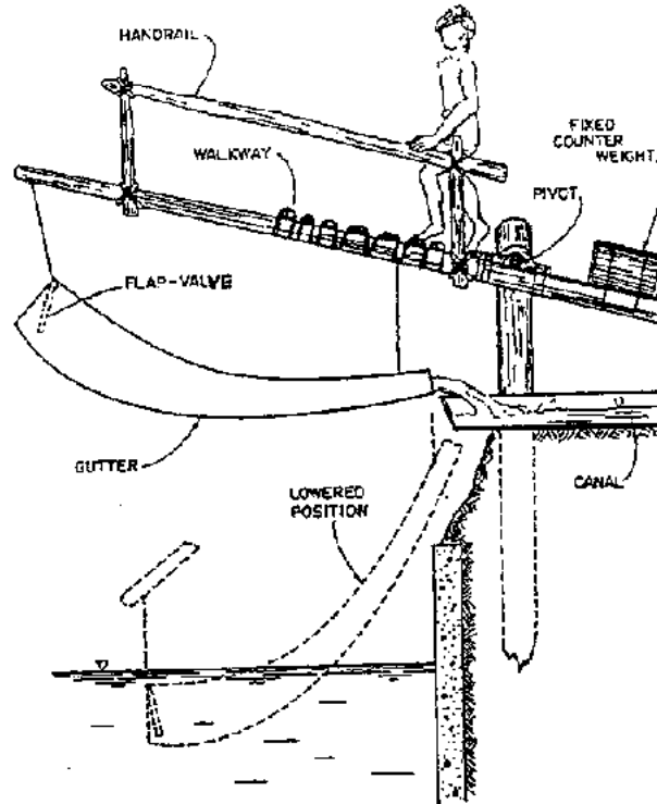
Figure 3.21 Picottah style Doon with Flap Valve (Ref. 58)
