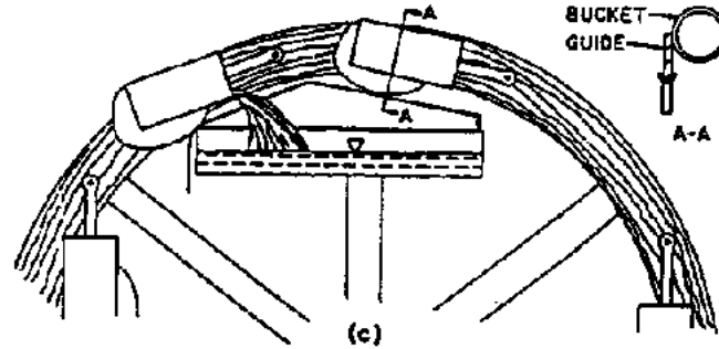
Figure 3.18 Noria: (Ref. 58) (c) With Moveable Buckets
