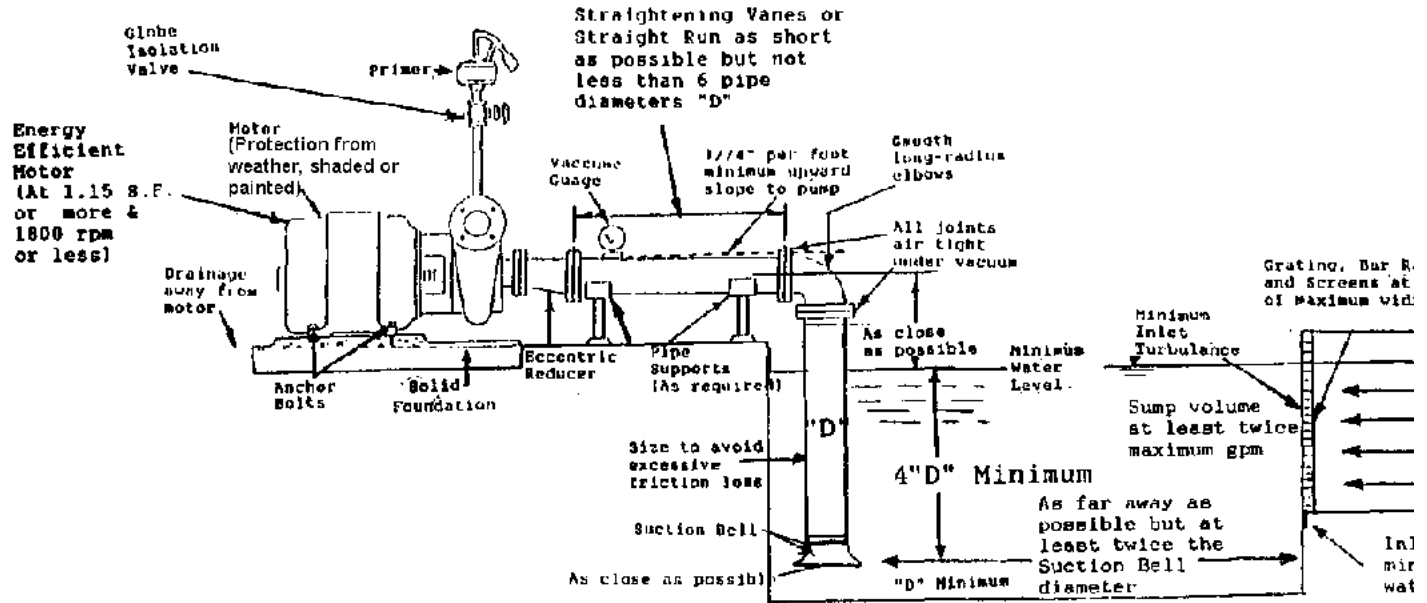
Figure 3.31 Recommended Pump Installation - Side View (Ref. 54)
