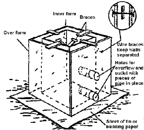
Figure 3.5 Forms for spring Box with Open Bottom (Ref. 39)
