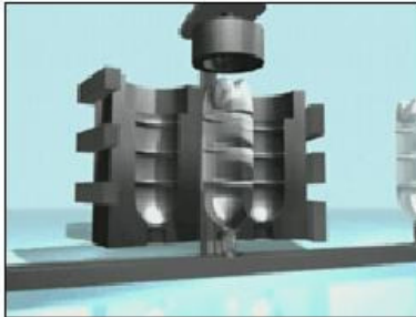
Fig : 9: Stretch forming
