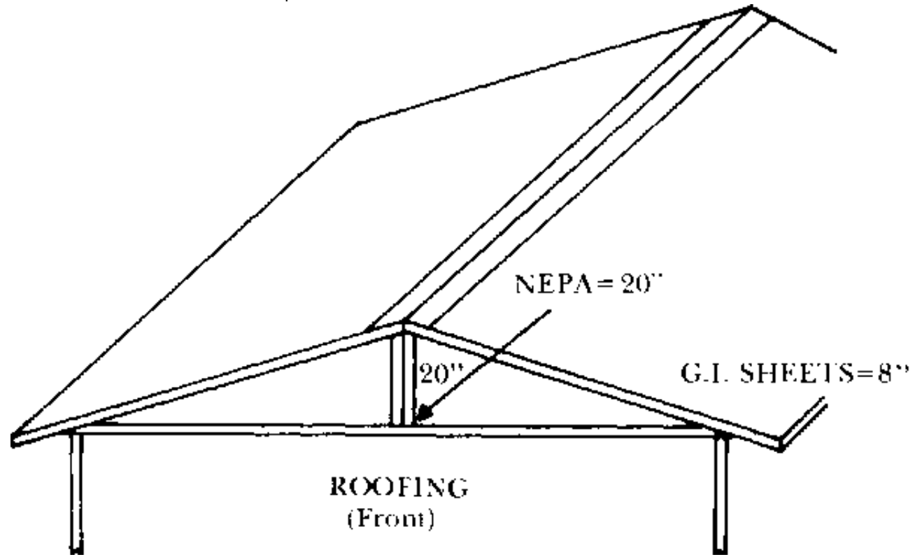
B: WOOD FRAME AND WIRE HUTCH - DOUBLE FACE
