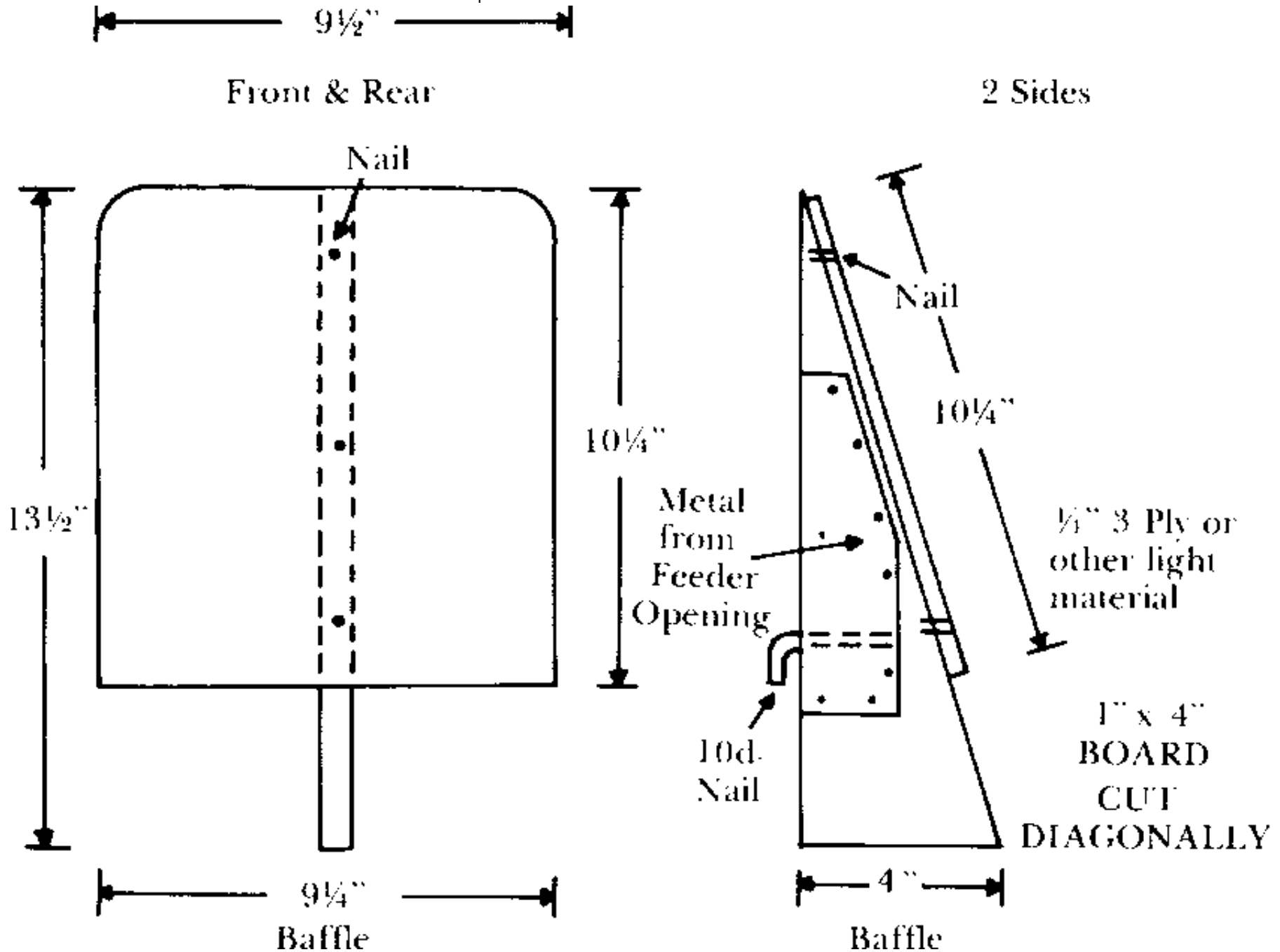
FIGURE 10 - DESIGNS FOR FEED HOPPER MADE FROM 5-GALLON CAN
