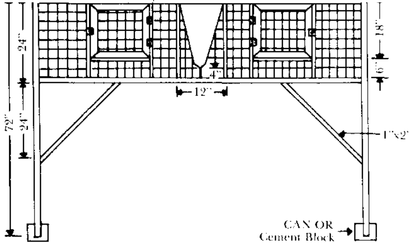
FRONT-REAR VIEW A: WOOD FRAME AND WIRE HUTCH - DOUBLE FACE
