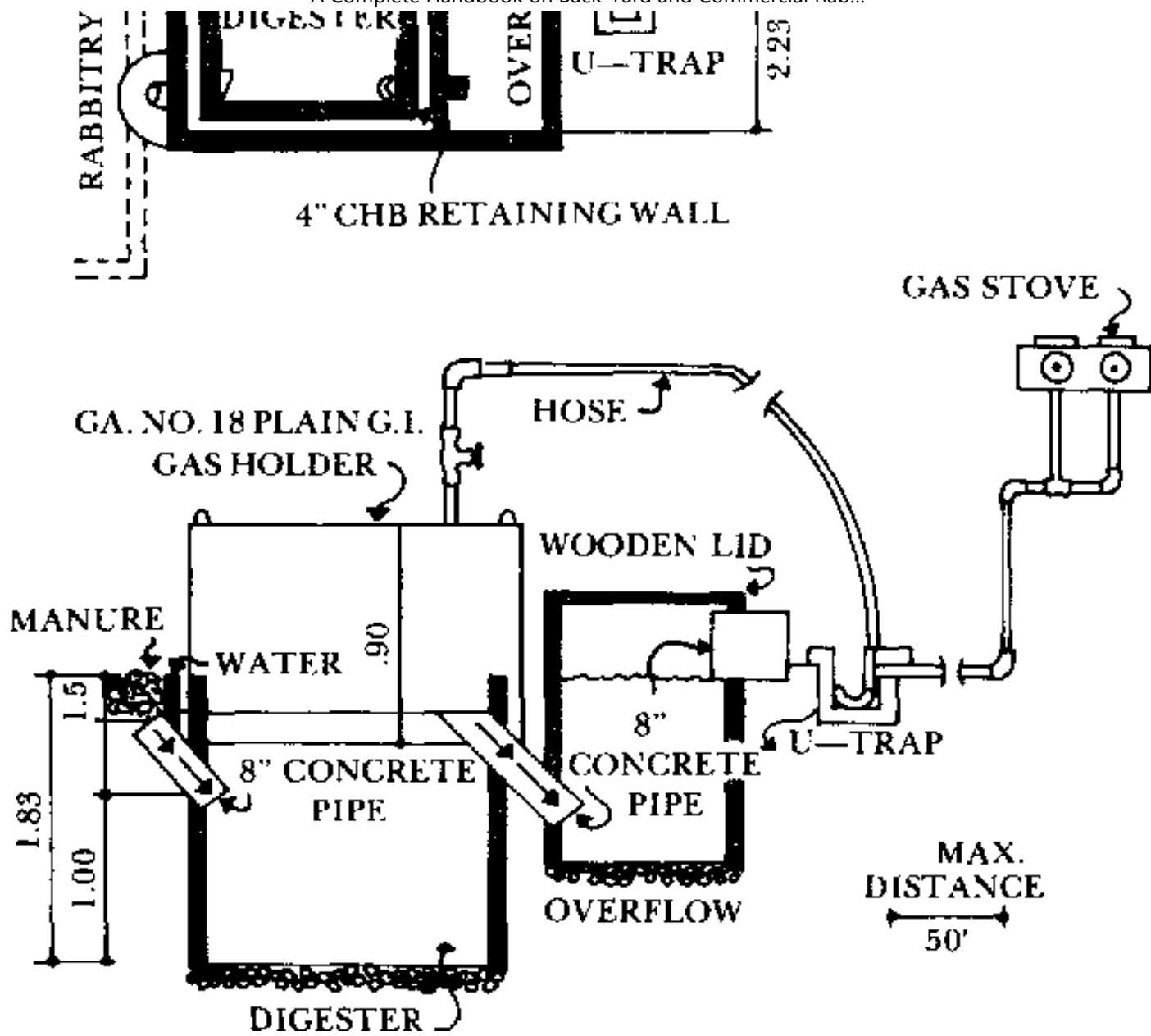
FIGURE 27 - Layout plan of a methane gas generator
