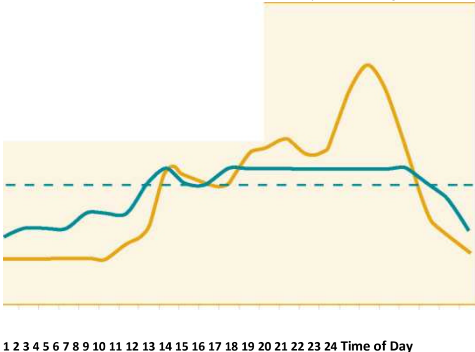
Figure 8. Load variation and effect of load management. Adapted from Micro-Hydro Power:
