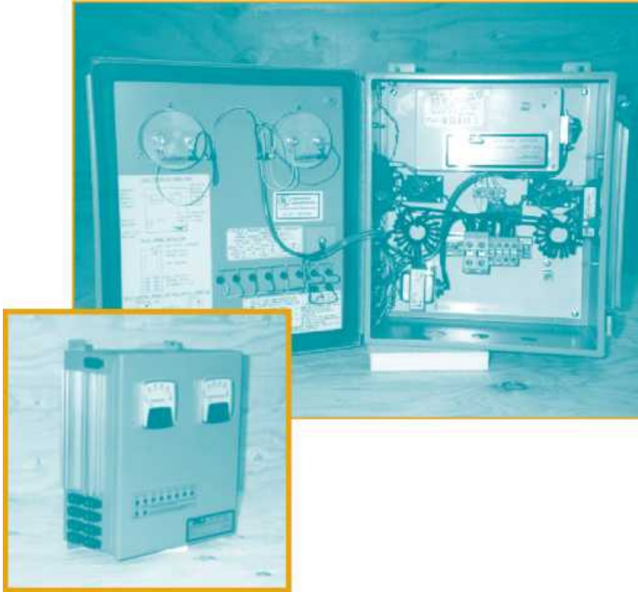
Figure 21. Electronic load controller, 12-kW-rated, front and inside view (photo courtesy of
