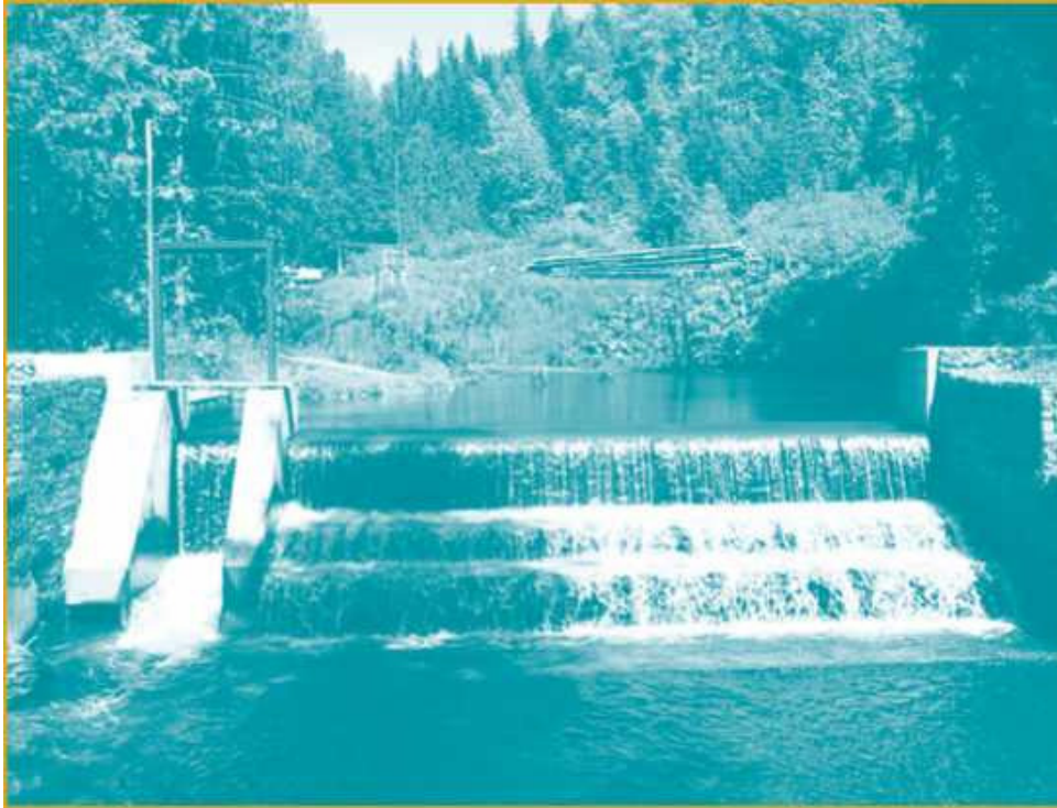
Figure 10. Intake of micro-hydropower system in Seaton Creek, British Columbia (photo courtesy of Homestead Hydro Systems)
