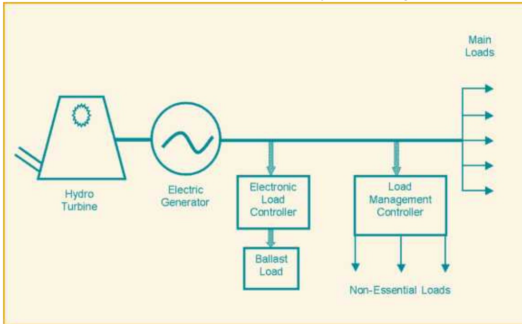
Figure 9. Basic set-up of load-management controller in a micro-hydropower system
