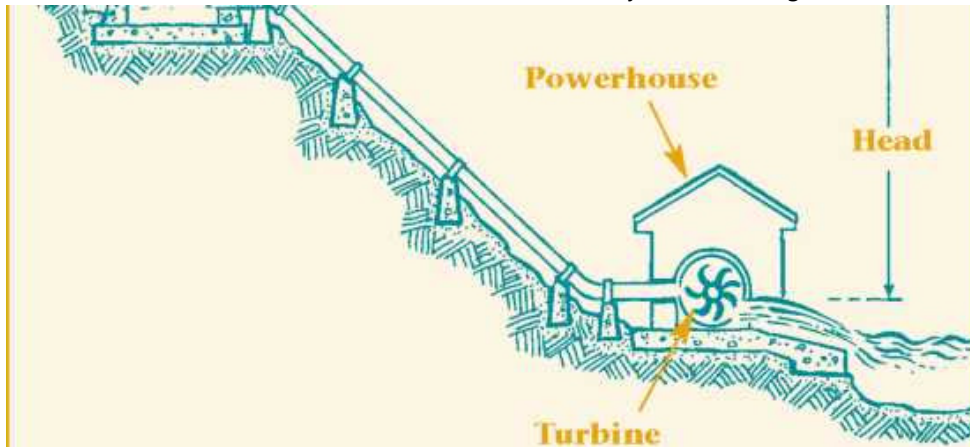
Figure 5. Head of a micro-hydropower system
