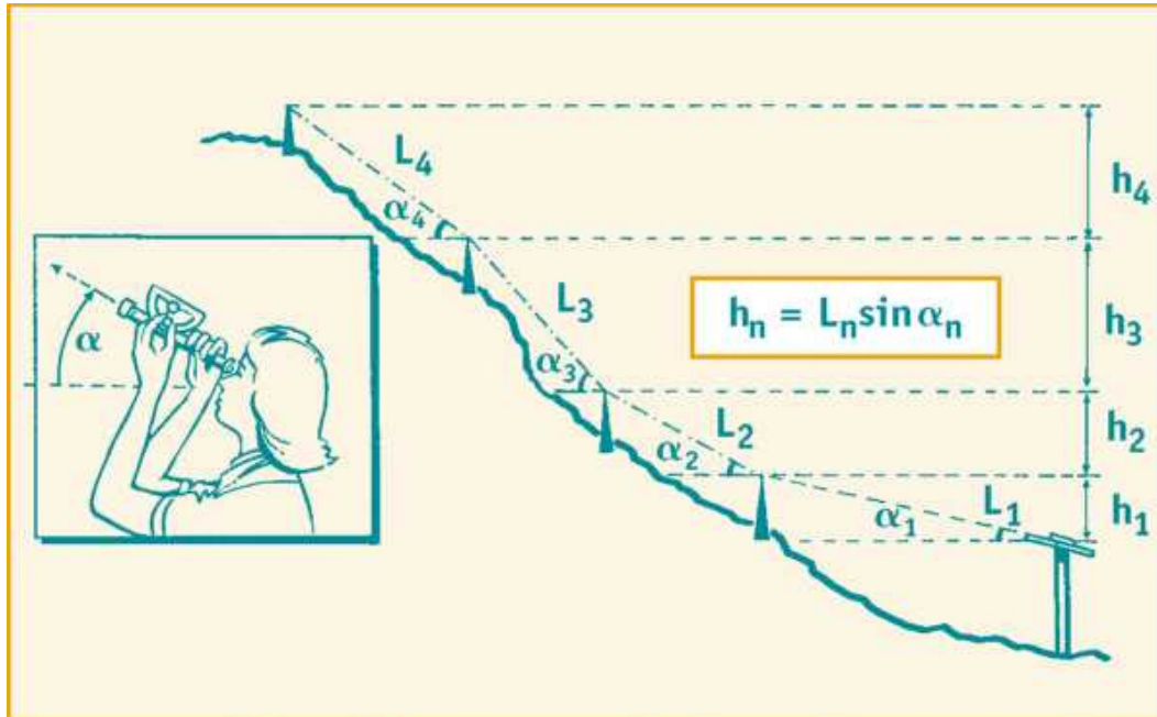
Figure 33. Measuring head using Abney-level method
