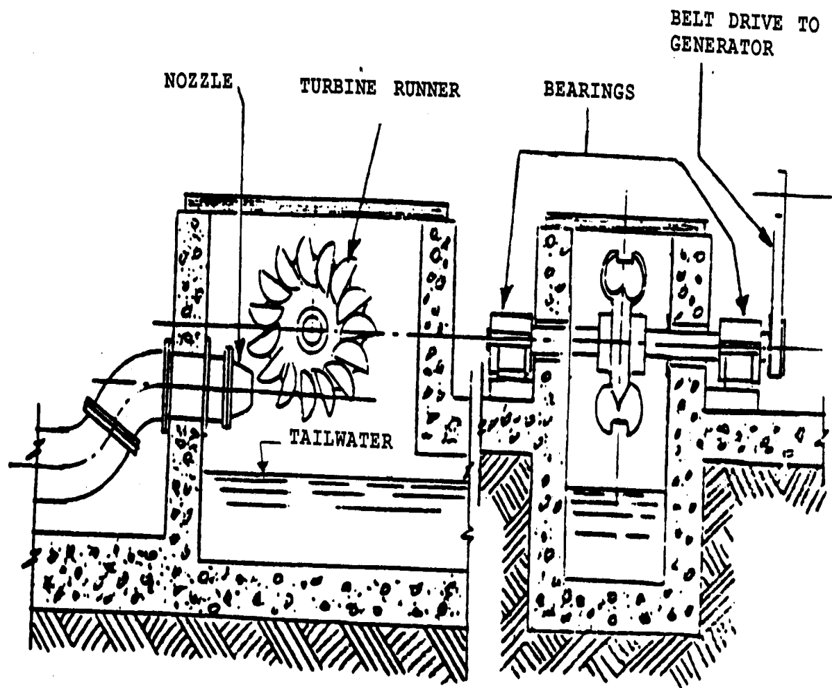
Figure 23. Small Impulse Turbine in Concrete Housing
