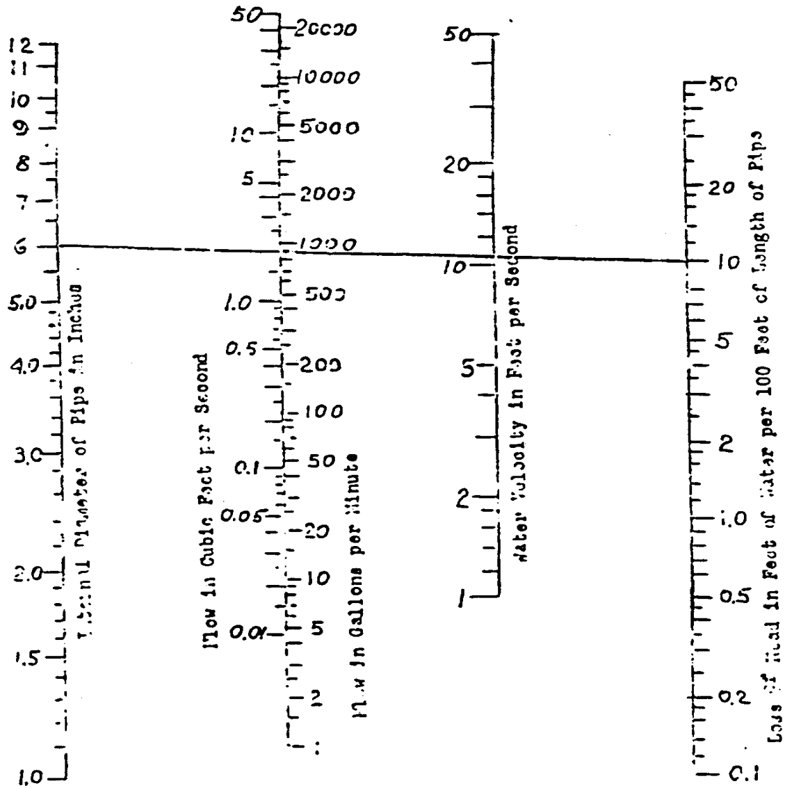
Figure 14. Nomograph for head loss in steel pipes
