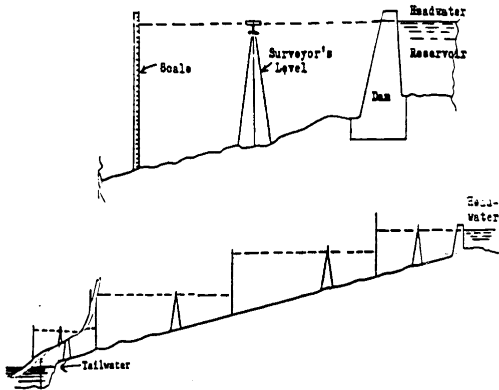
Figure 1. Measuring head with surveyor's level (Total Gross Head = A + B + C + D)
