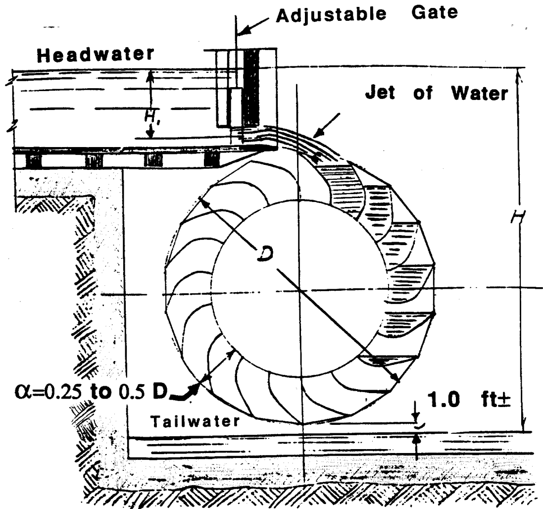
Figure 31. Overshot Water Wheel
