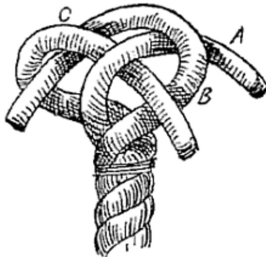
FIG. III.—Single crown (making).
