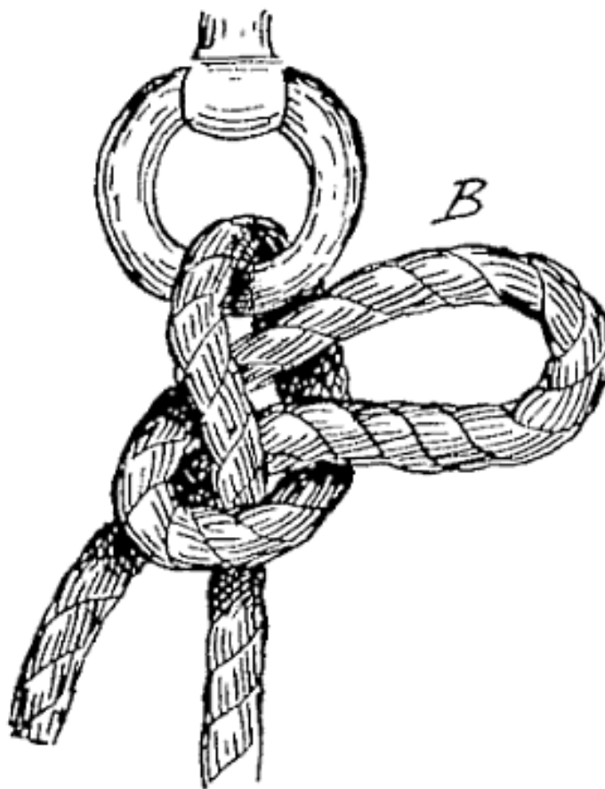
FIG. 32.—Slippery hitch (complete).
