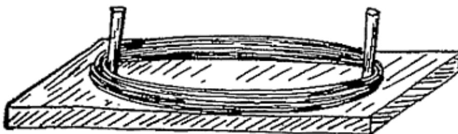
FIG. 88.—Selvagee board.
