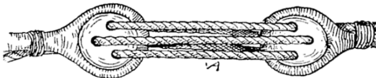
FIG. 98.—Deadeye lashing.
