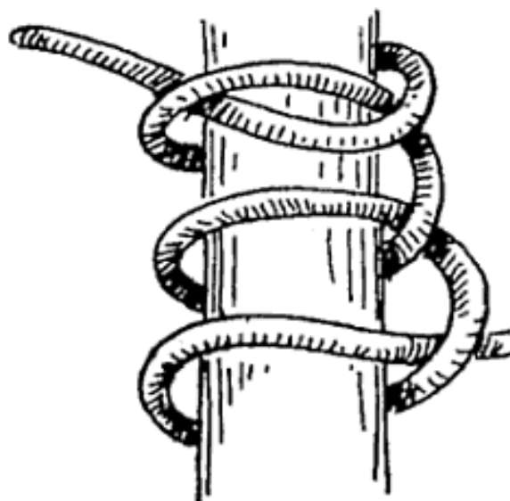
FIG. 139.—Half-hitch work.
