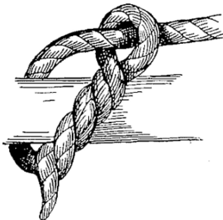
FIG. 38.—Timber hitch.
