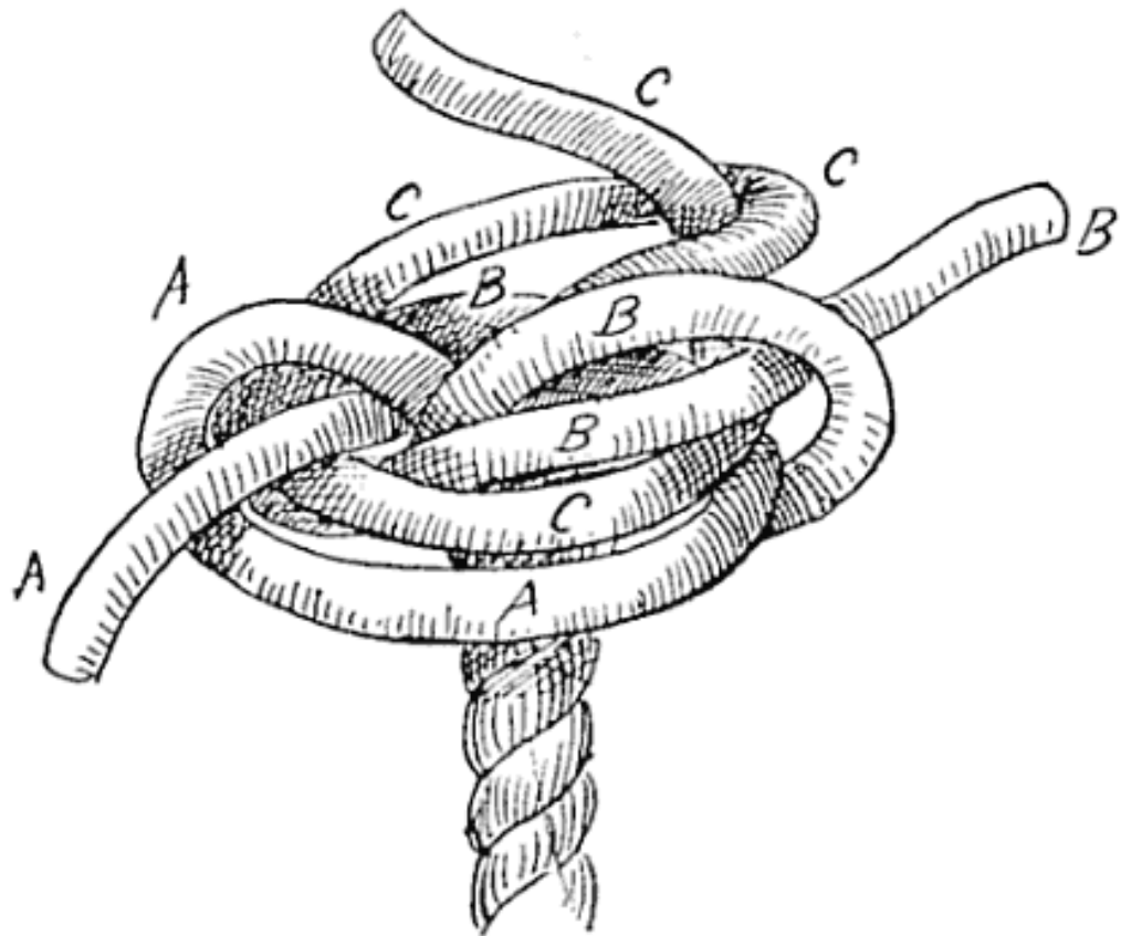
FIG. 132.—Matthew Walker (complete but slack).
