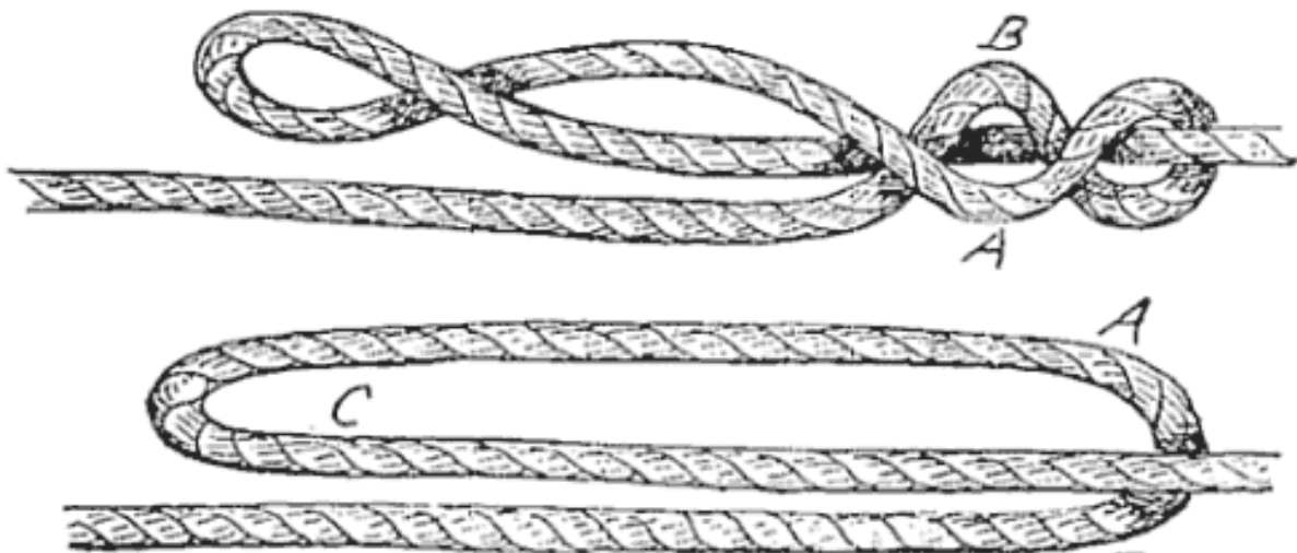
FIG. 71.—Twist braid (making). B
