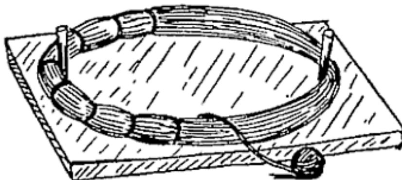
FIG. 89.—Seizing a selvagee strap.
