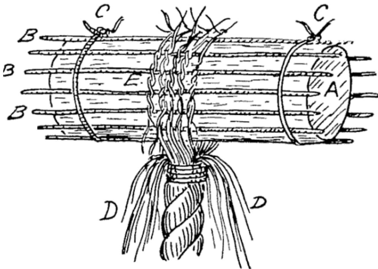
FIG. 90 A.—Making Flemish eye.
