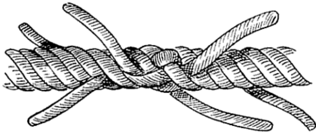
FIG. 106 D .—Short splice (continued).
