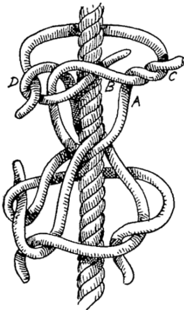
FIG. 119.—French shroud knot (making).
