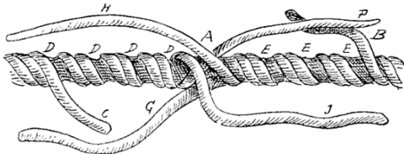
FIG. 107.—Long splice.
