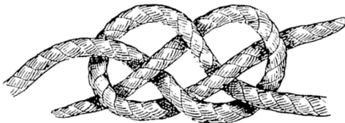
FIG. 27.—Garrick bend (tying).
