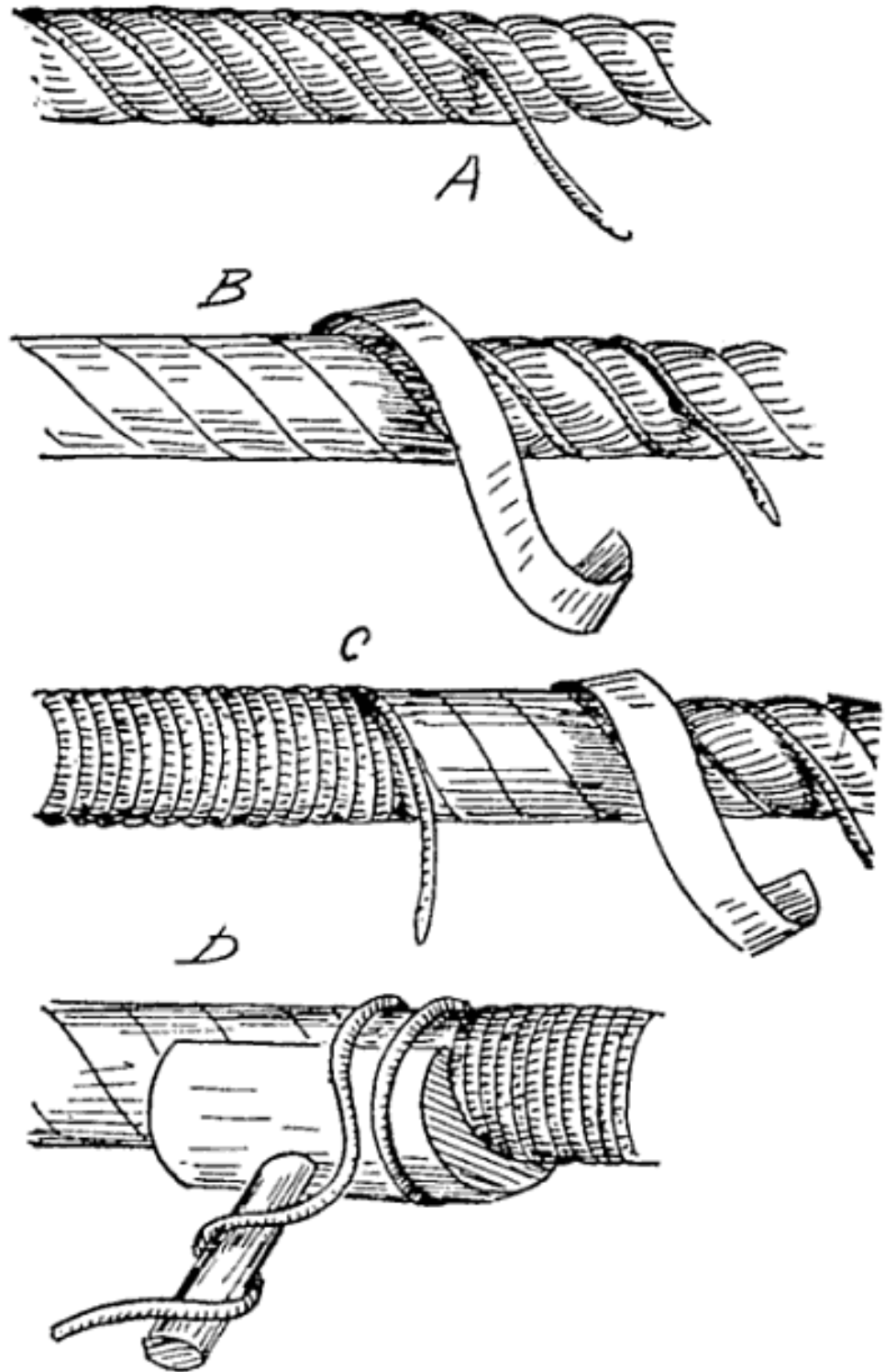
FIG. 138.—Worming, parcelling, and serving.
