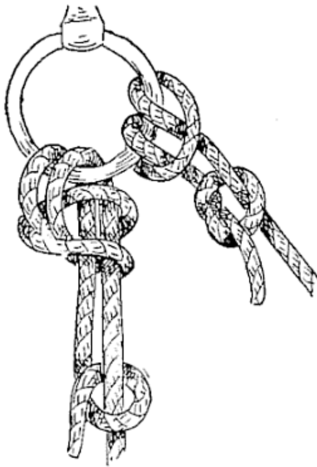
FIG. 56.—Larks' heads and running noose.
