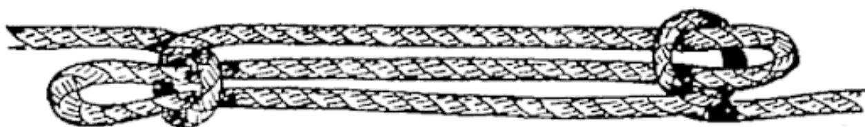
FIG. 79.—Another sheepshank.
