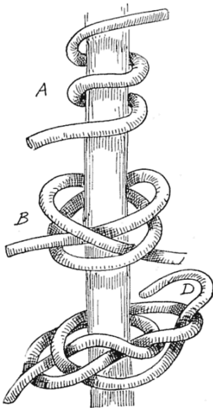
FIG. 135.—Making Turk's head.
