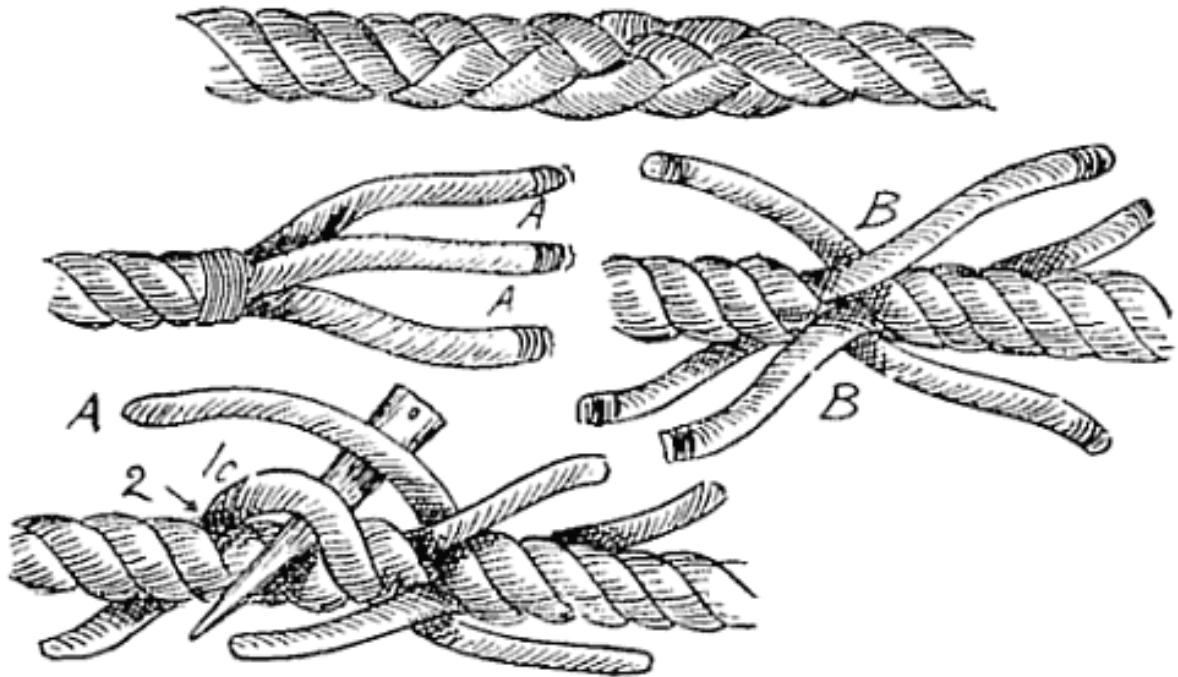
FIG. 106.—Short splice.
