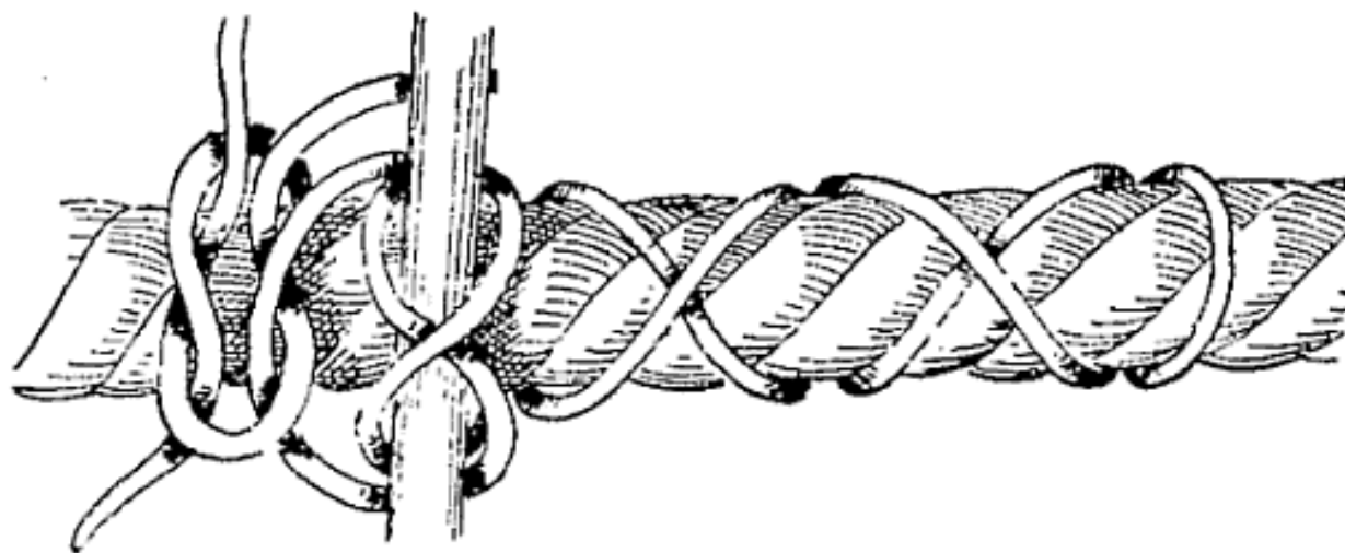
FIG. 47.—Chain hitch with bar.
