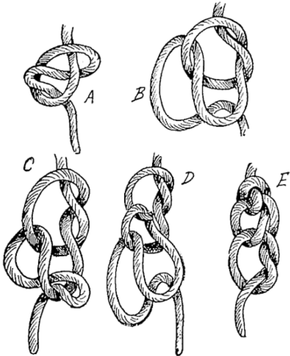
FIG. 70.—Single plait or monkey chain (making).
