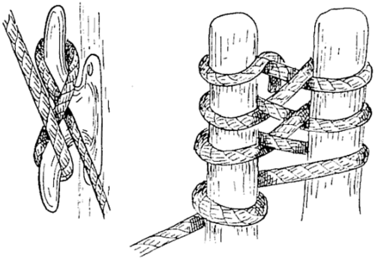
FIG. 57.—Cleat and wharf ties.
