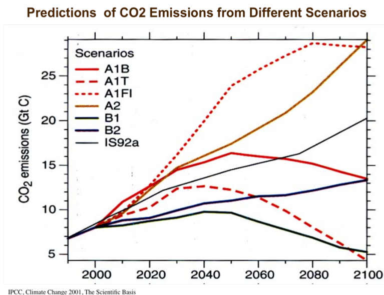
Figure 5.2: The development of carbon emission scenarios over the next century.
