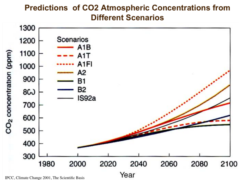
Figure 5.3: Values over the next century of predicted atmospheric concentrations of carbon dioxide.
