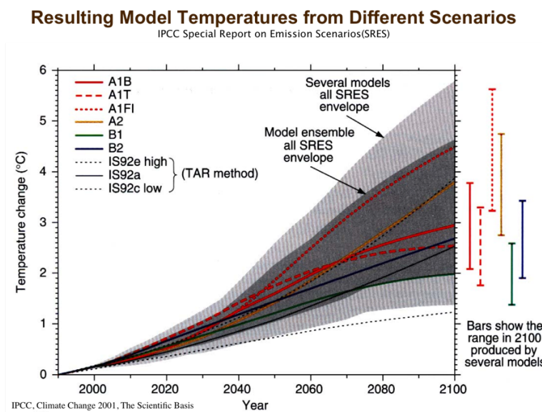
Figure 5.4: Modeled global temperature values for the standard IPCC fossil fuel scenarios.
