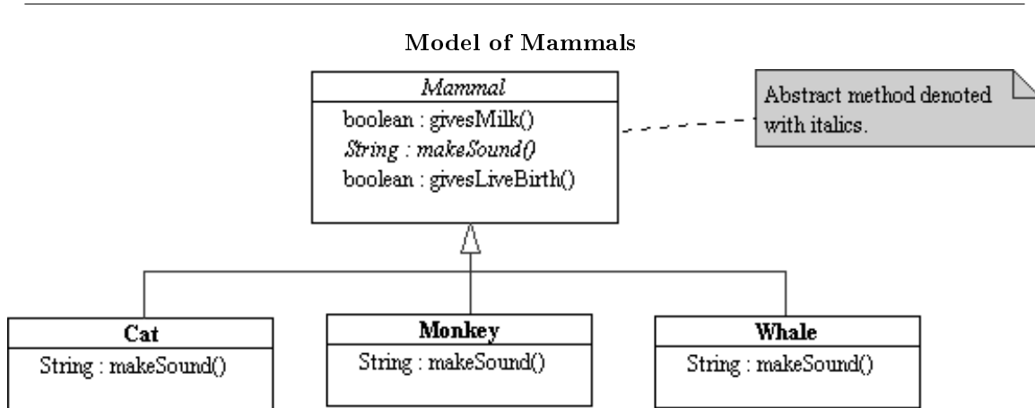
Figure 2.3: Abstract and common methods hoisted to the superclass.
