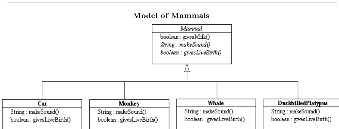
Figure 2.4: Properly abstracted model.
