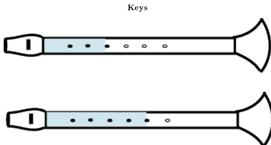
Figure 2.3: In general, the more holes that are closed with a key or covered by a finger, the longer the standing wave inside the instrument, and the lower the pitch.
