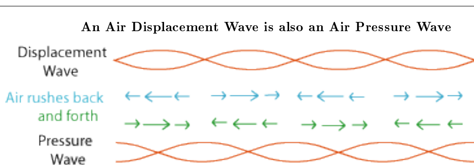
Figure 1.9: The nodes of the displacement wave, where the air is not rushing back-and-forth but is doing the most piling-up-and-spreading-out, are the antinodes of the pressure wave. The antinodes of the displacement wave, where the air is rushing back-and-forth the most, but is not piling up or spreading out at all, are the nodes of the pressure wave. Both waves must have exactly the same frequency, of course; they are actually just two aspects of the same sound wave.
