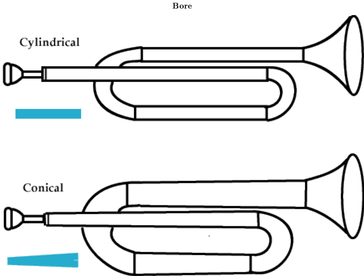
Figure 2.2: Bore affects the timbre of the instrument. In general, instruments with a cylindrical bore have a more direct sound with less complex harmonics. Instruments with a conical bore usually have a mellower sound with more complex harmonics.
