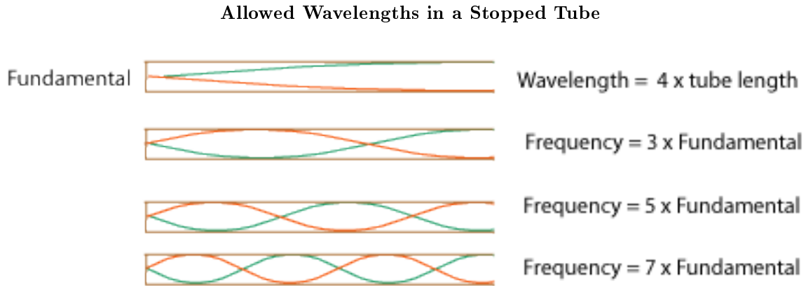
Figure 1.11: Again, these are the lowest (lowest pitch and lowest frequency) four harmonics allowed. Any wave with a displacement node at the closed end and antinode at the open end is allowed. Note that this means only the odd-numbered harmonics "fit".
