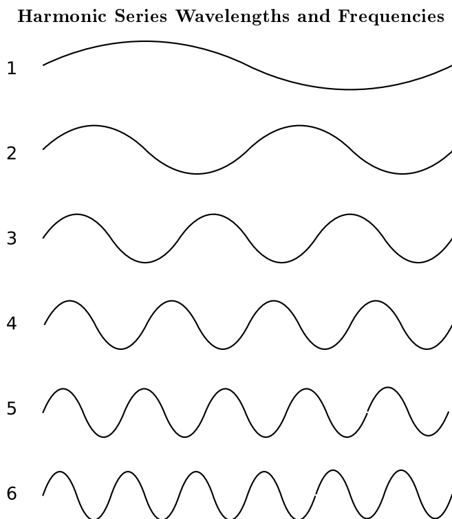
Figure 1.17: The second harmonic has half the wavelength and twice the frequency of the first. The third harmonic has a third the wavelength and three times the frequency of the first. The fourth harmonic has a quarter the wavelength and four times the frequency of the first, and so on. Notice that the fourth harmonic is also twice the frequency of the second harmonic, and the sixth harmonic is also twice the frequency of the third harmonic.
