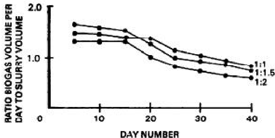
FIG. 3-9 RATIO OF VOLUME OF GAS PER DAY TO VOLUME OF DIGESTER SLURRY.
