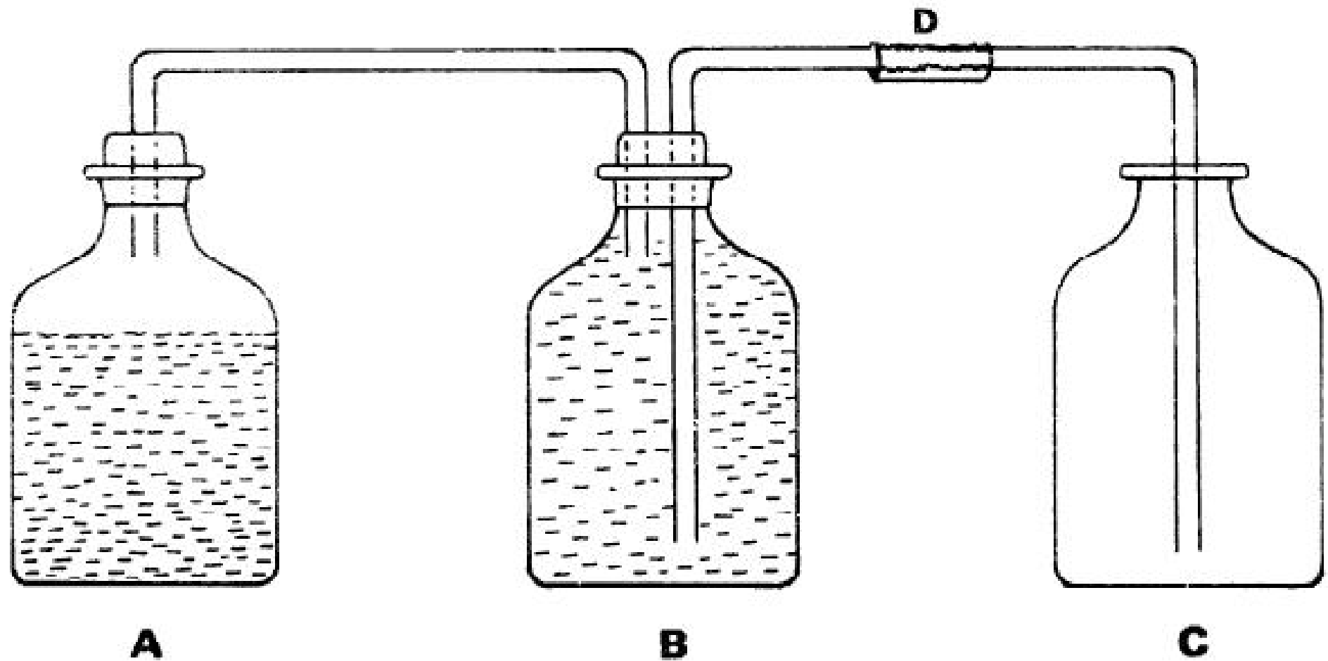
Fig. 3-1: Laboratory set-up for study of biological production of methane
