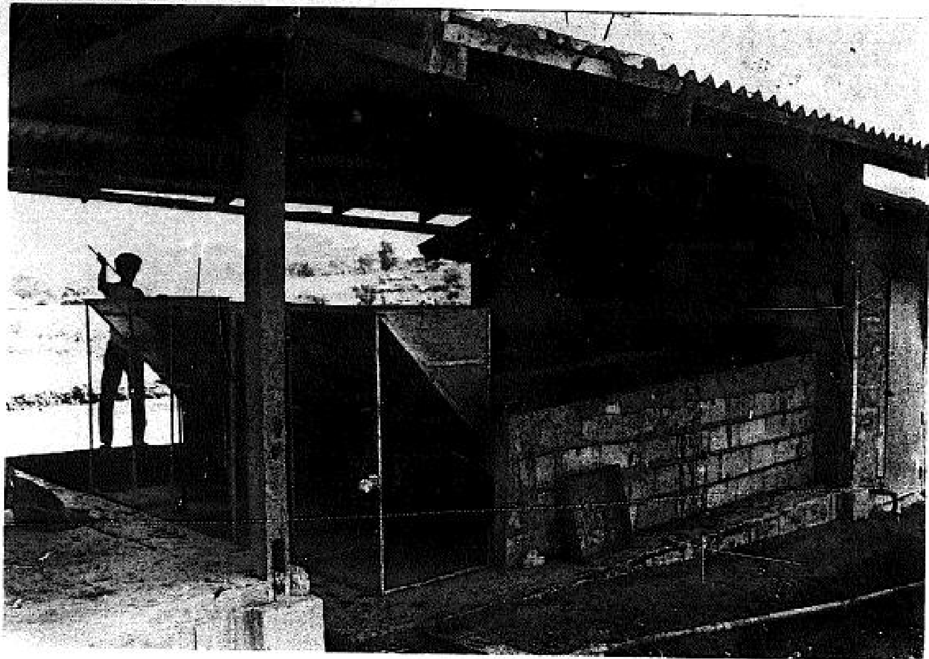
Illustration 4-9: Rice hull firing chamber
