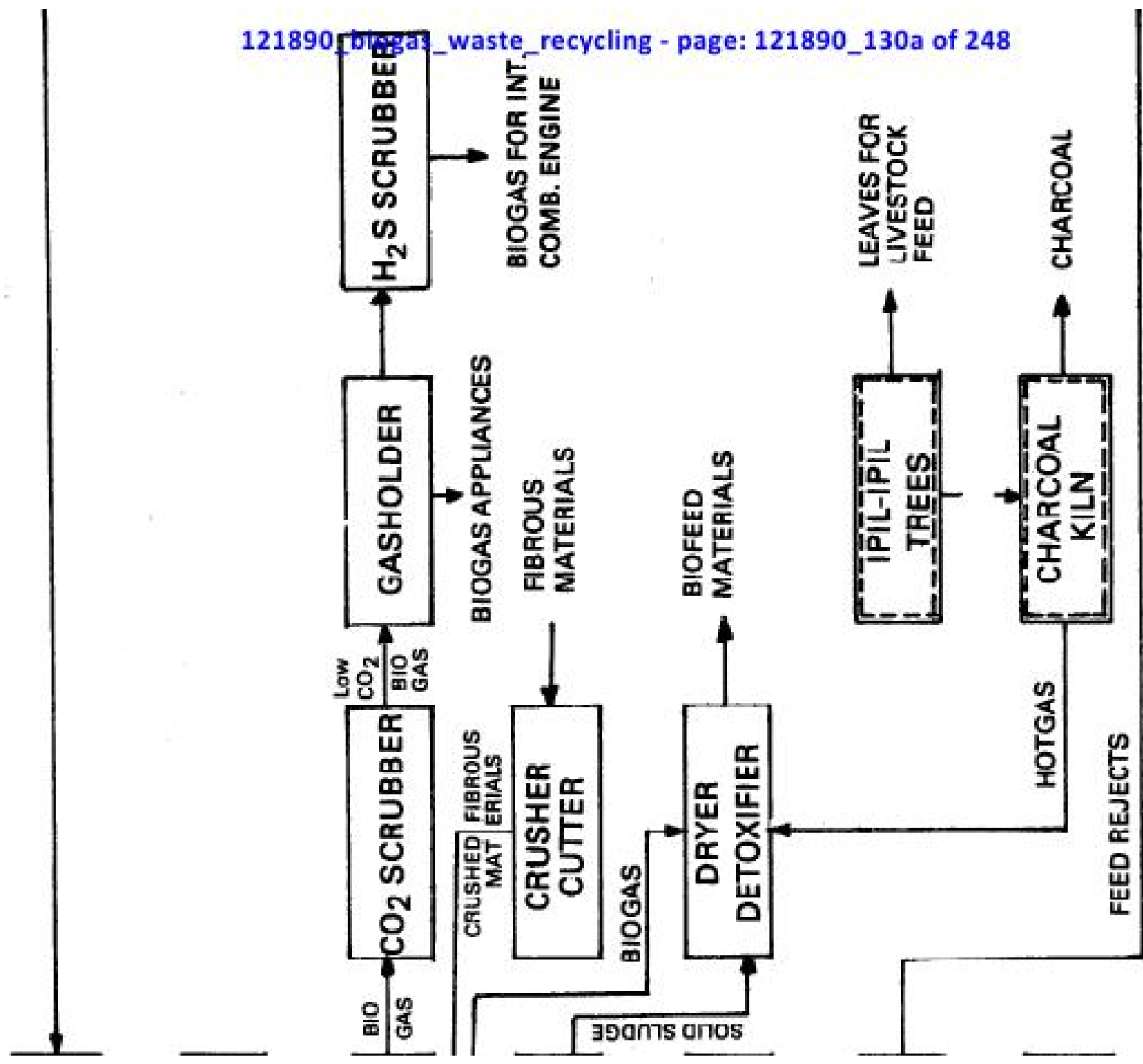
BIOGAS WORKS FLOWSHEET
