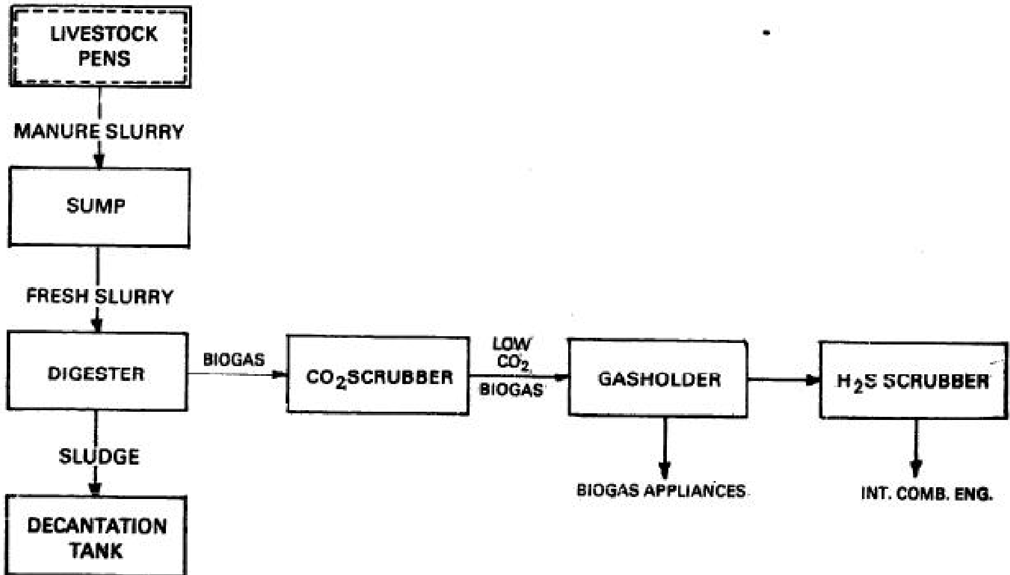
FIG. 6-2 SPLIT CONTINUOUS-FED BIOGAS PLANT
