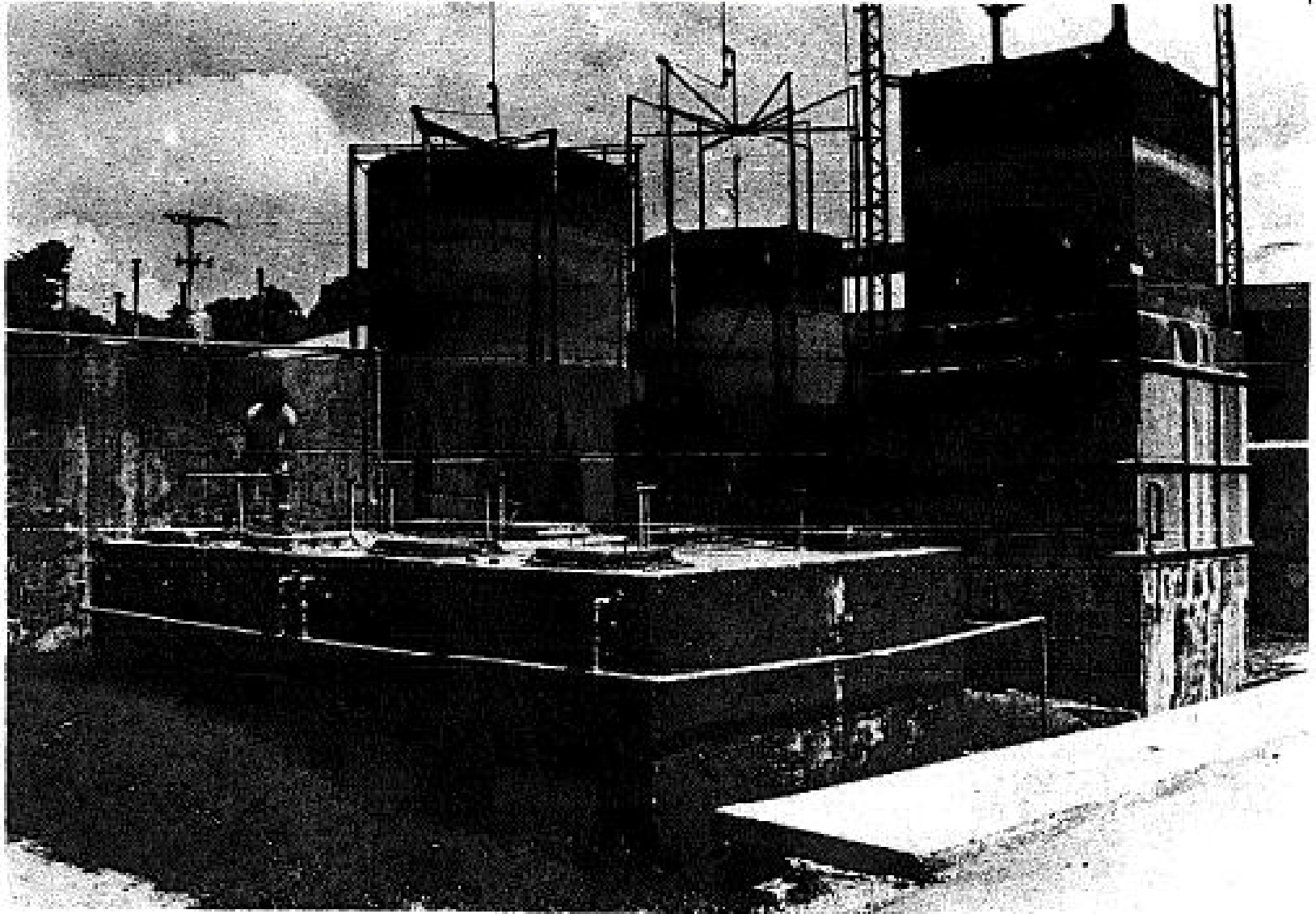
Illustration 1-5: Pilot plant batch-fed digesters
