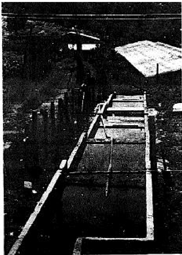
Illustration 2-5: Sludge conditioning canals with overflow dams.
