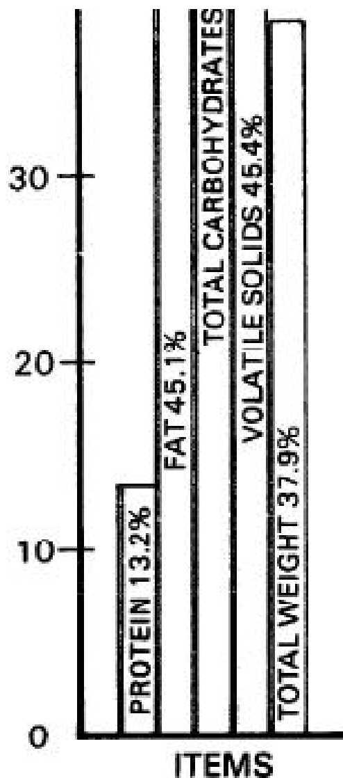
FIG. 5-3 PERCENT REDUCTION IN WEIGHT OF EACH ITEM 0 TO 50 DAYS
