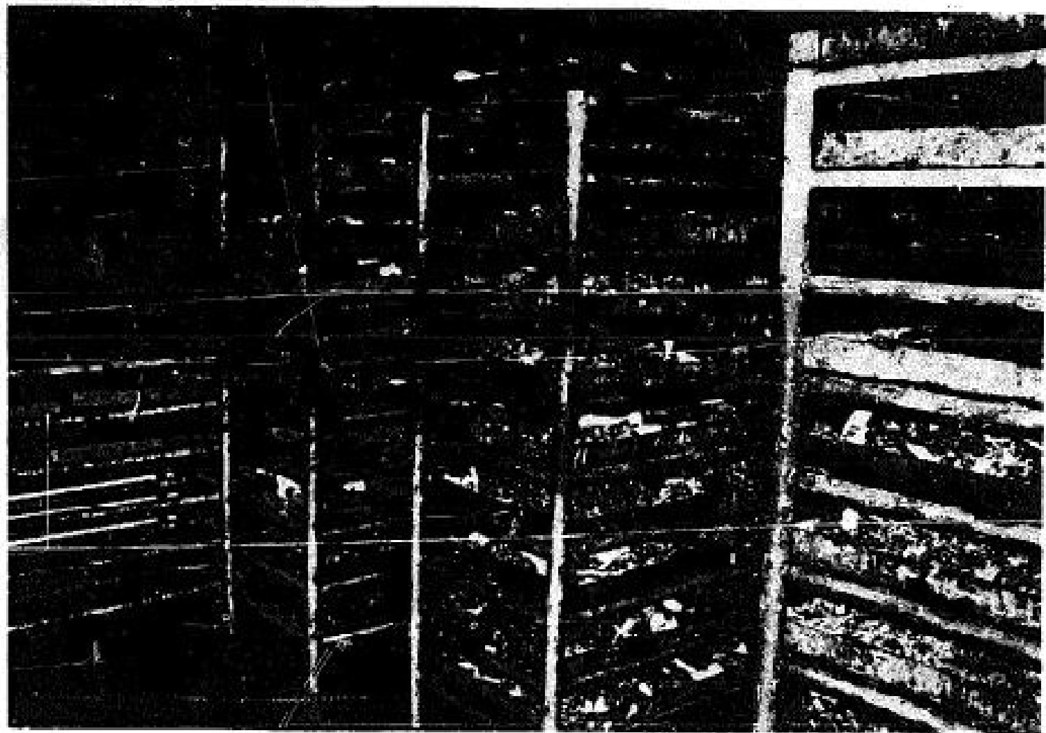
Illustration 3-3: Biogas-heated drying room in rendering plant.
