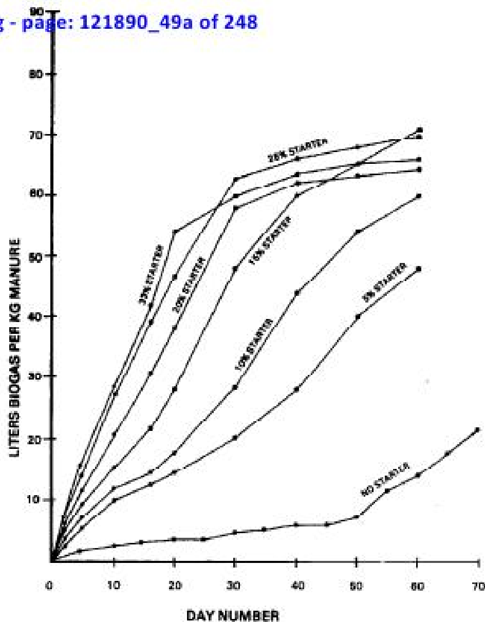
FIG. 3-6 GAS PRODUCTION CURVES FOR VARYING STARTER PERCENTAGE
