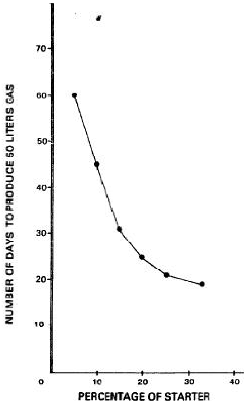
FIG. 3-7 RELATION OF PERCENTAGE OF STARTER AND NUMBER OF DAYS TO PRODUCE 50 LITERS BIOGAS
