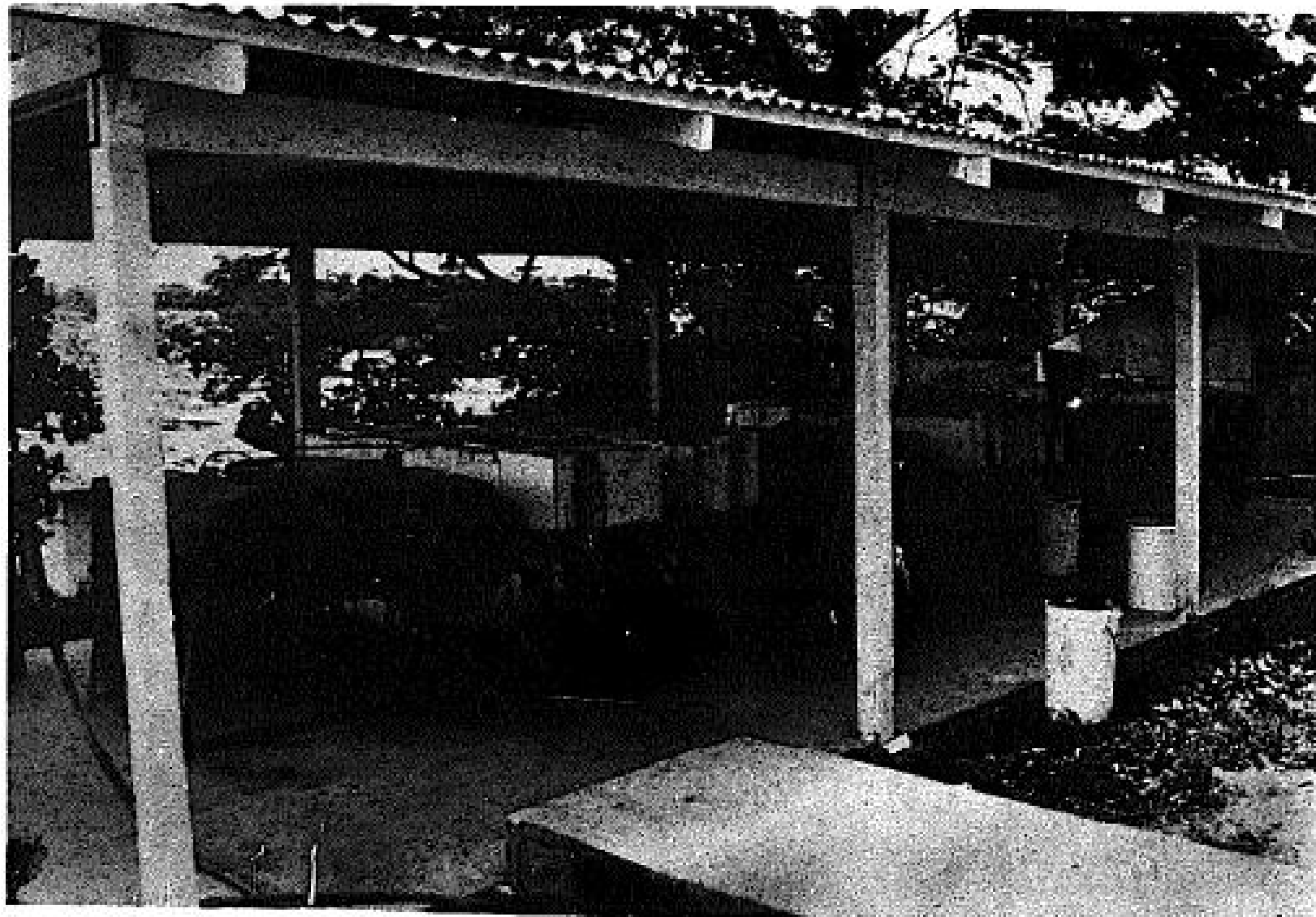
Illustration 1-6: Pilot plant continuous-fed digesters
