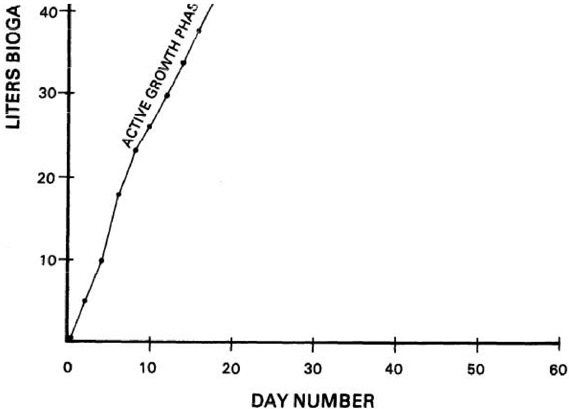
FIG. 3-2. TYPICAL BIOGAS PRODUCTION CURVE
