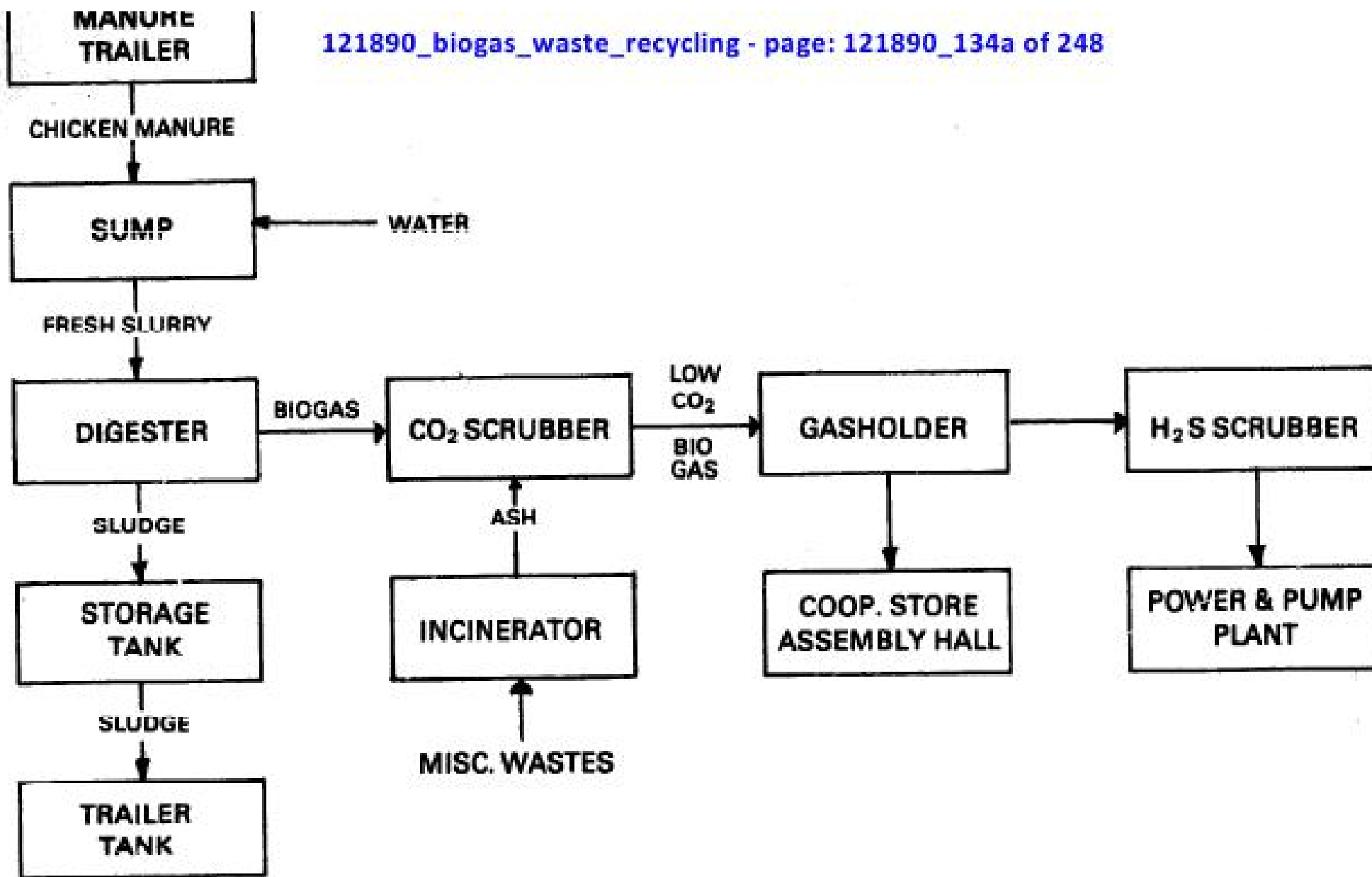
FIG. 9-9 COOPERATIVE BIOGAS WORKS FLOWSHEET
