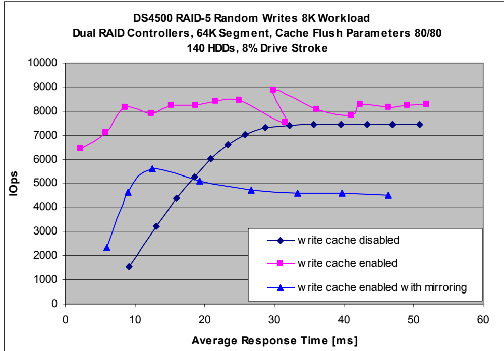
Chart 5. DS4500 RAID-5 Random Writes 8K Workload
