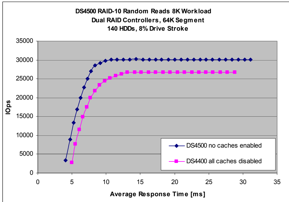
Chart 12. RAID-10 DS4500 8K Random Reads vs. DS4400 8K Random Reads
