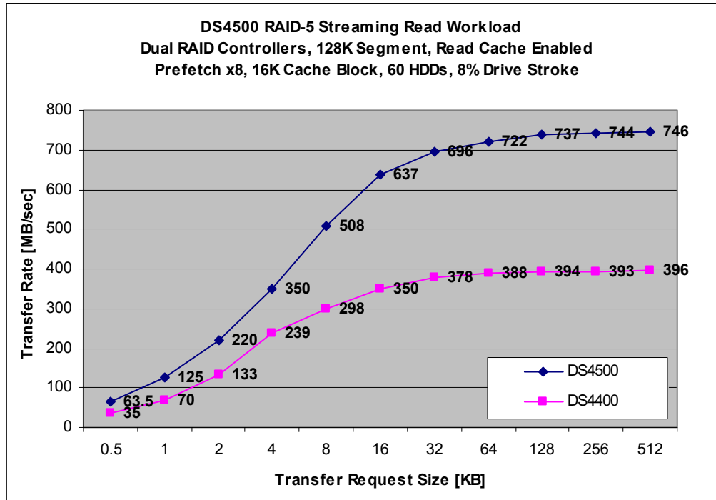
Chart 2. DS4500 RAID-5 Streaming Reads vs. DS4400 RAID-5 Streaming Reads
