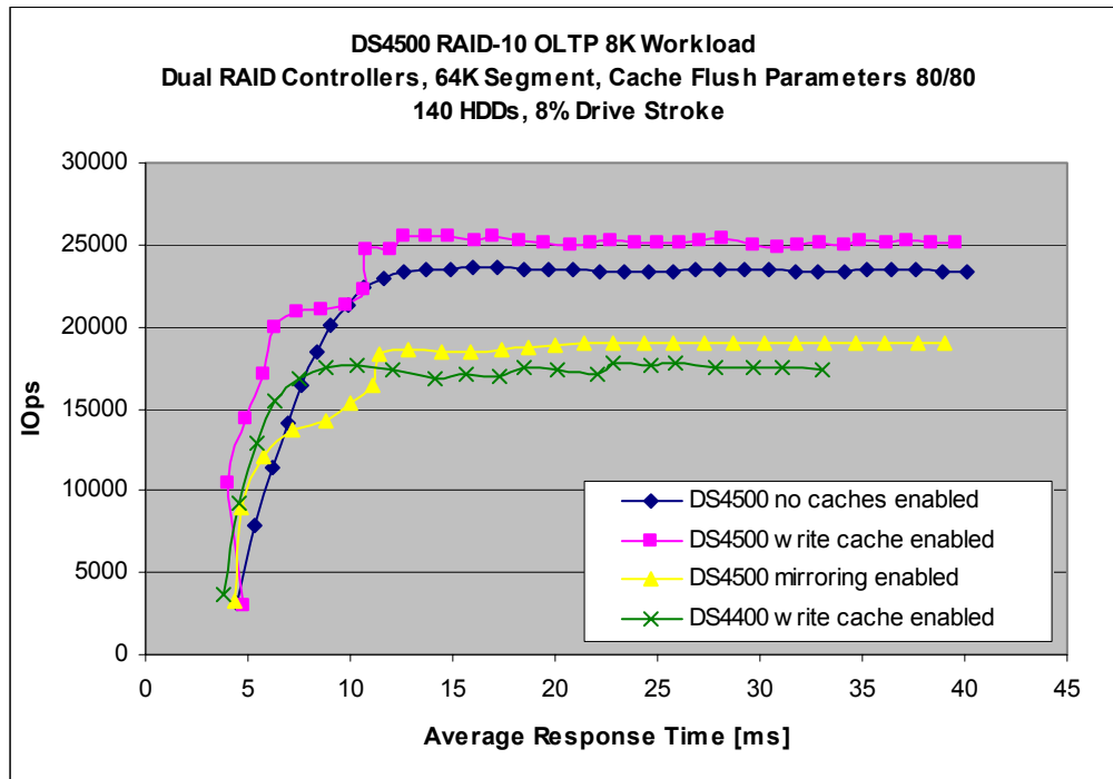
Chart 7. DS4500 RAID-10 OLTP 8K vs. DS4400
