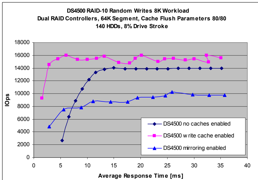
Chart 11. DS4500 RAID-10 Random Writes 8K Workload
