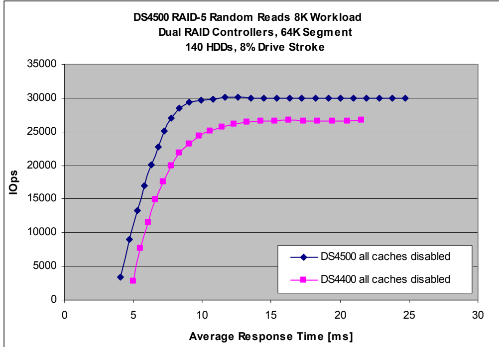
Chart 6. RAID-5 DS4500 8K Random Reads vs. DS4400 8K Random Reads
