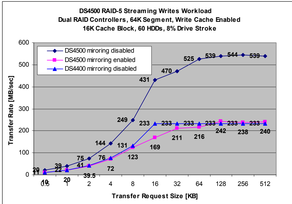
Chart 3. DS4500 RAID-5 Streaming Writes vs. DS4400 RAID-5 Streaming Writes
