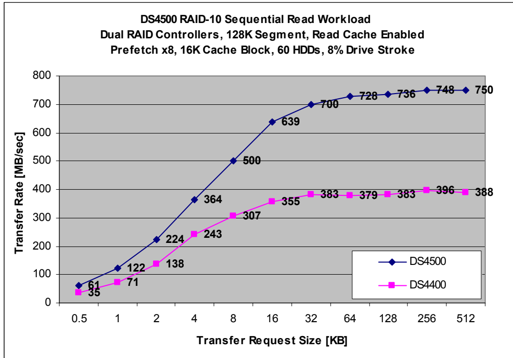
Chart 8. DS4500 RAID-10 Streaming Reads Transfer Rate
