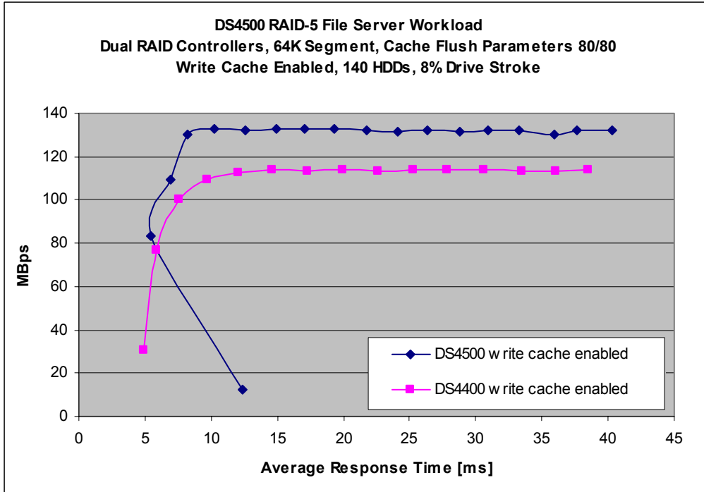
Chart 4. RAID-5 DS4500 File Server Workload vs. DS4400 File Server Workload
