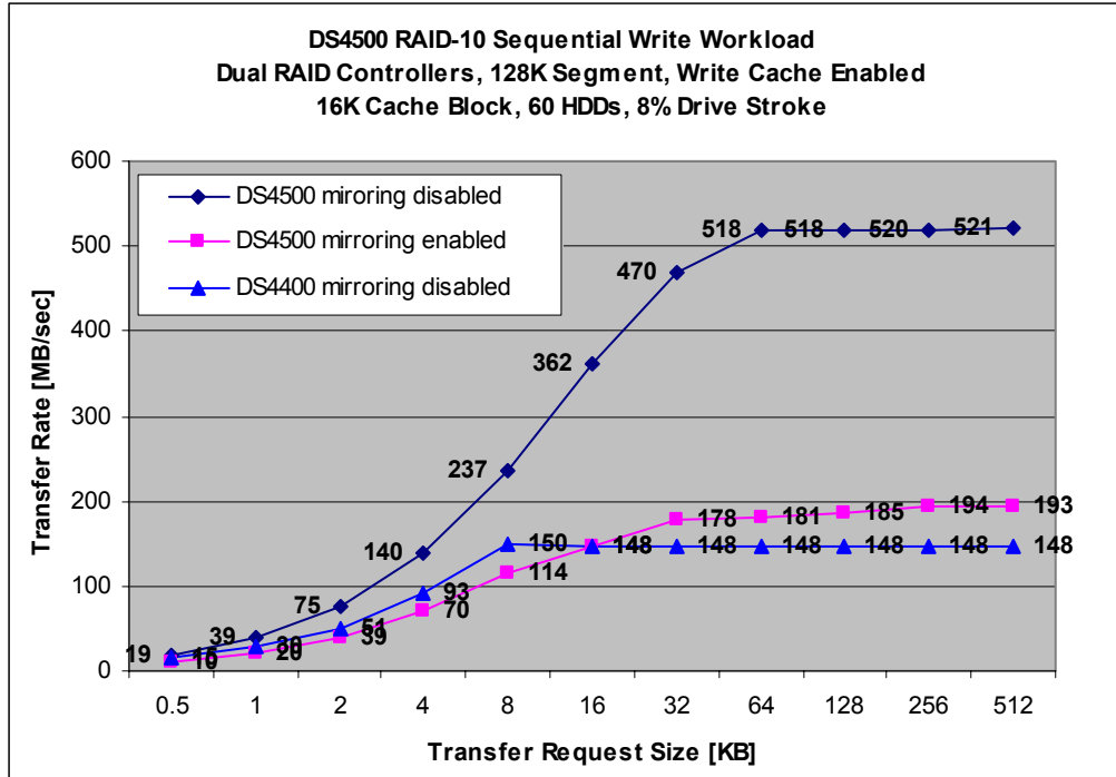
Chart 9. DS4500 RAID-10 Streaming Writes Transfer Rate
