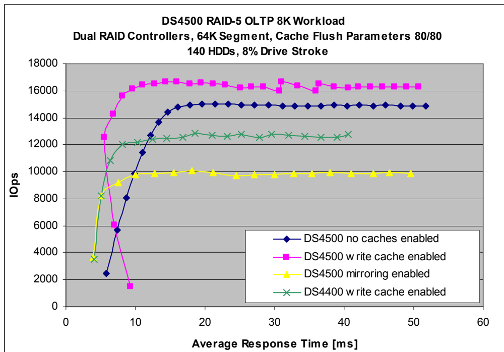
Chart 1. DS4500 RAID-5 OLTP 8K vs. DS4400 RAID-5 OLTP 8K
