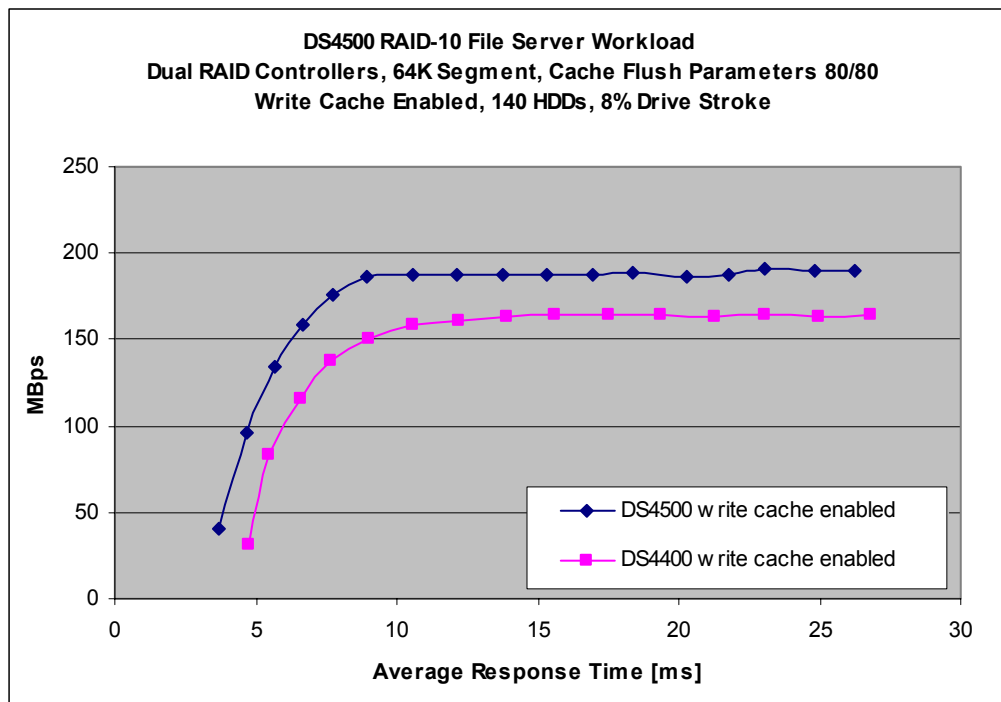
Chart 10. DS4500 RAID-10 File Server Workload vs. DS4400 File Server Workload
