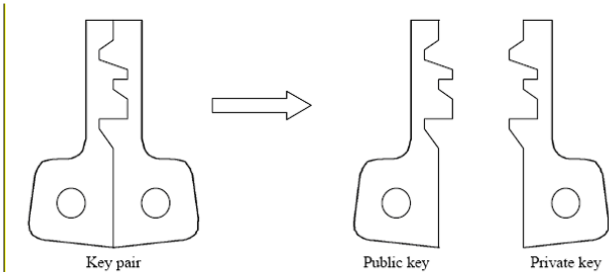
Figure 5-90: Asymmetric keys
