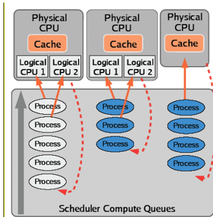
Figure 5-14: Hyperthreaded scheduling
