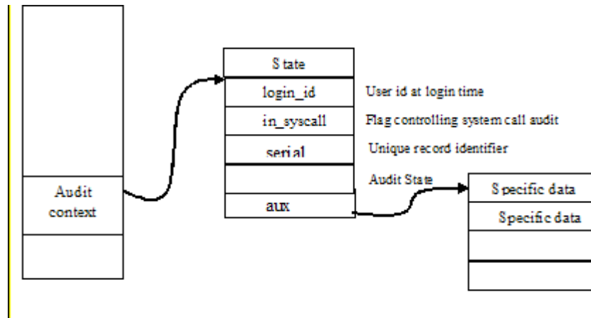
Figure 5-73: Task Structure
