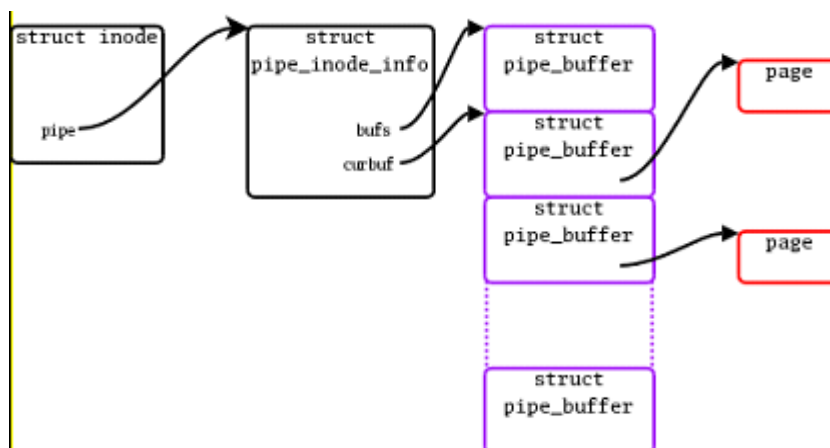
Figure 5-15: Pipes Implementation
