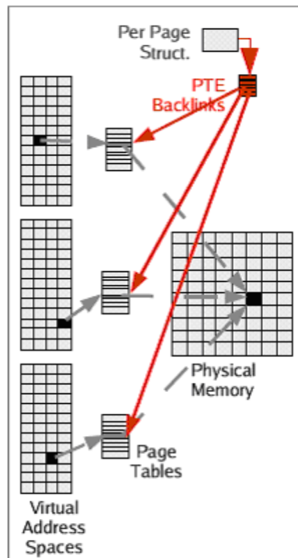
Figure 5-67: Rmap VM
