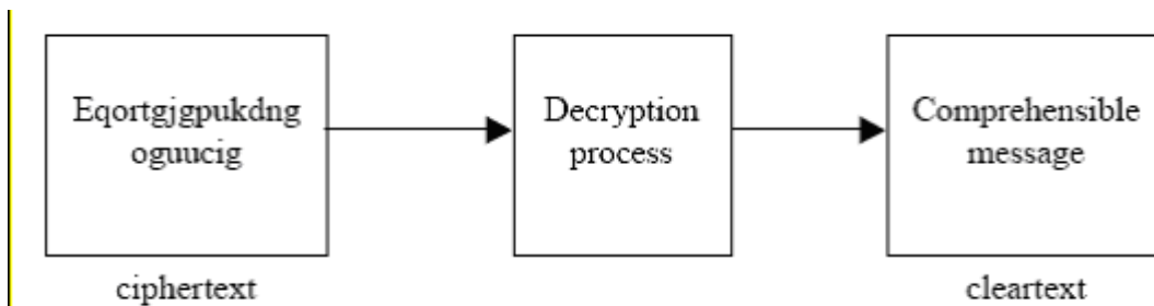
Figure 5-88: Decryption
