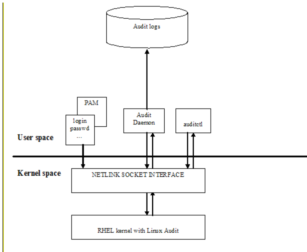
Figure 5-71: Audit framework components
