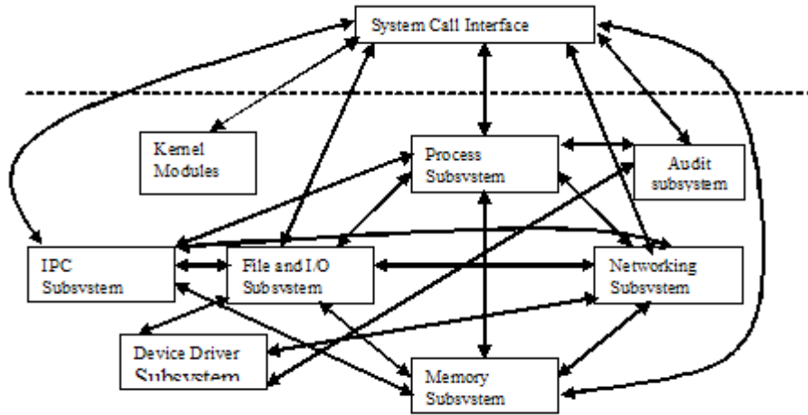
Figure 4-5: Logical kernel subsystems and their interactions
