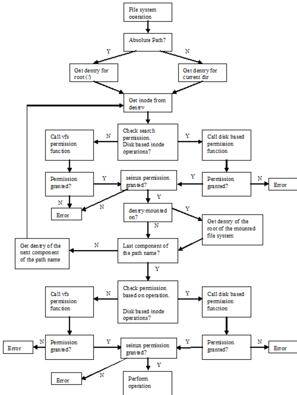
Figure 5-5: VFS pathname translation and access control checks
