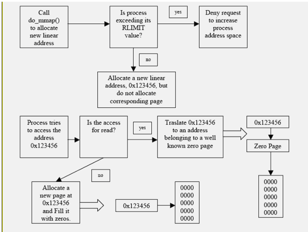
Figure 5-70: Object reuse handling while allocating new linear address
