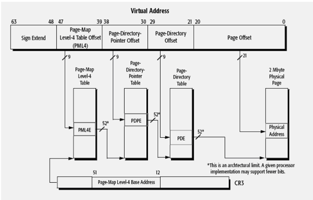
Figure 5-64: 2 MB page translation, virtual to physical address translation
