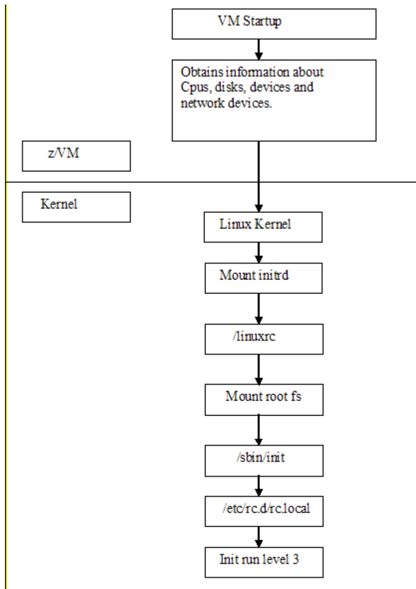
Figure 5-84: System z Red Hat Enterprise Linux boot sequence
