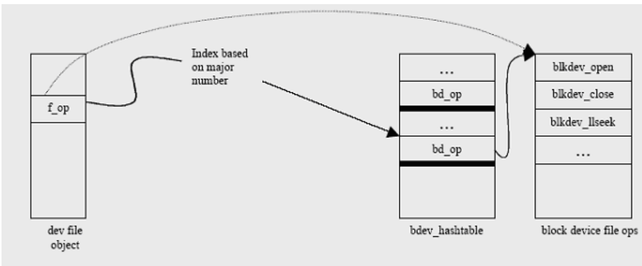
Figure 5-80: Setup of f_op for block device specific file operations
