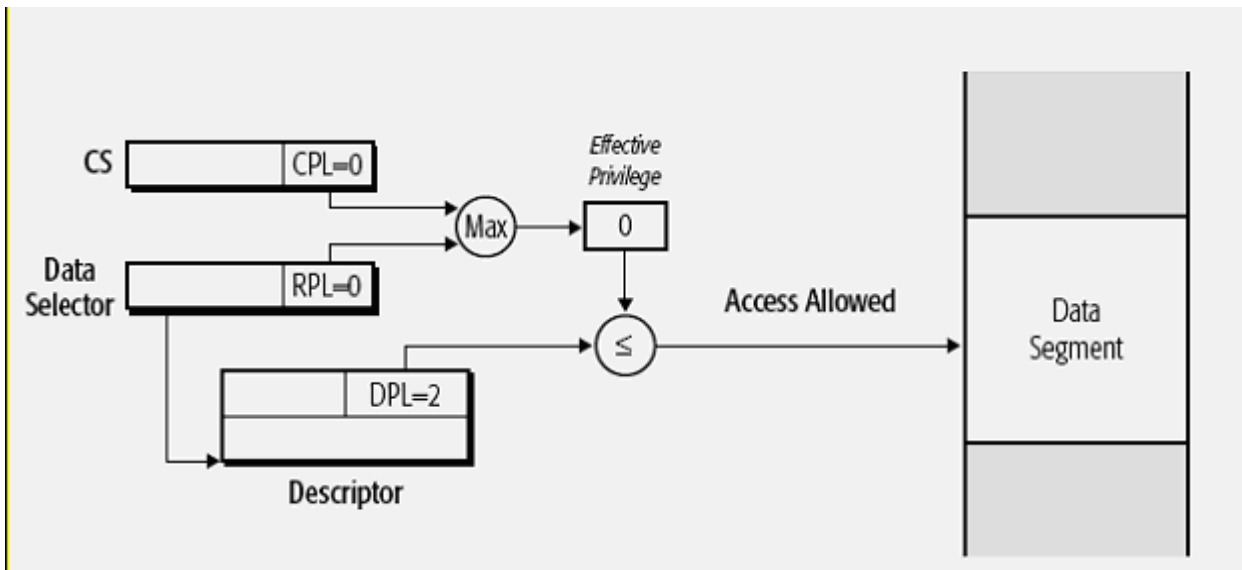
Figure 5-61: Data access privilege checks
