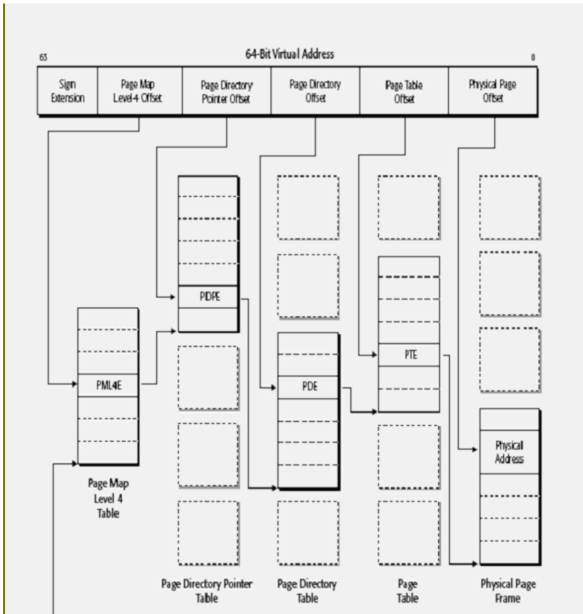
Figure 5-63: 4 KB page translation, virtual to physical address translation
