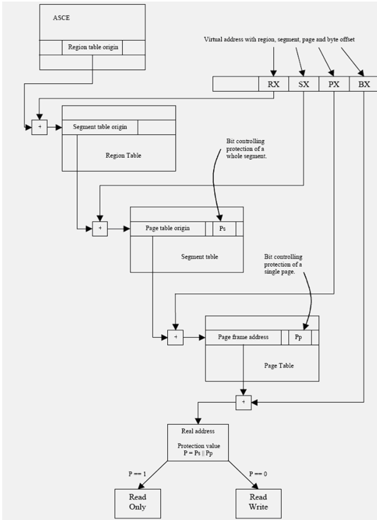
Figure 5-57: 64-bit Dynamic Address Translation with page table protection
