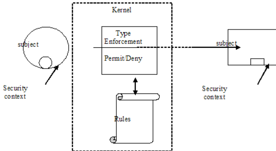
Figure 4-3: SELinux Type Enforcement
