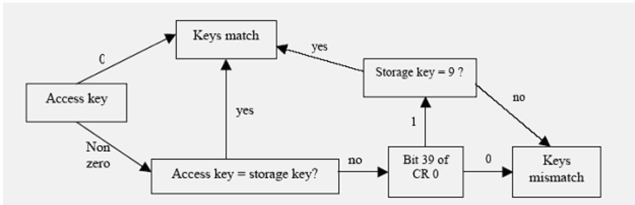
Figure 5-58: Key match logic for key-controlled protection
