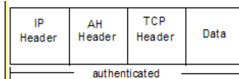
An IP Packet with transport mode AH
