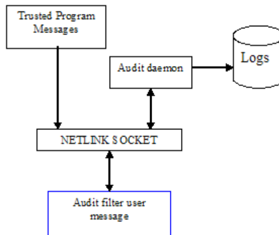
Figure 5-77: User Space Record Generation
