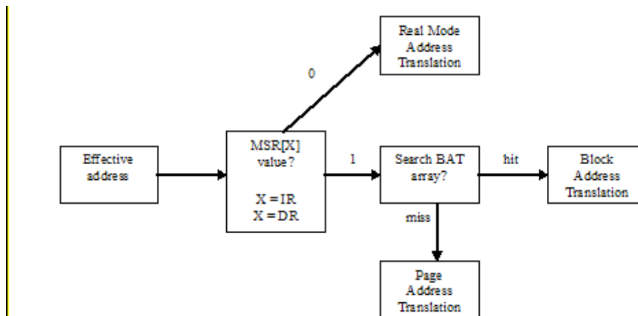
Figure 5-48: Address translation method selection
