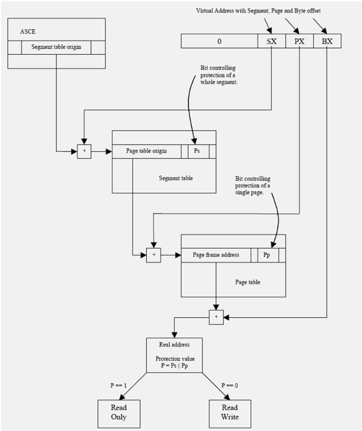
Figure 5-56: 31-bit Dynamic Address Translation with page table protection
