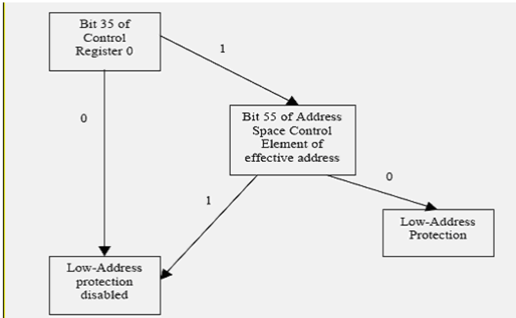
Figure 5-55: Low-address protection on effective address
