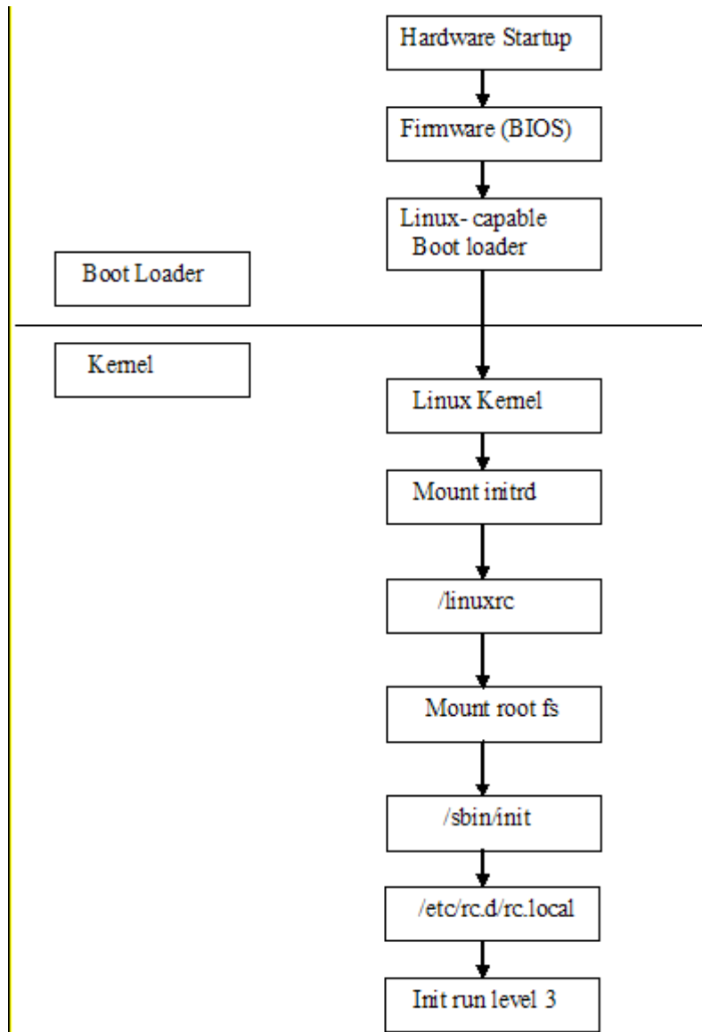
Figure 5-85: eServer 326 Red Hat Enterprise Linux boot sequence
