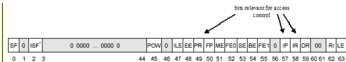
Figure 5-44: Machine state register
