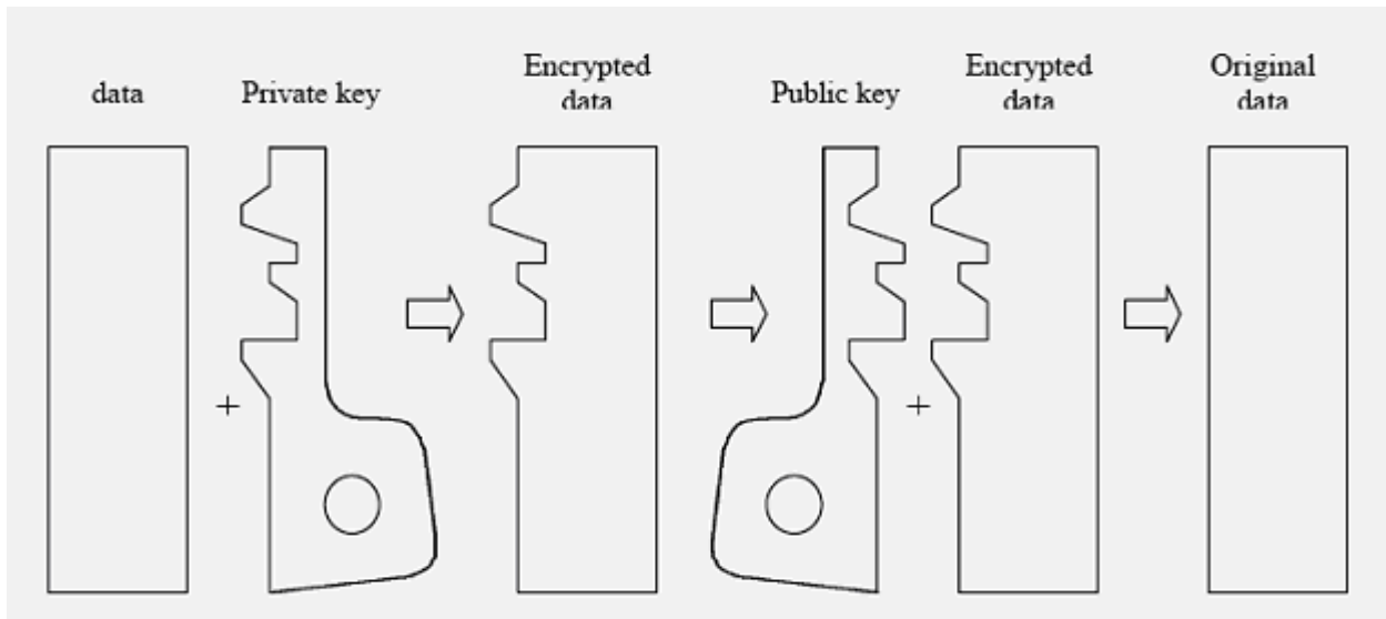
Figure 5-91: Encryption with private key provides authentication
