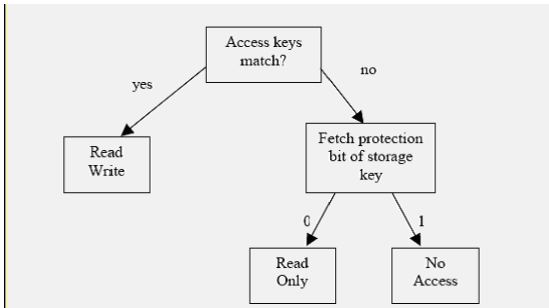
Figure 5-59: Fetch protection override for key-controlled
