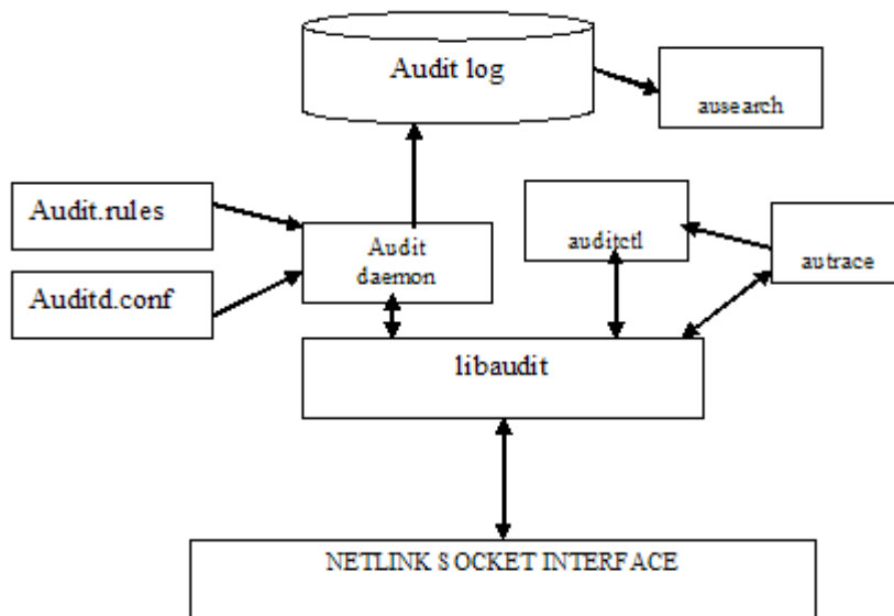
Figure 5-74: Audit User Space Components
