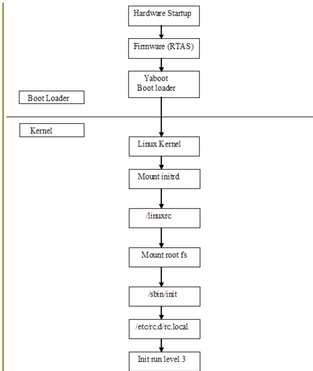
Figure 5-82: System p Red Hat Enterprise Linux boot sequence
