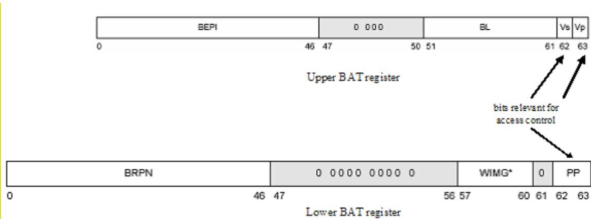
Figure 5-47: Block Address Translation entry
