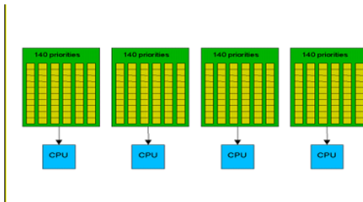
Figure 5-13: O(1) scheduling
