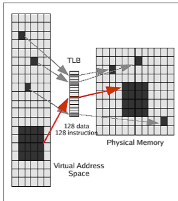
Figure 5-68: TLB Operation
