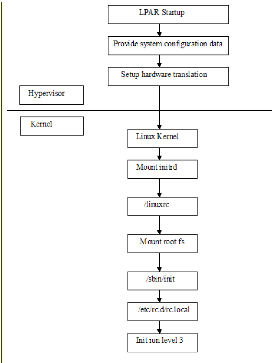
Figure 5-83: System p LPAR Red Hat Enterprise Linux boot sequence
