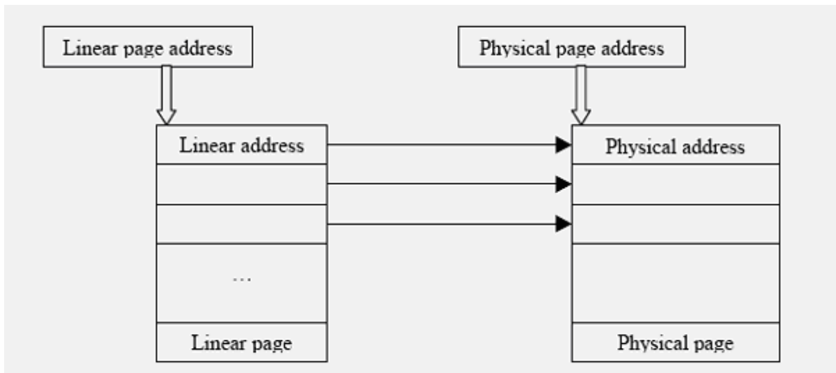
Figure 5-62: Contiguous linear addresses map to contiguous physical addresses
