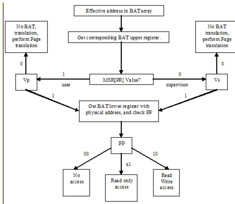
Figure 5-49: Block Address Translation access control
