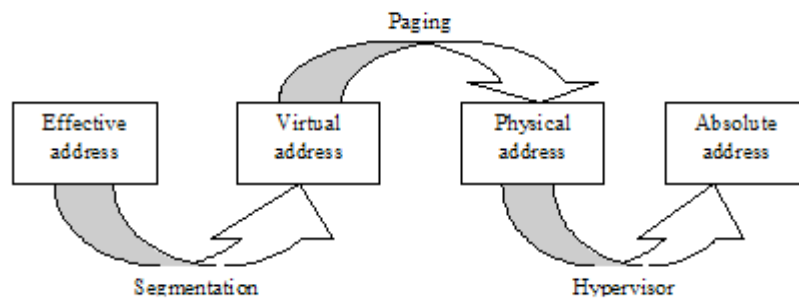
Figure 5-38: Address translation in LPAR
