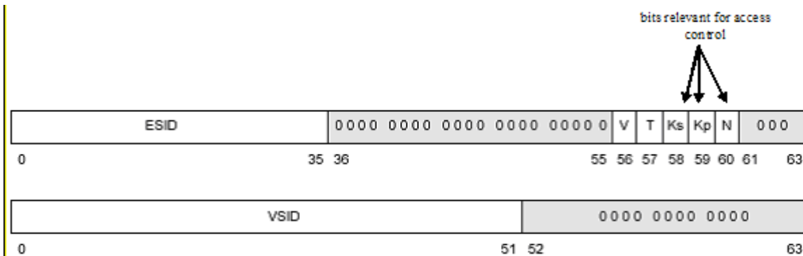
Figure 5-46: Segment Table Entry
