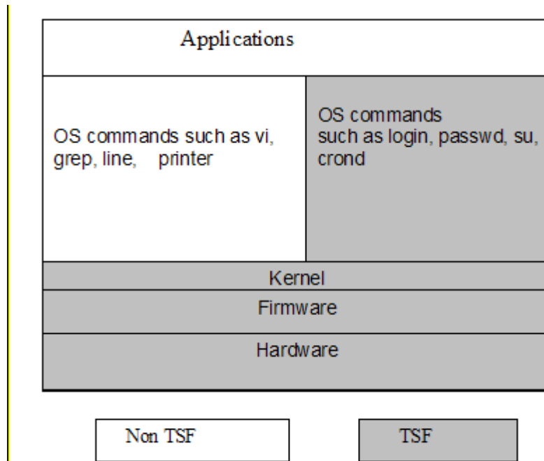
Figure 4-4: TSF and non-TSF software
