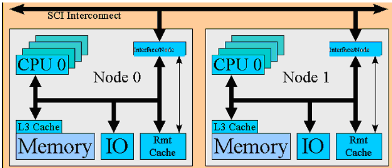
Figure 5-66: NUMA Design
