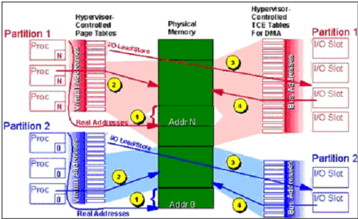
Figure 5-40: DMA addressing
