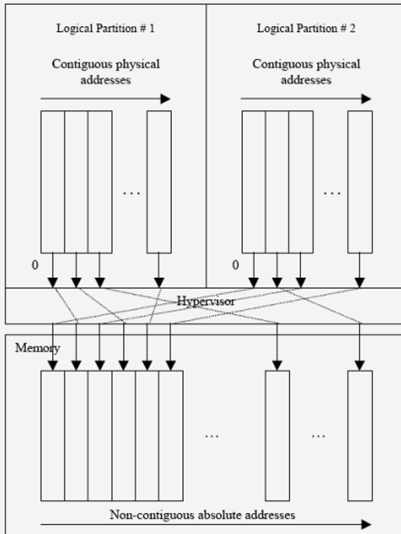
Figure 5-39: Absolute addresses
