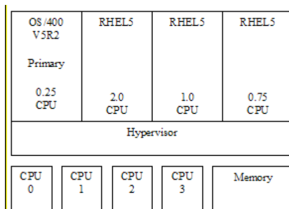
Figure 5-34: Logical partitions
