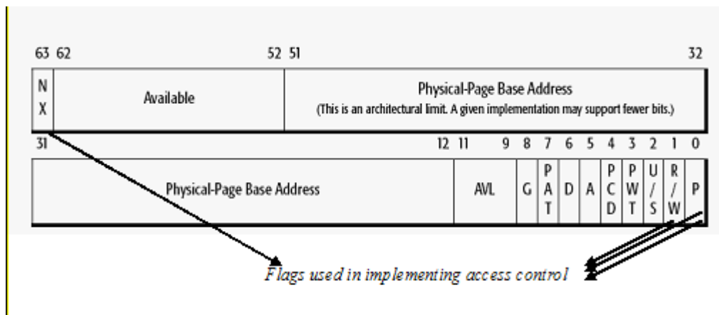
Figure 5-65: Page map level four entry
