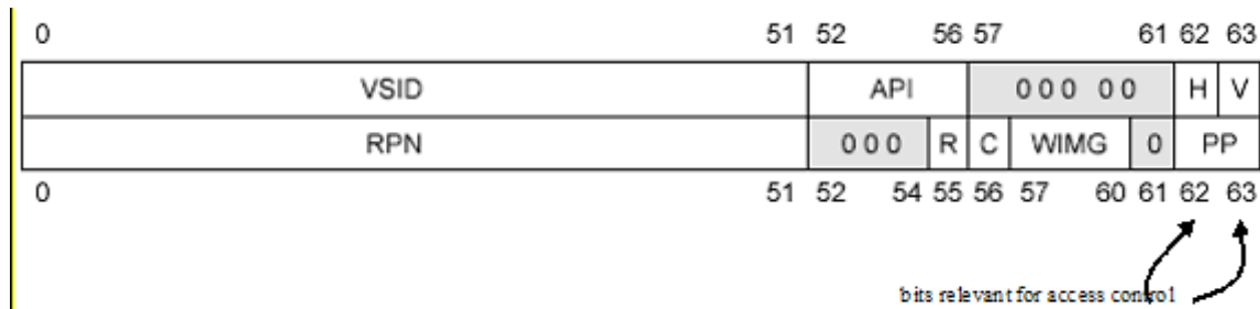
Figure 5-45: Page table entry
