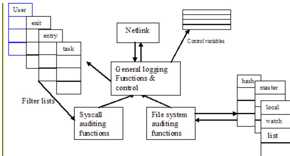
Figure 5-72: Audit Kernel Components
