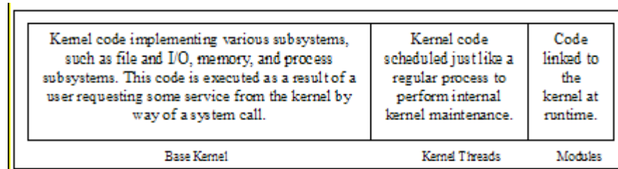
Figure 4-6: Kernel execution components
