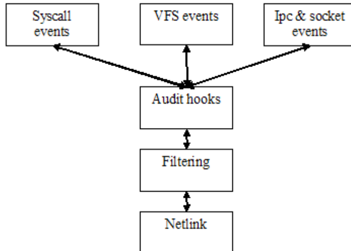
Figure 5-75: Audit Record Generation
