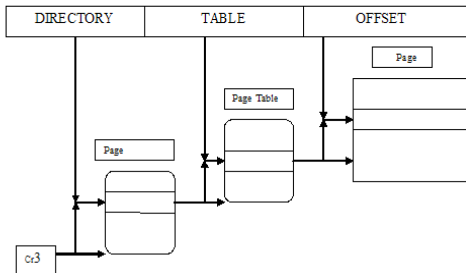
Figure 5-30: Regular paging
