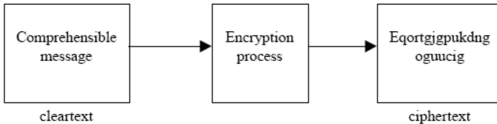
Figure 5-87: Encryption
