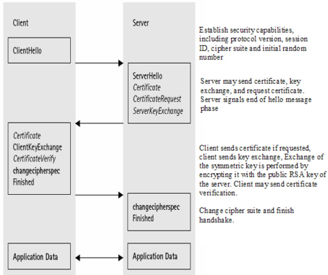
Figure 5-93: Handshake protocol (optional or content-dependent handshake messages are in italic type)
