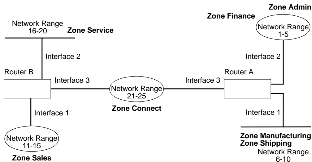
Figure 32-2. Example of Network Filtering.
