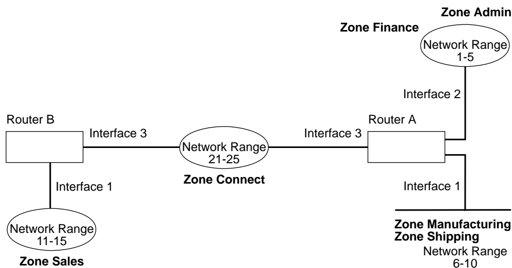
Figure 32-1. Example of Zone Filtering
