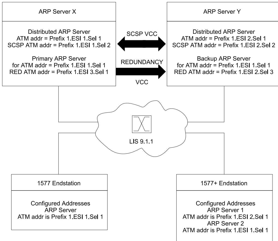
Figure 23-4. ARP Server Configuration with RFC 1577 and 1577+ Clients
