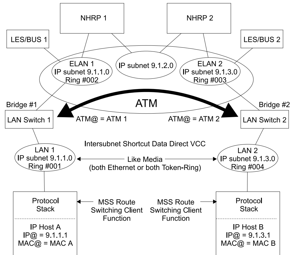
Figure 30-9. Route Switching Overview
