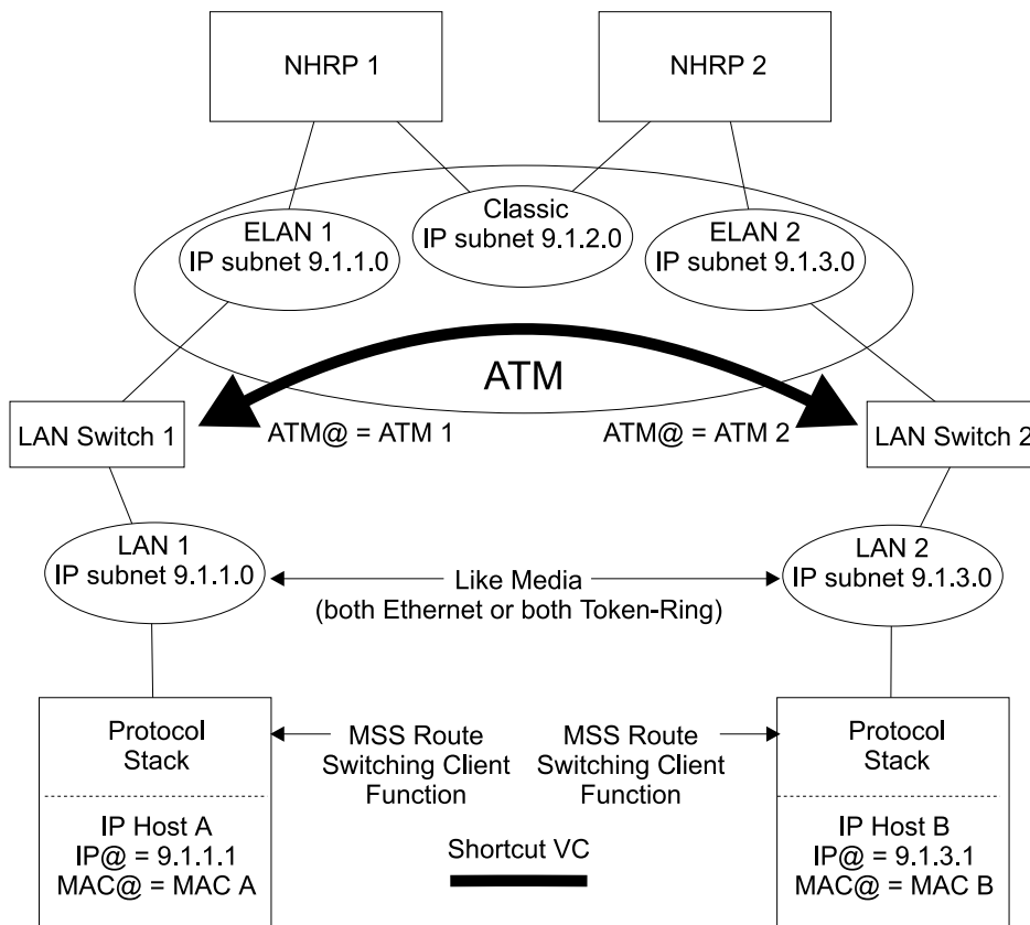
Figure 30-10. Route Switching in Both Directions
