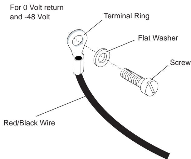
Figure 13. Connecting the Red/Black Wires
