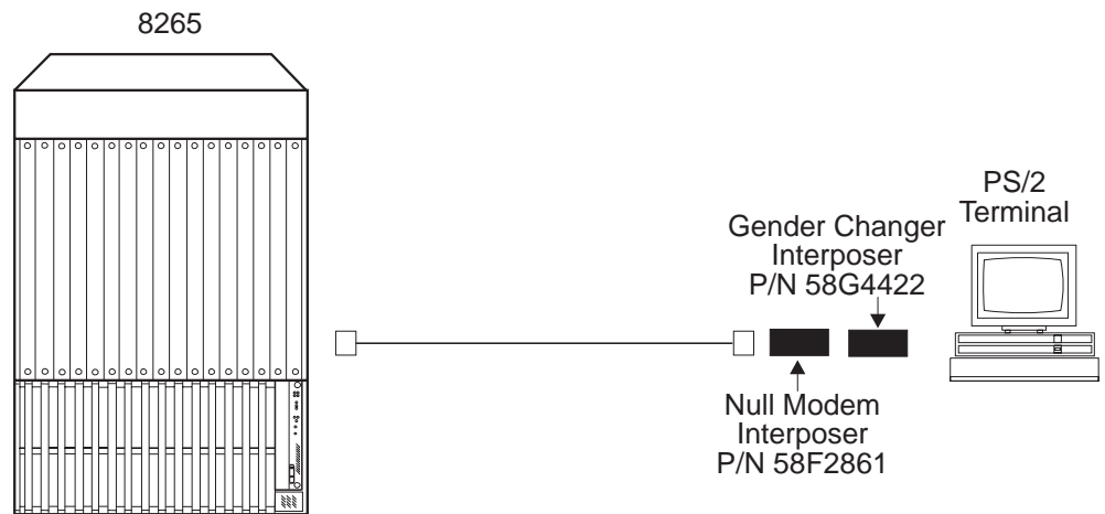
Figure 20. PC or PS/2 Cabling
