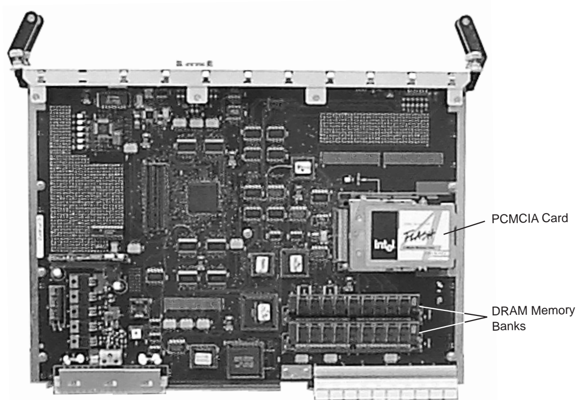
Figure 17. 8265 CPSW Module
