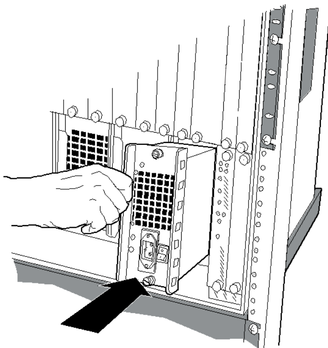
Figure 22. Replacing a Defective Load-Sharing Power Supply
