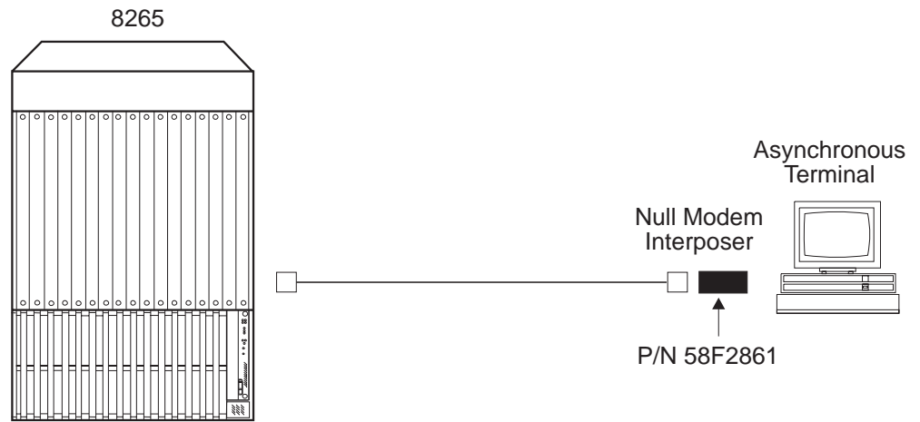
Figure 19. ASCII Terminal Cabling
