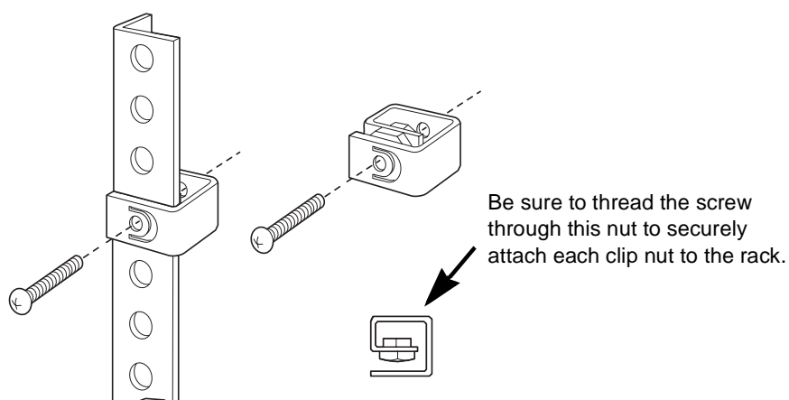
Figure 4. Installing a Clip Nut in the Rack
