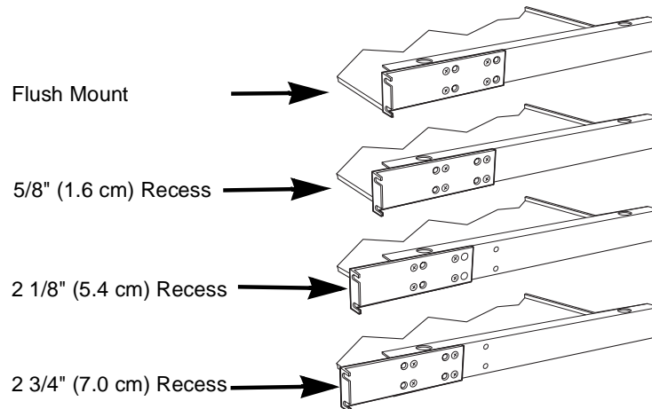
Figure 3. Cable Management Tray Rack Mount Positions
