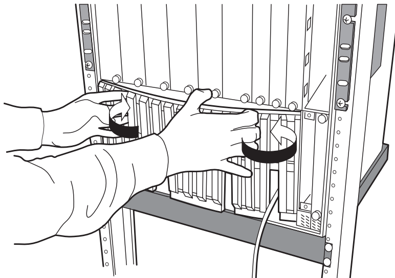
Figure 15. Installing the Power Supply Bay Grille
