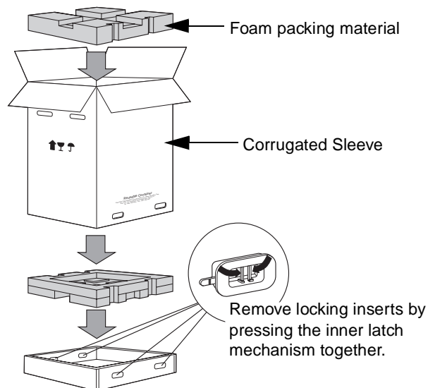
Figure 2. Unpacking the Switch Shipping Box
