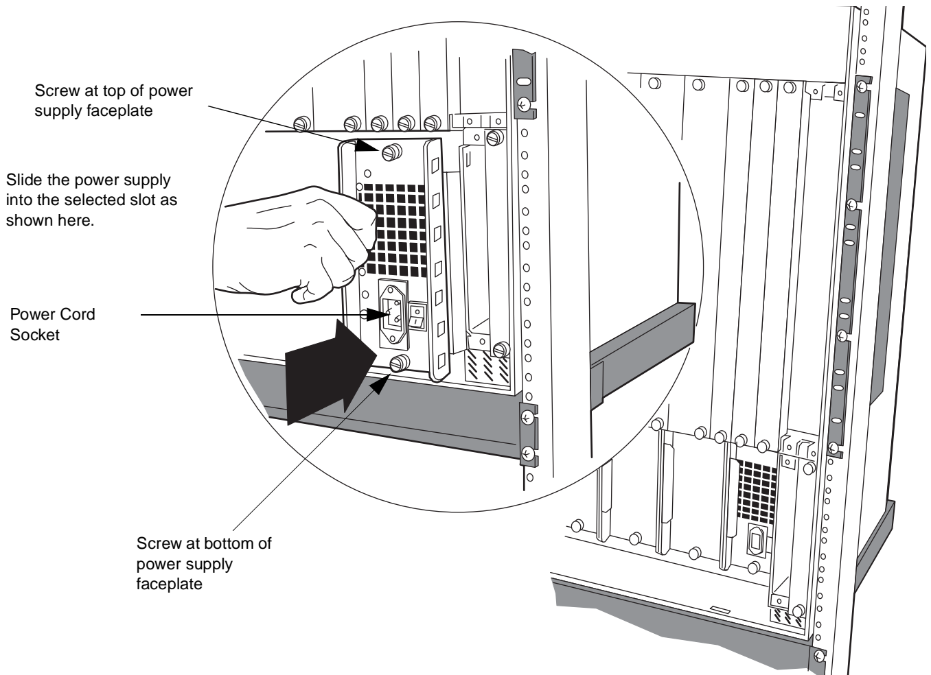
Figure 9. Installing a Load-Sharing Power Supply
