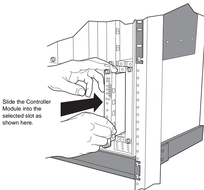
Figure 16. Installing a Controller Module
