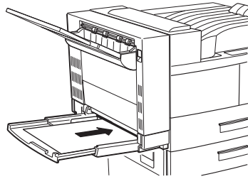
Auxiliary Tray, Face-up Output Bin Jams
