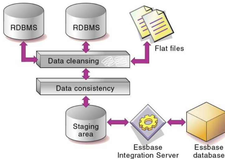
Figure 3: Data Warehouse with Staging Area
