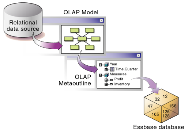
Figure 1: Workflow for Creating an Essbase Database from a Relational Data Source
